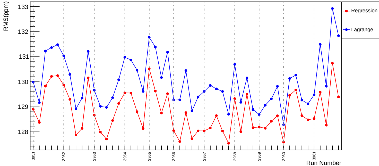
Slug35: Corrected RMS (ppm): asym_usr
