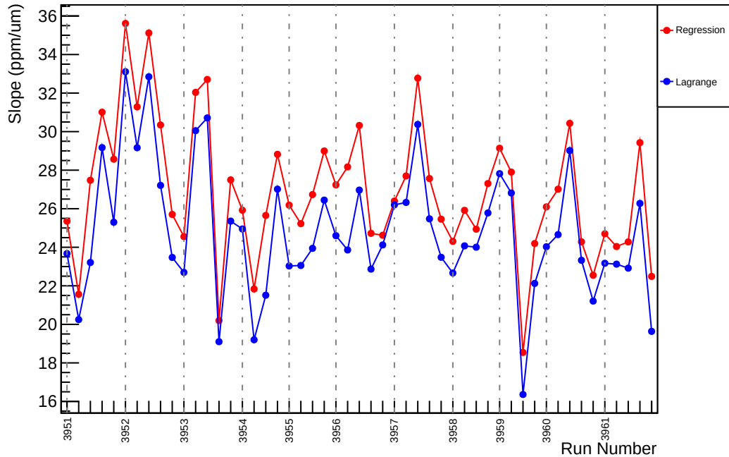
Slug35: Slope : usr_vs_evMon5 (ppm/um)
