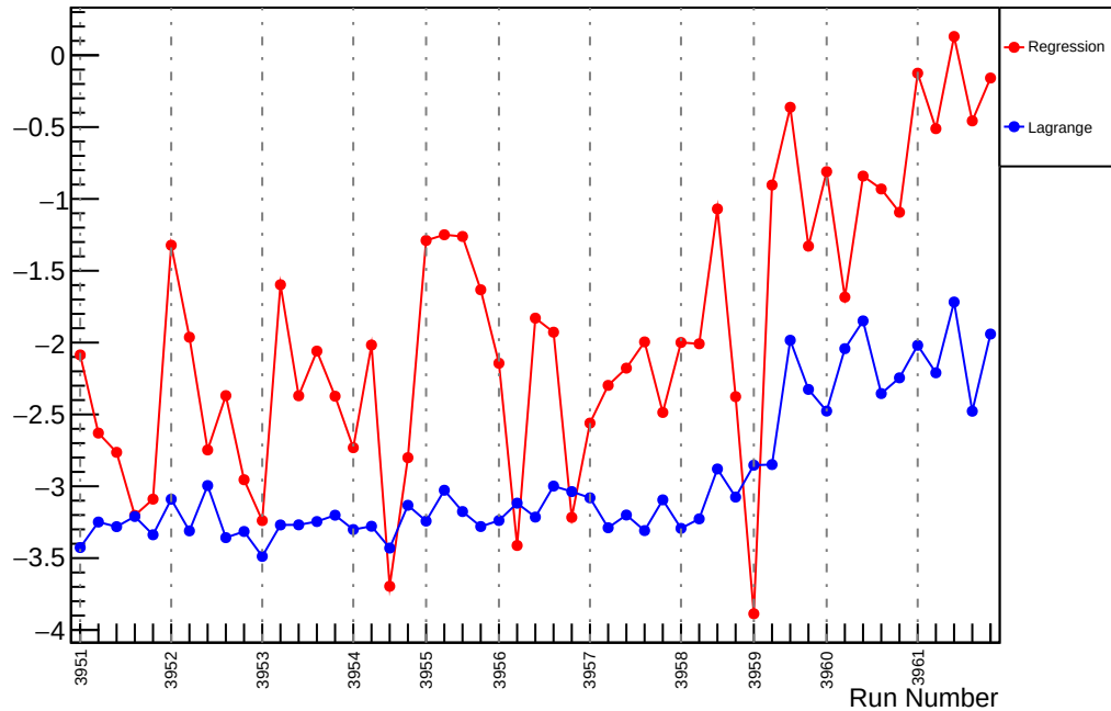
Slug35: Slope : usr_vs_evMon3 (ppm/um)
