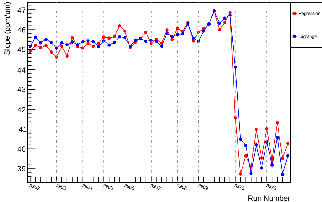
Slug36: Slope : usl_vs_evMon2 (ppm/um)
