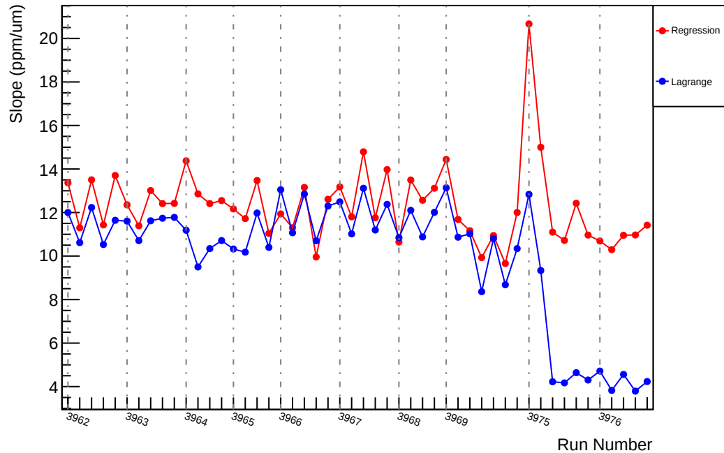
Slug36: Slope : usl_vs_evMon4 (ppm/um)
