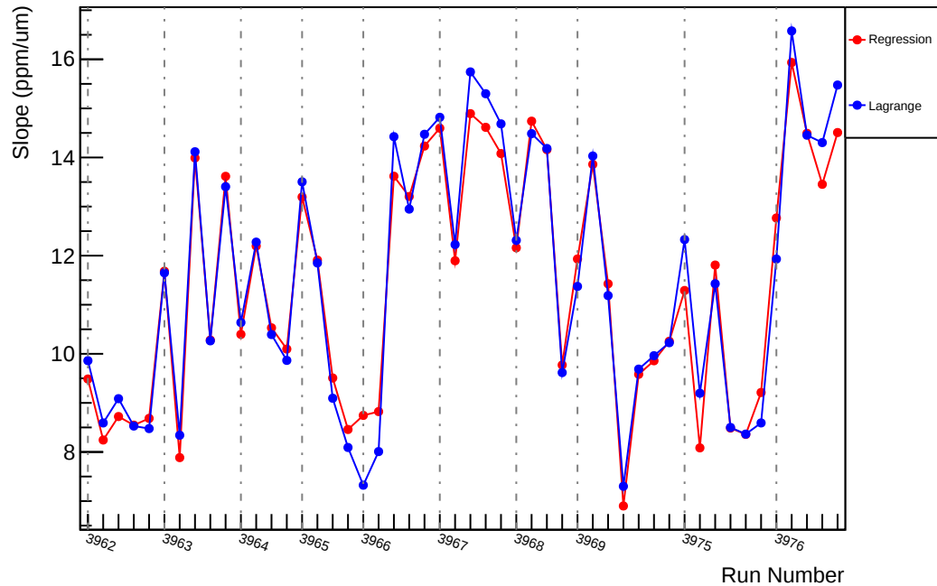
Slug36: Slope : usl_vs_evMon6 (ppm/um)
