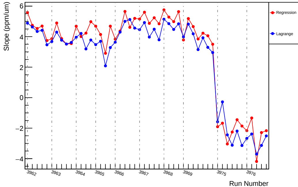
Slug36: Slope : usl_vs_evMon3 (ppm/um)
