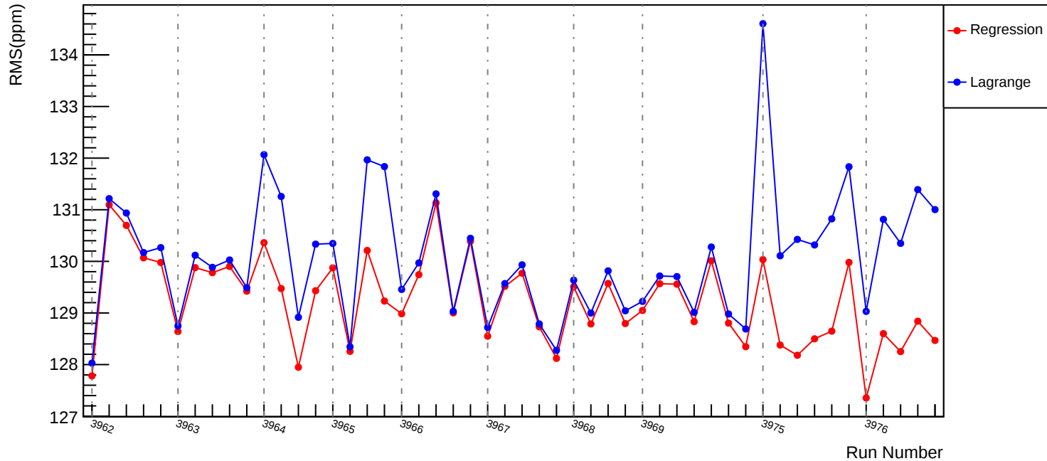
Slug36: Corrected RMS (ppm): asym_usl
