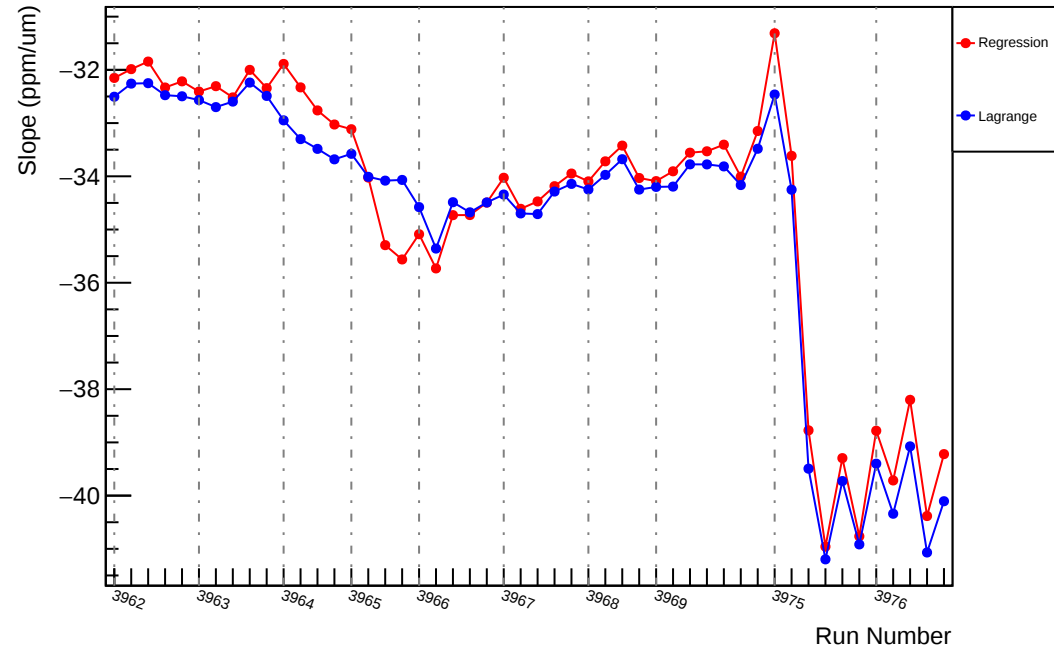
Slug36: Slope : usl_vs_evMon0 (ppm/um)
