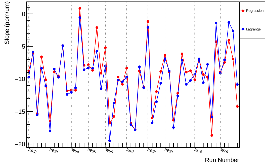
Slug36: Slope : usl_vs_evMon10 (ppm/um)
