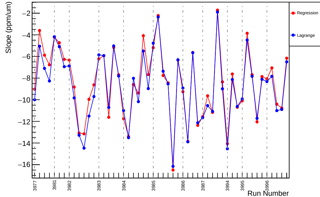
Slug37: Slope : us_dd_vs_evMon11 (ppm/um)
