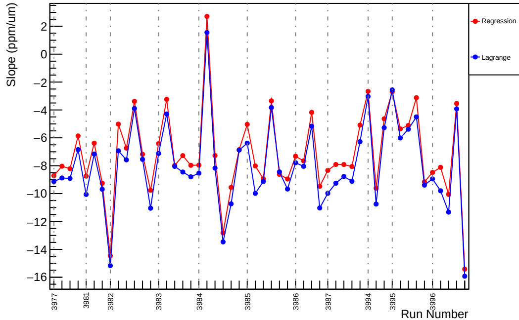
Slug37: Slope : us_dd_vs_evMon10 (ppm/um)
