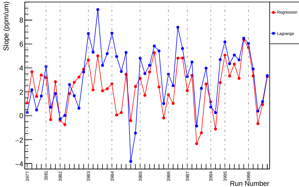
Slug37: Slope : us_dd_vs_evMon8 (ppm/um)
