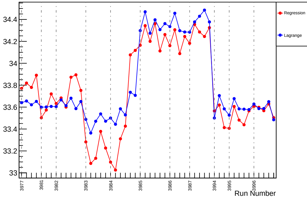
Slug37: Slope : us_dd_vs_evMon0 (ppm/um)
