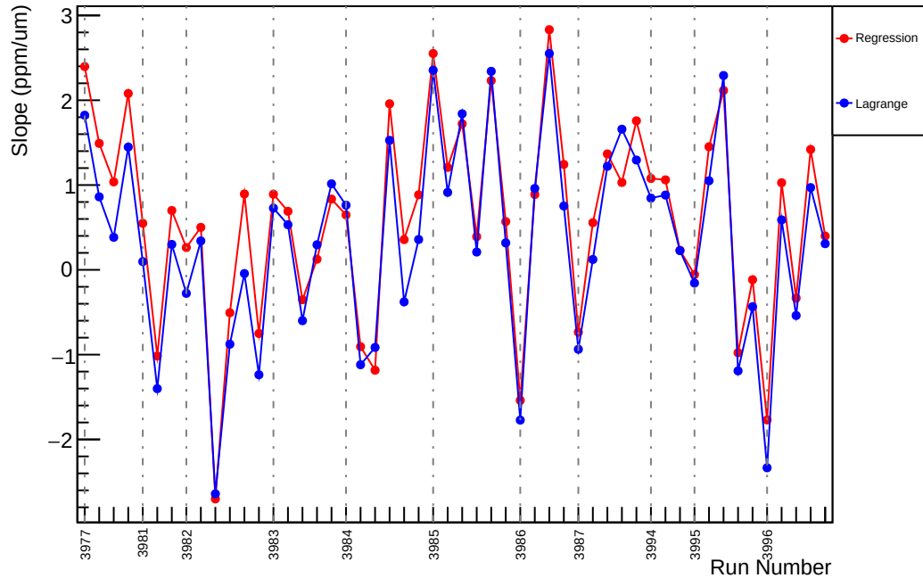
Slug37: Slope : us_dd_vs_evMon6 (ppm/um)
