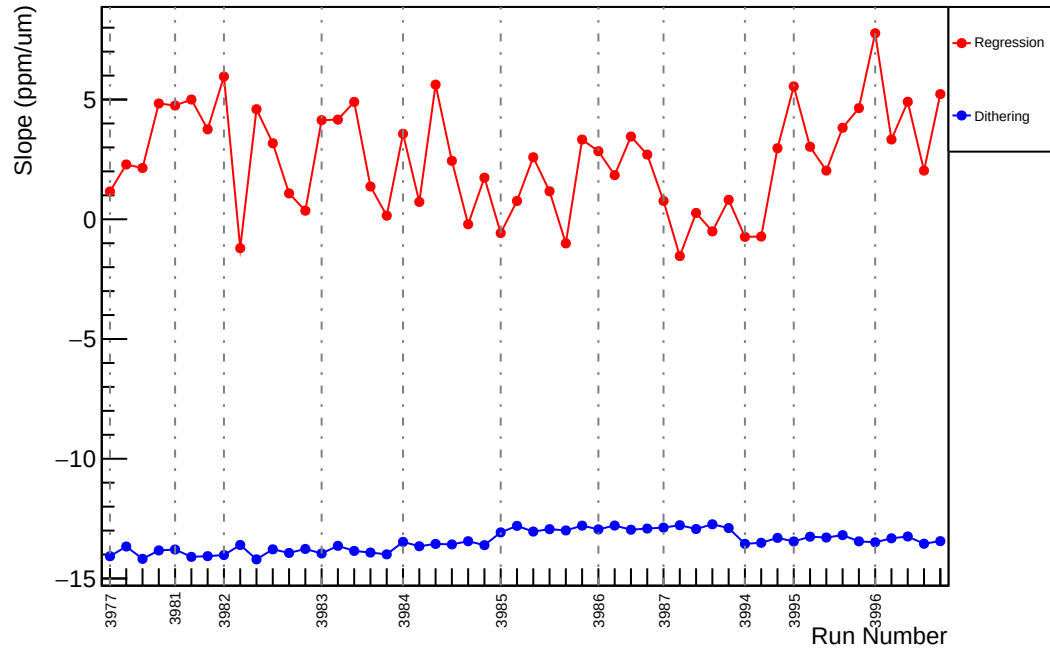
Slug37: Slope : usr_vs_evMon4 (ppm/um)
