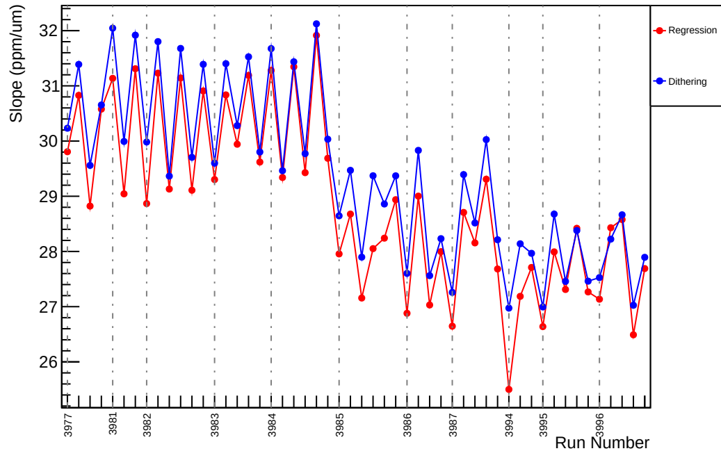
Slug37: Slope : usr_vs_evMon2 (ppm/um)
