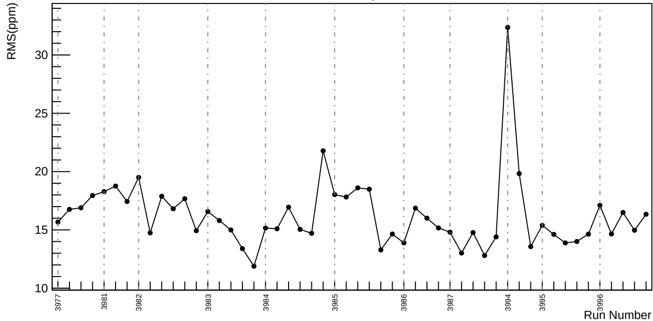
Slug37: asym_usr: \sqrt{\sigma_{\text{dit}}^2 - \sigma_{\text{reg}}^2} (ppm)
