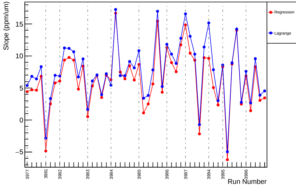
Slug37: Slope : usr_vs_evMon11 (ppm/um)
