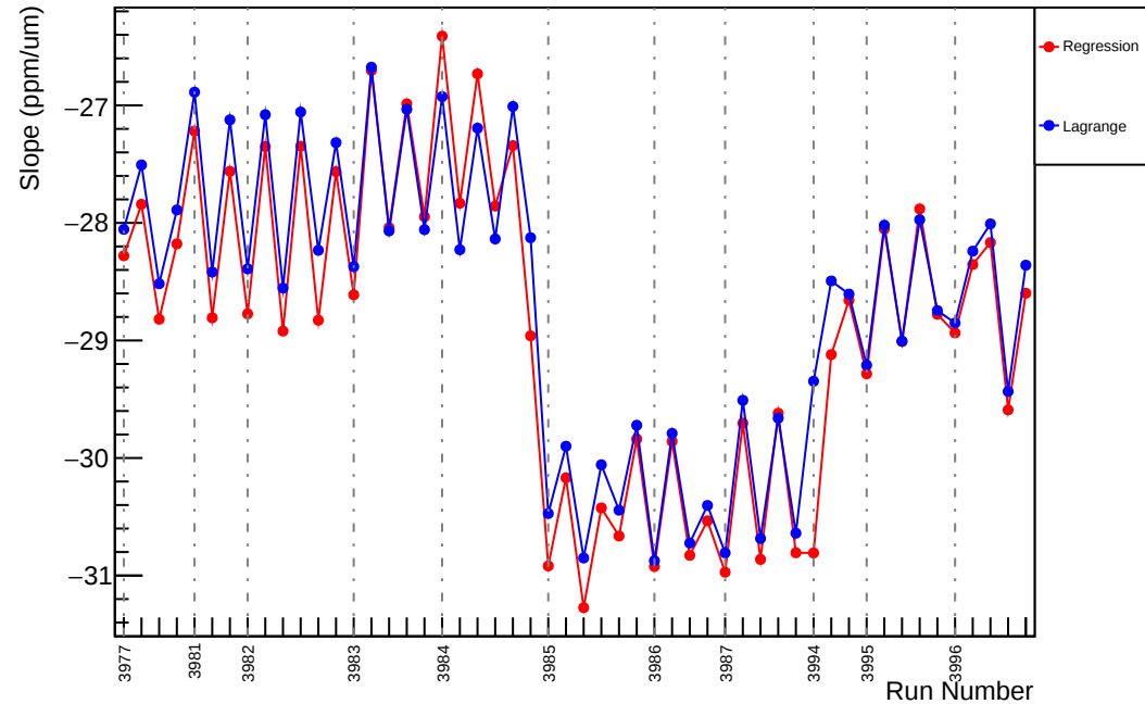
Slug37: Slope : usr_vs_evMon0 (ppm/um)
