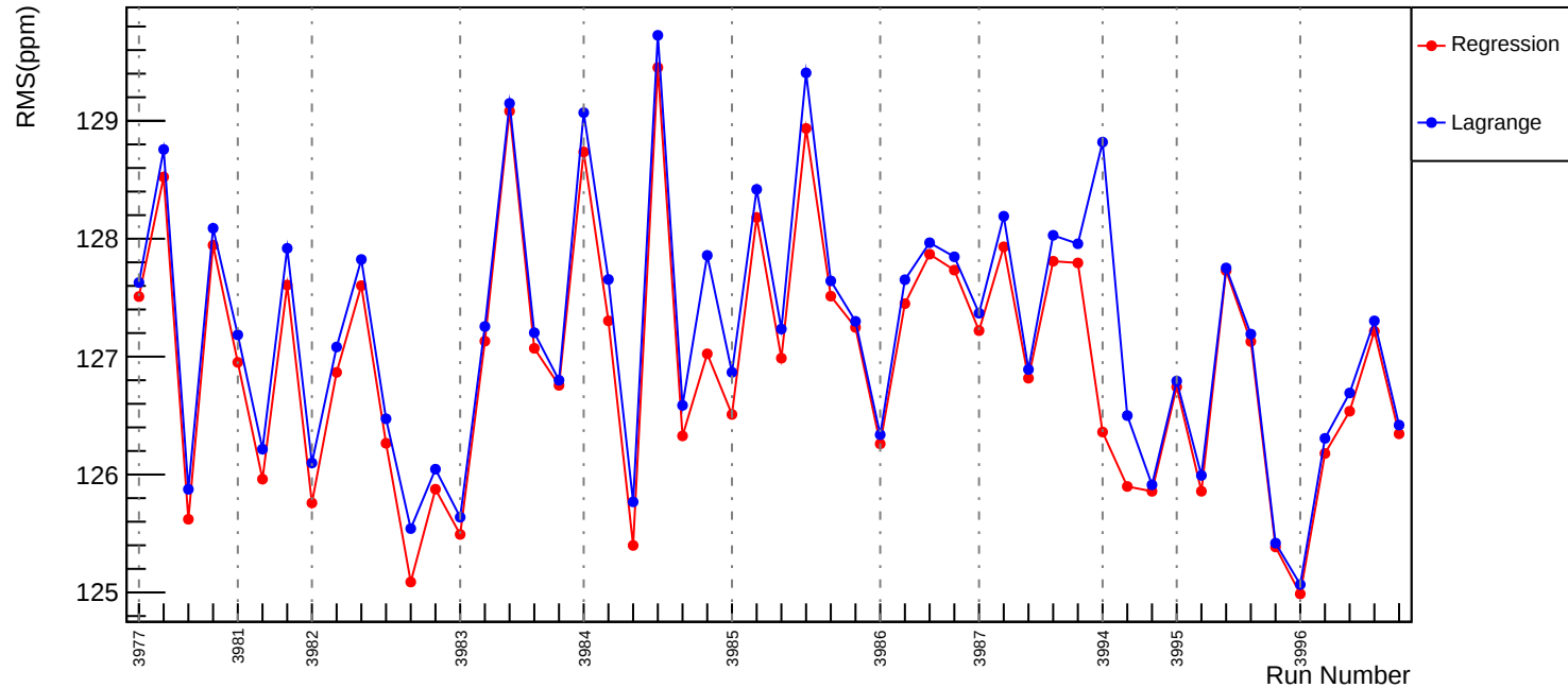
Slug37: Corrected RMS (ppm): asym_usr
