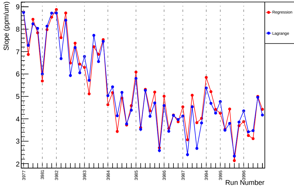
Slug37: Slope : usr_vs_evMon3 (ppm/um)
