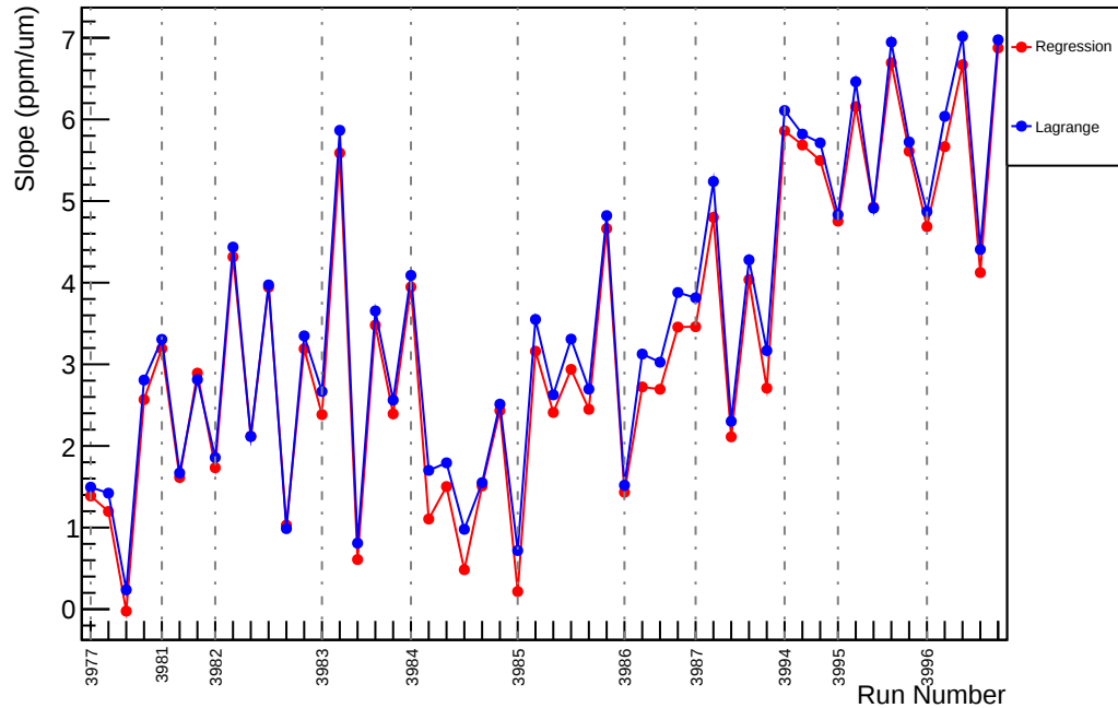
Slug37: Slope : usr_vs_evMon1 (ppm/um)
