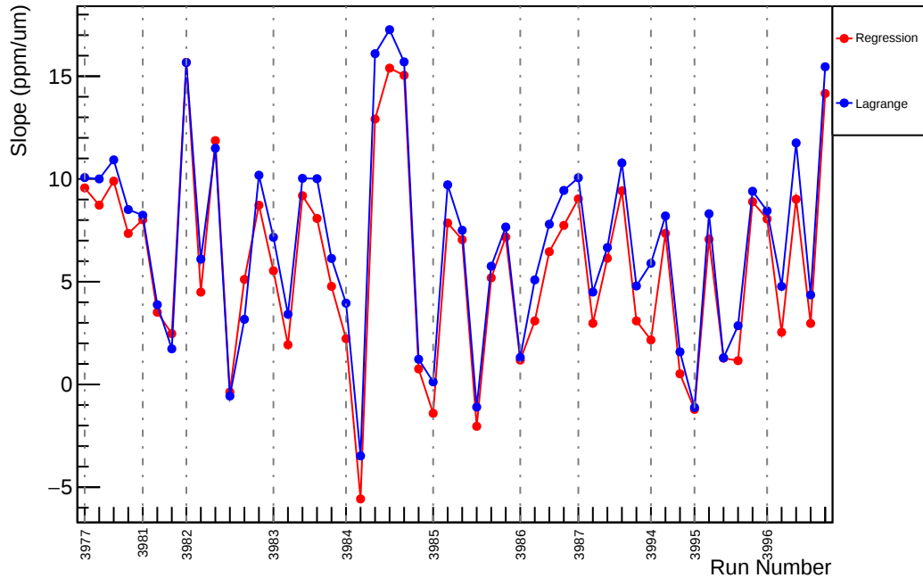
Slug37: Slope : usr_vs_evMon10 (ppm/um)
