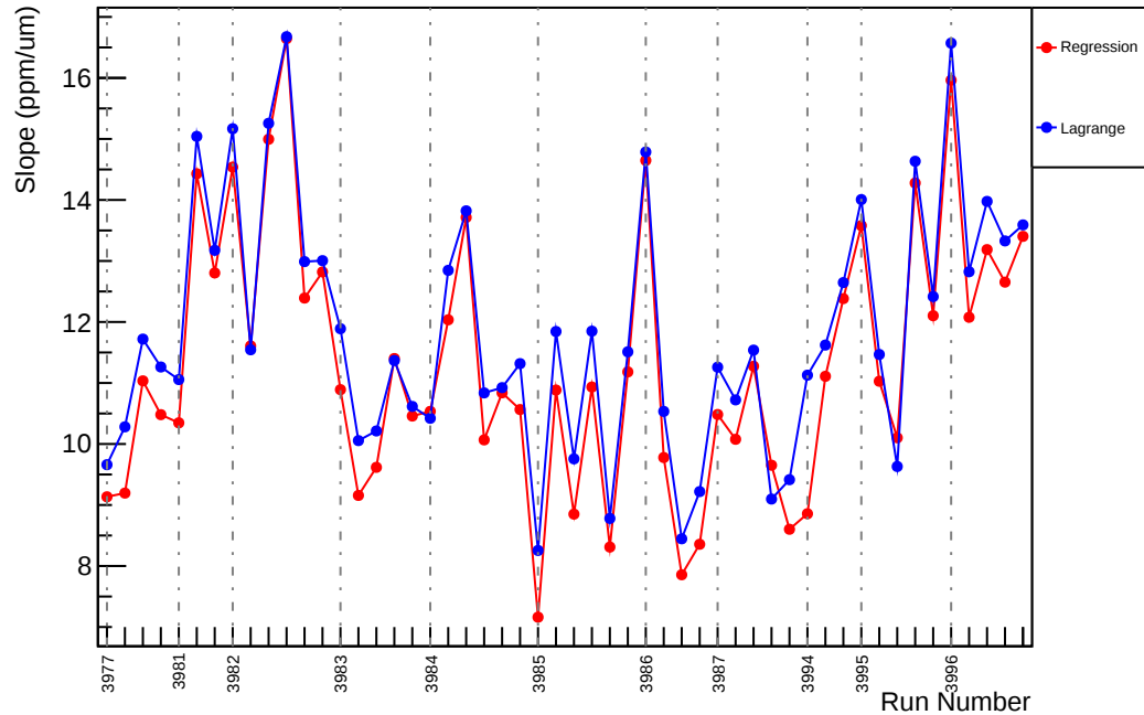
Slug37: Slope : usr_vs_evMon6 (ppm/um)
