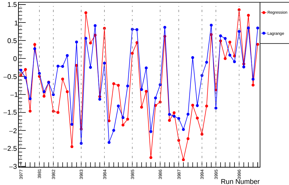
Slug37: Slope : usr_vs_evMon5 (ppm/um)
