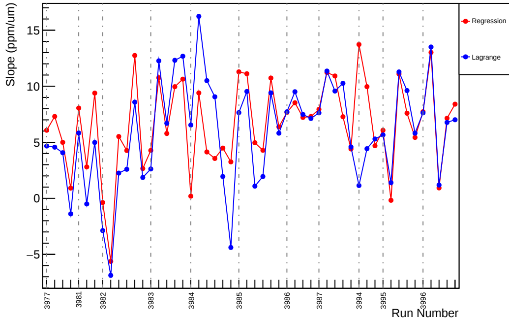
Slug37: Slope : usr_vs_evMon9 (ppm/um)
