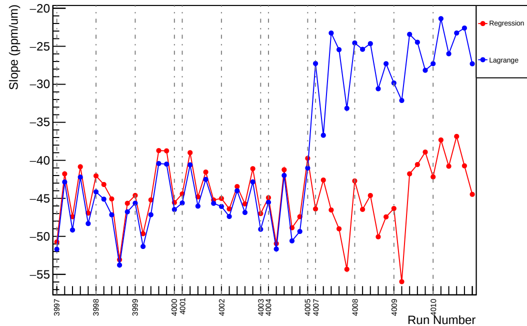
Slug38: Slope : usl_vs_evMon5 (ppm/um)
