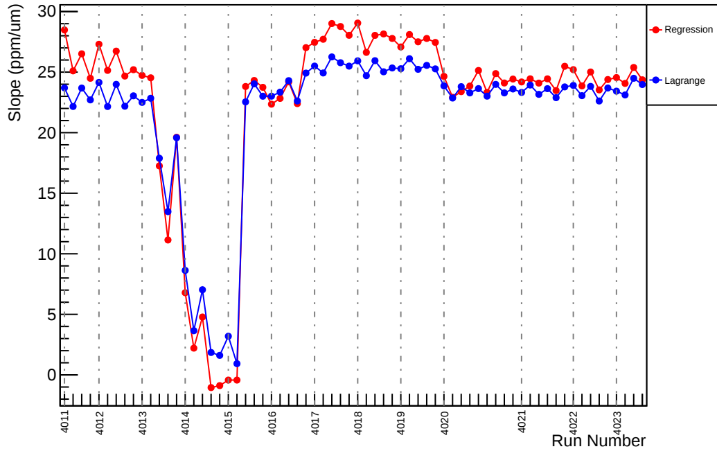
Slug39: Slope : us_avg_vs_evMon3 (ppm/um)
