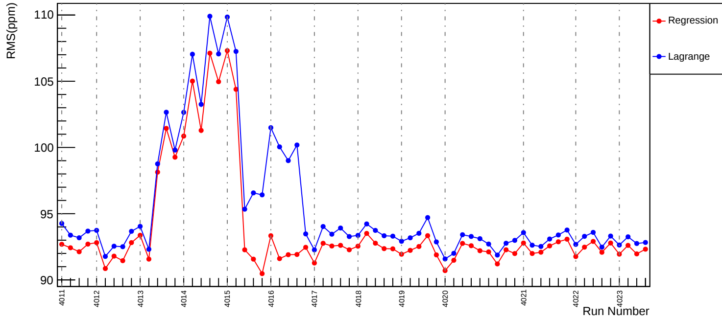
Slug39: Corrected RMS (ppm): asym_us_avg
