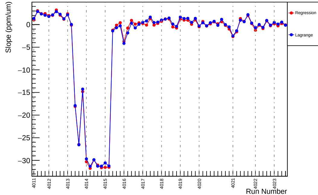
Slug39: Slope : us_avg_vs_evMon5 (ppm/um)
