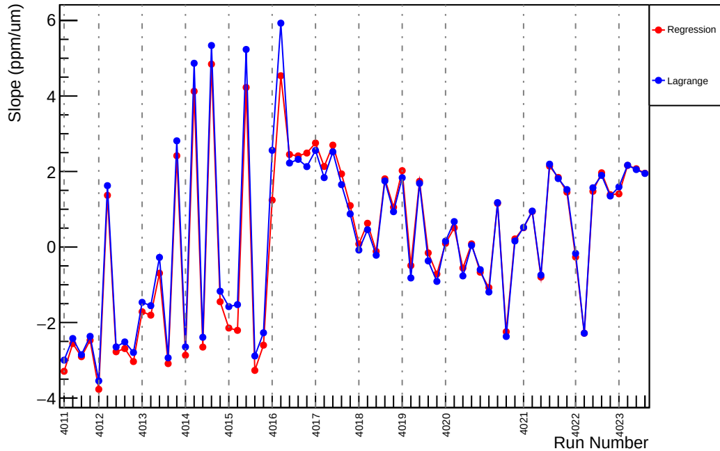
Slug39: Slope : us_avg_vs_evMon1 (ppm/um)
