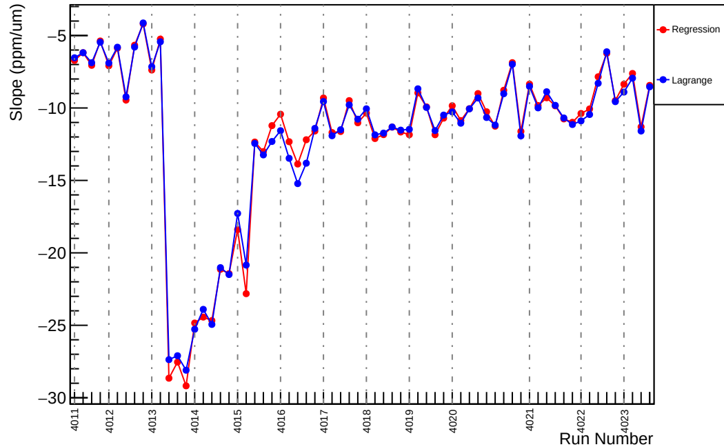
Slug39: Slope : us_avg_vs_evMon6 (ppm/um)
