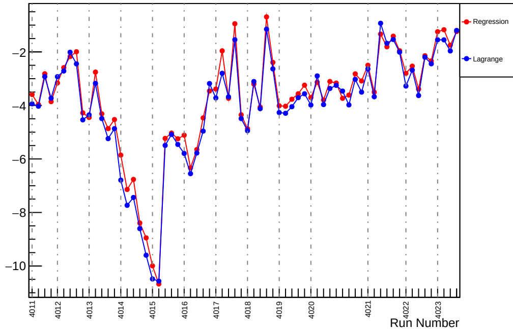
Slug39: Slope : us_avg_vs_evMon3 (ppm/um)
