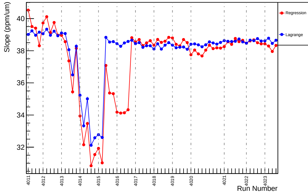
Slug39: Slope : us_avg_vs_evMon2 (ppm/um)
