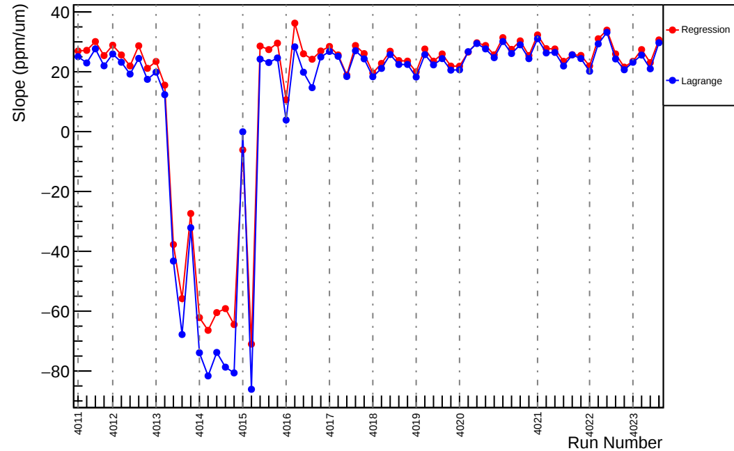
Slug39: Slope : usr_vs_evMon5 (ppm/um)
