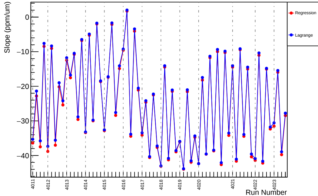
Slug39: Slope : usr_vs_evMon0 (ppm/um)
