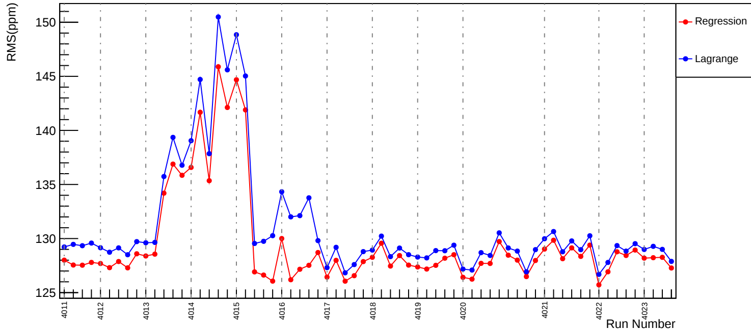
Slug39: Corrected RMS (ppm): asym_usr
