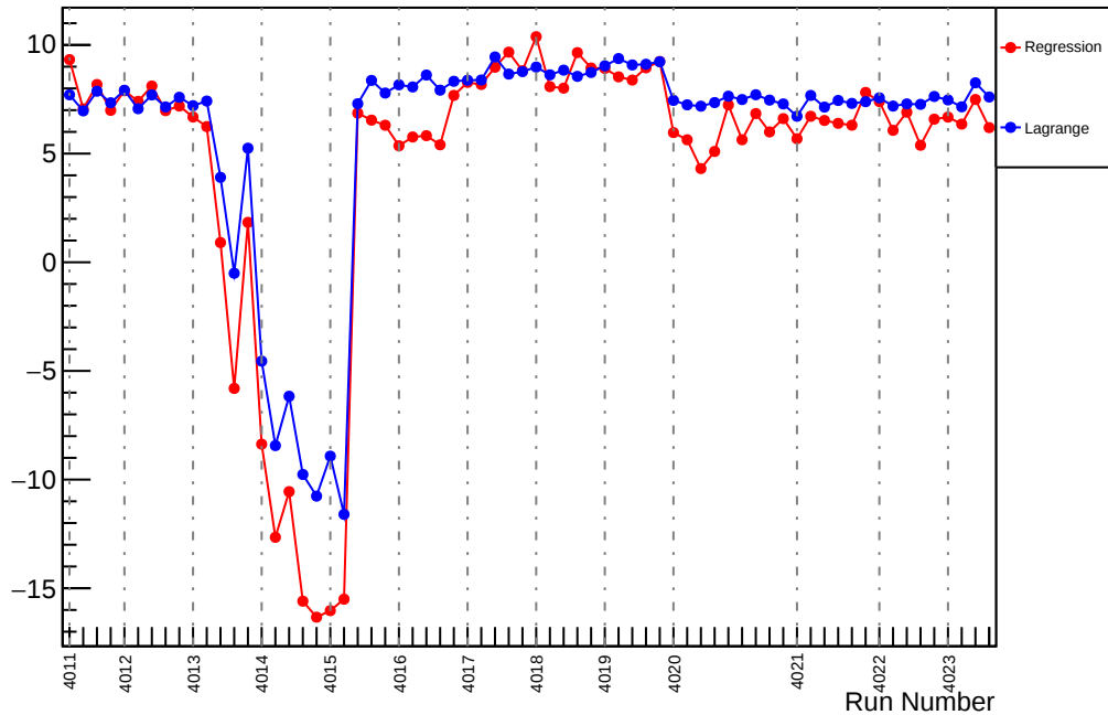
Slug39: Slope : usr_vs_evMon3 (ppm/um)
