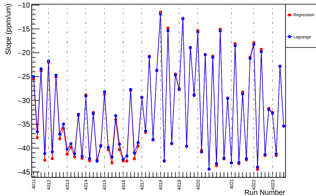
Slug39: Slope : usr_vs_evMon1 (ppm/um)
