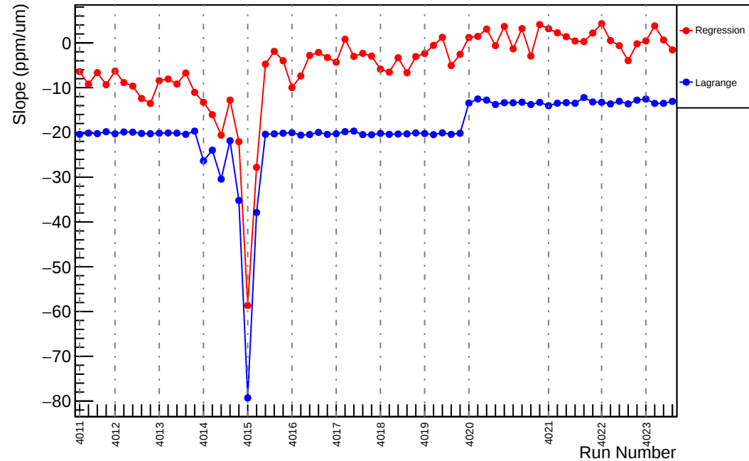
Slug39: Slope : usr_vs_evMon4 (ppm/um)
