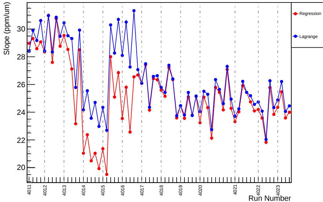
Slug39: Slope : usr_vs_evMon2 (ppm/um)
