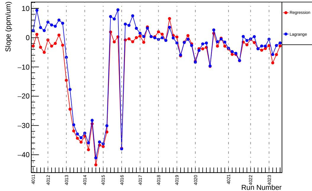
Slug39: Slope : usr_vs_evMon8 (ppm/um)
