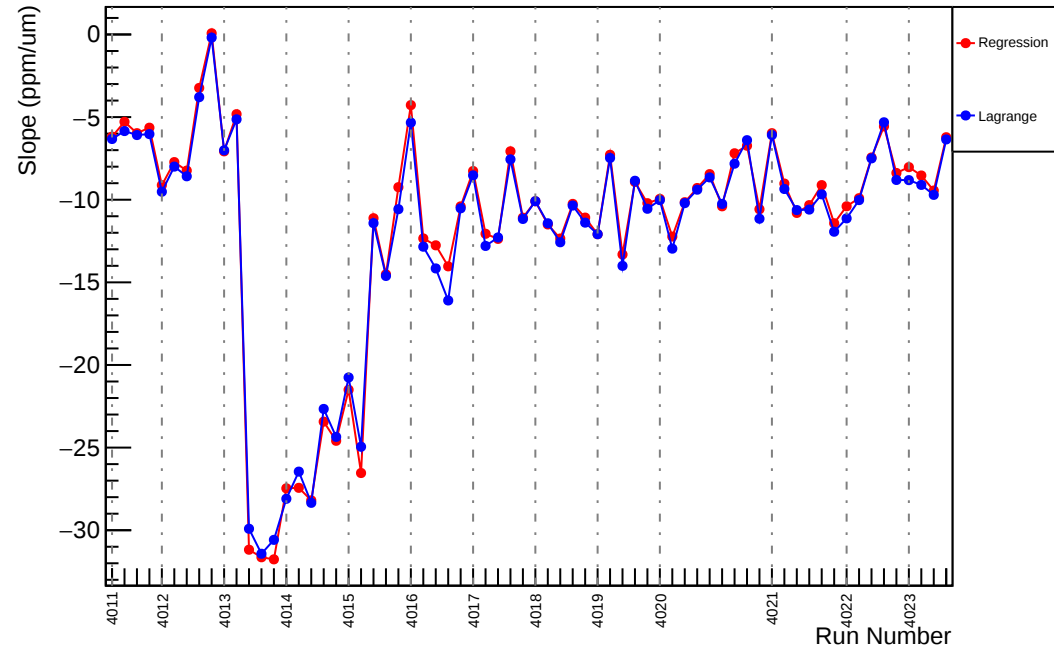
Slug39: Slope : usr_vs_evMon6 (ppm/um)
