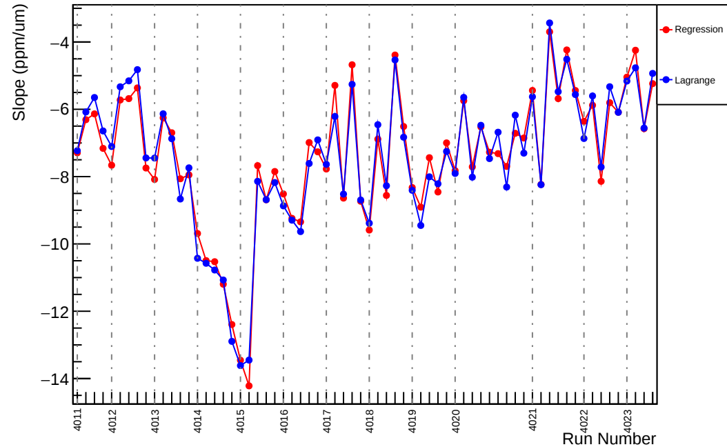
Slug39: Slope : usr_vs_evMon3 (ppm/um)
