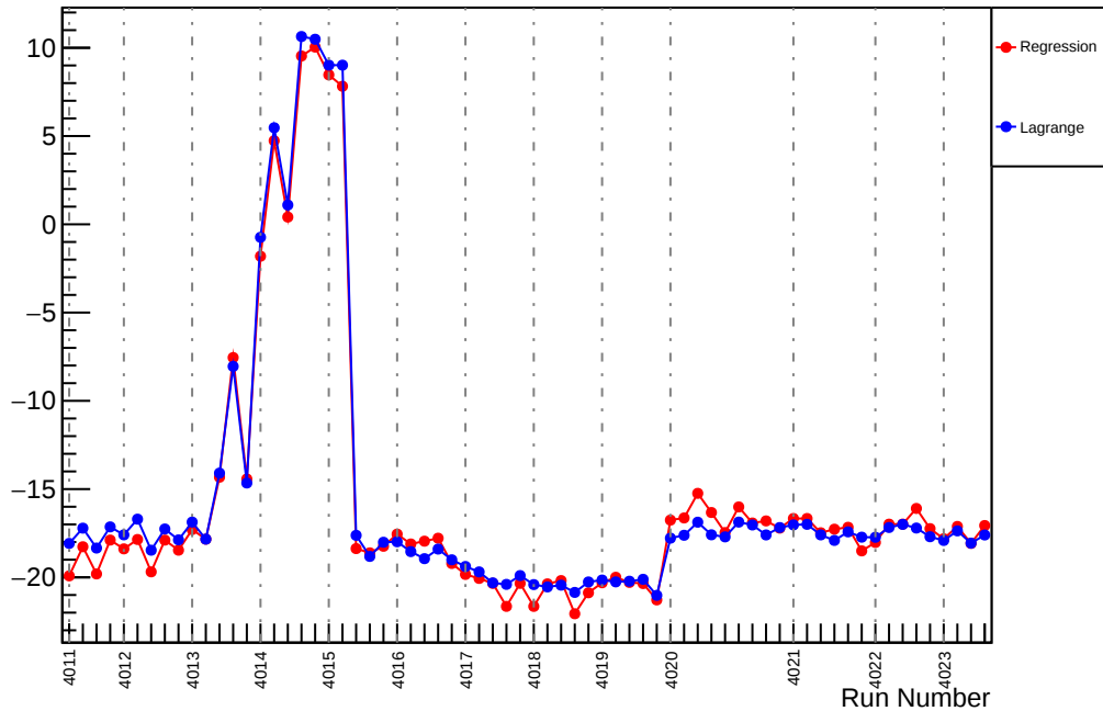
Slug39: Slope : usr_vs_evMon4 (ppm/um)
