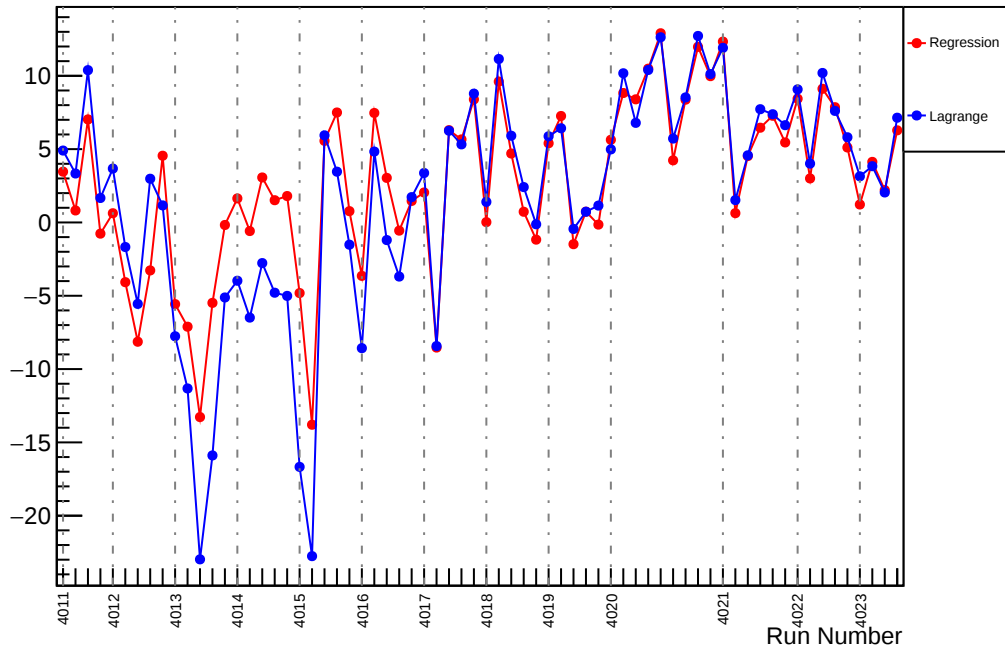
Slug39: Slope : usr_vs_evMon10 (ppm/um)
