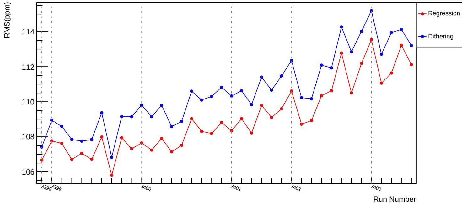
Slug3: Corrected RMS (ppm): asym_us_avg
