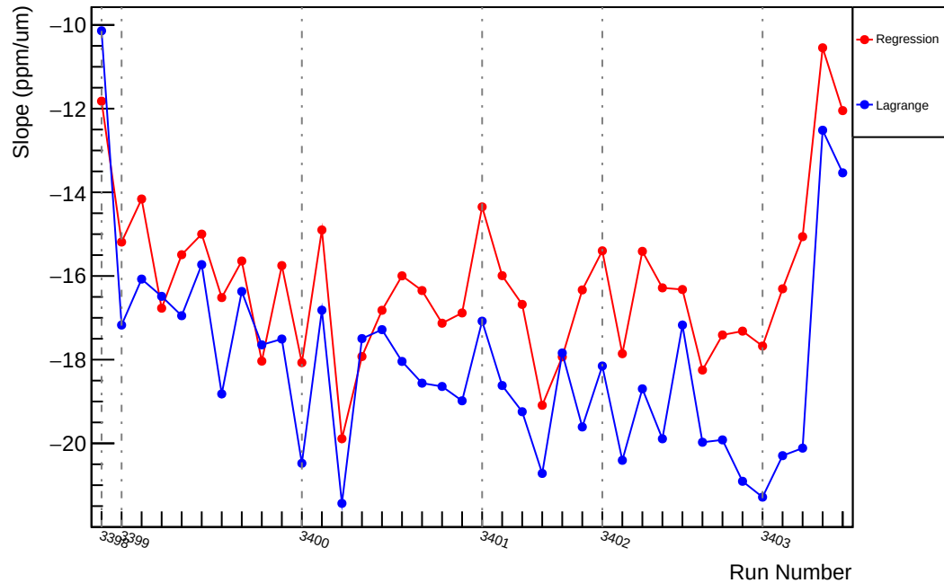
Slug3: Slope : us_avg_vs_evMon3 (ppm/um)
