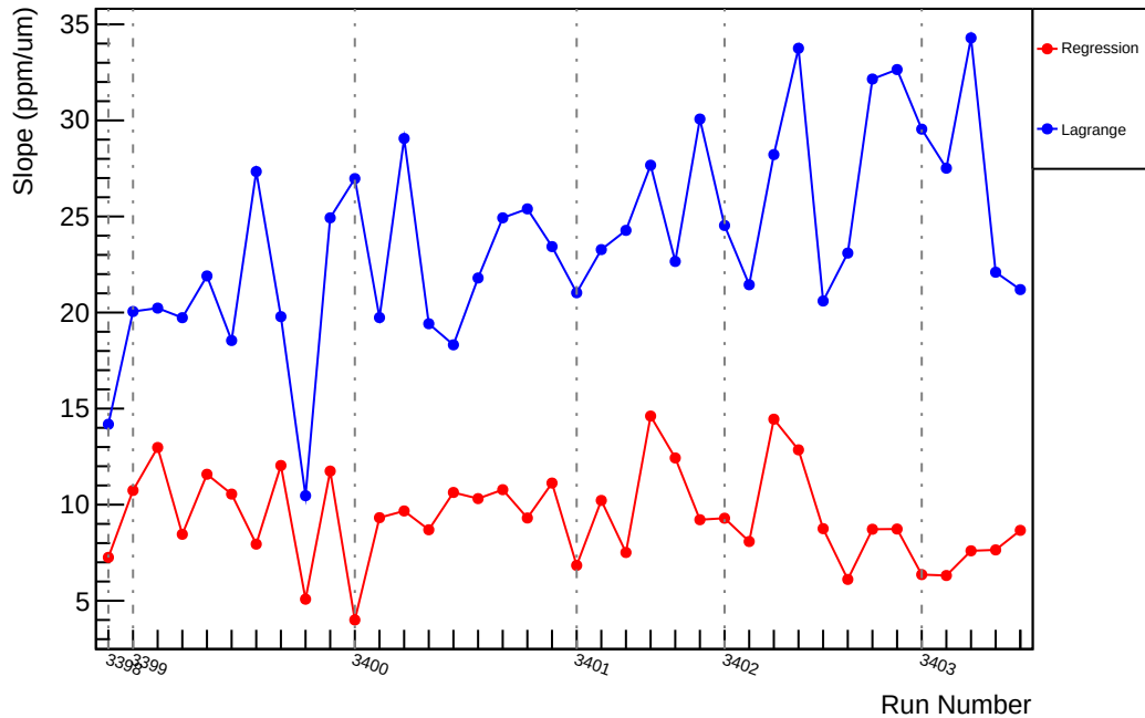
Slug3: Slope : us_avg_vs_evMon5 (ppm/um)
