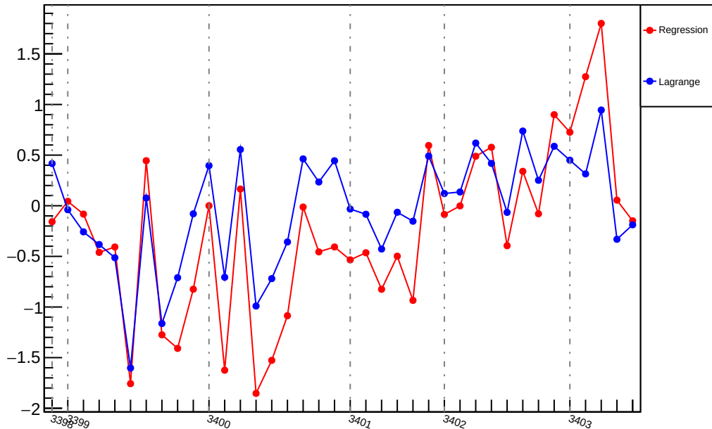
Slug3: Slope : us_avg_vs_evMon0 (ppm/um)
