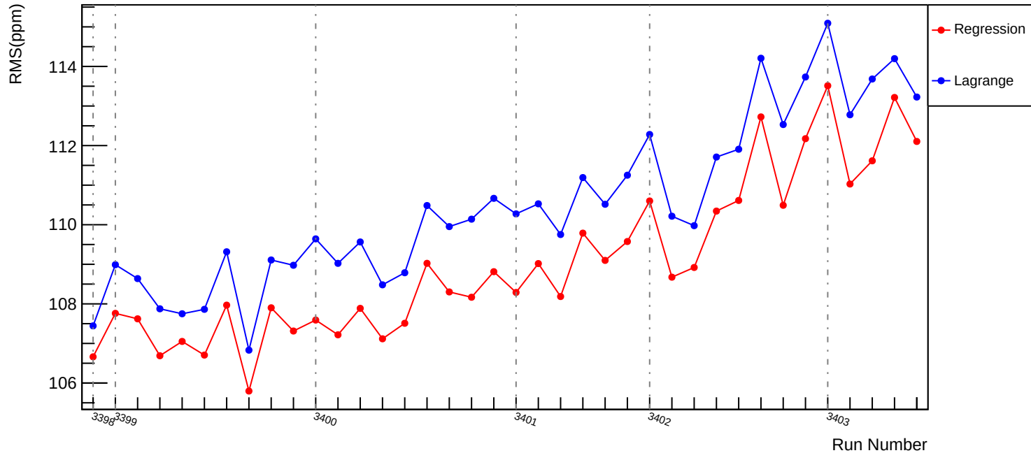
Slug3: Corrected RMS (ppm): asym_us_avg
