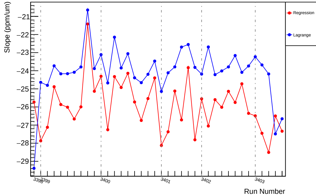
Slug3: Slope : us_avg_vs_evMon4 (ppm/um)
