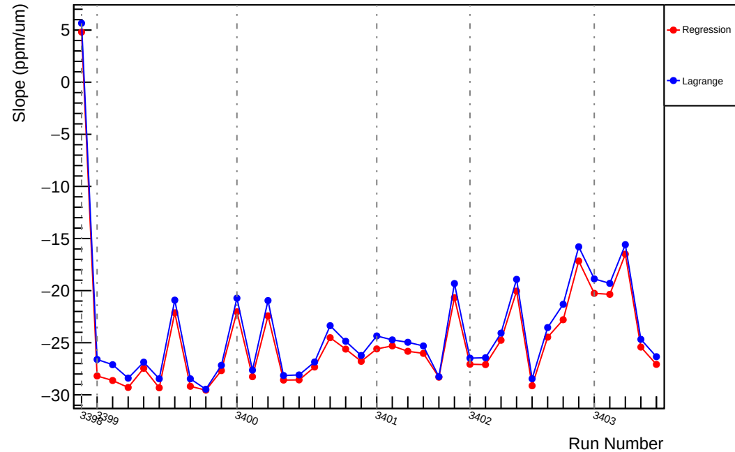
Slug3: Slope : us_avg_vs_evMon1 (ppm/um)
