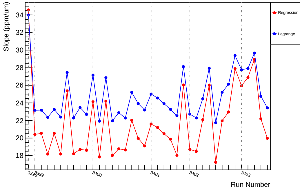
Slug3: Slope : us_avg_vs_evMon2 (ppm/um)
