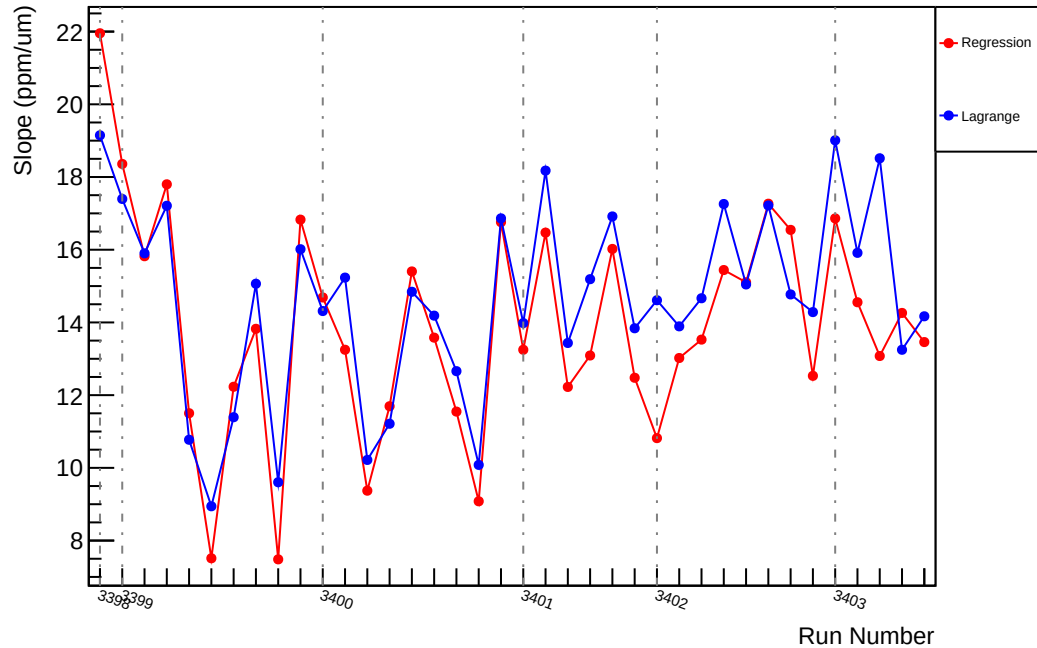
Slug3: Slope : usl_vs_evMon7 (ppm/um)
