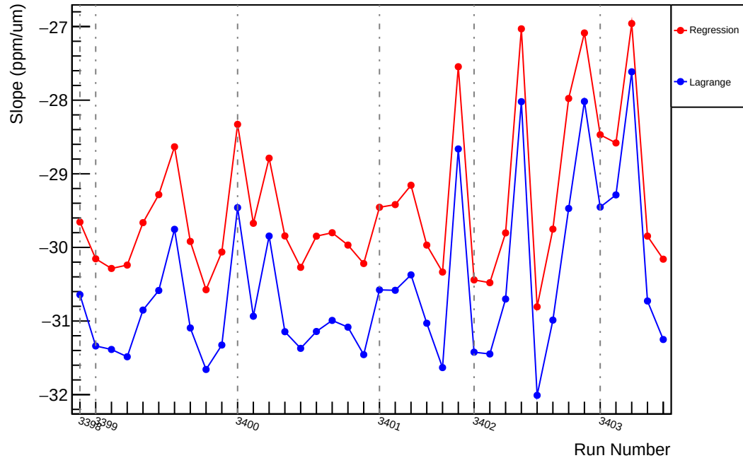
Slug3: Slope : usl_vs_evMon0 (ppm/um)
