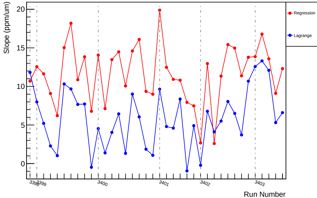
Slug3: Slope : usl_vs_evMon9 (ppm/um)
