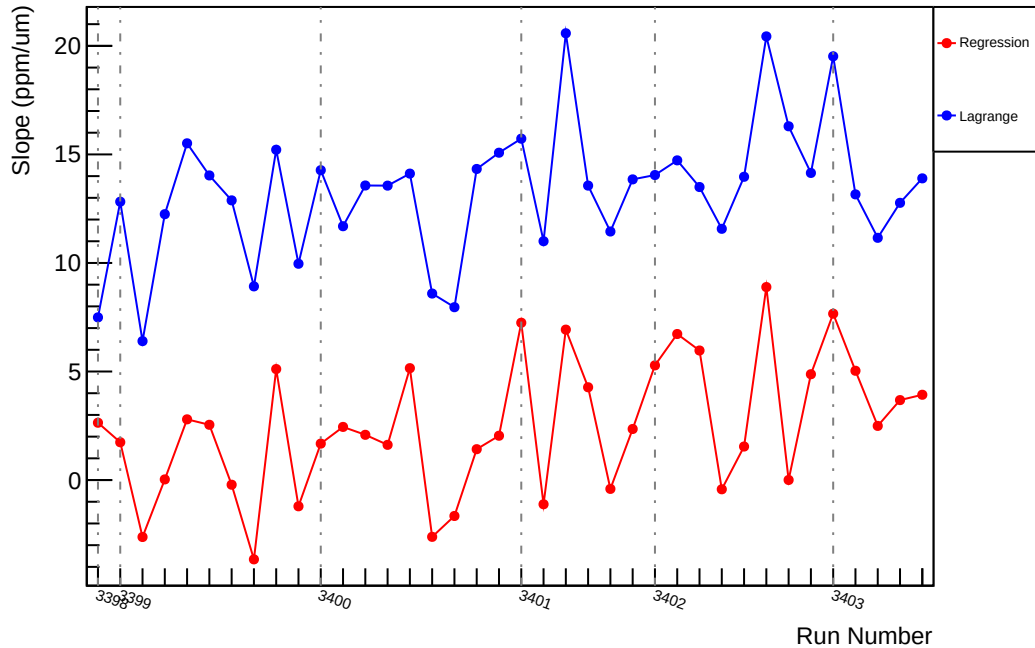
Slug3: Slope : usl_vs_evMon8 (ppm/um)
