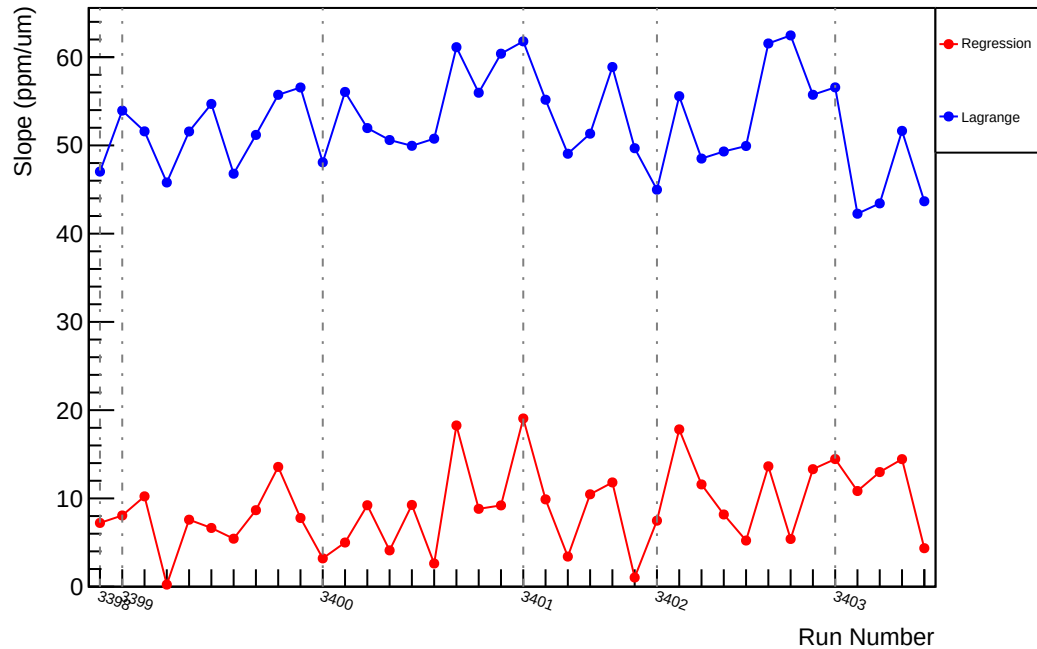
Slug3: Slope : usl_vs_evMon10 (ppm/um)
