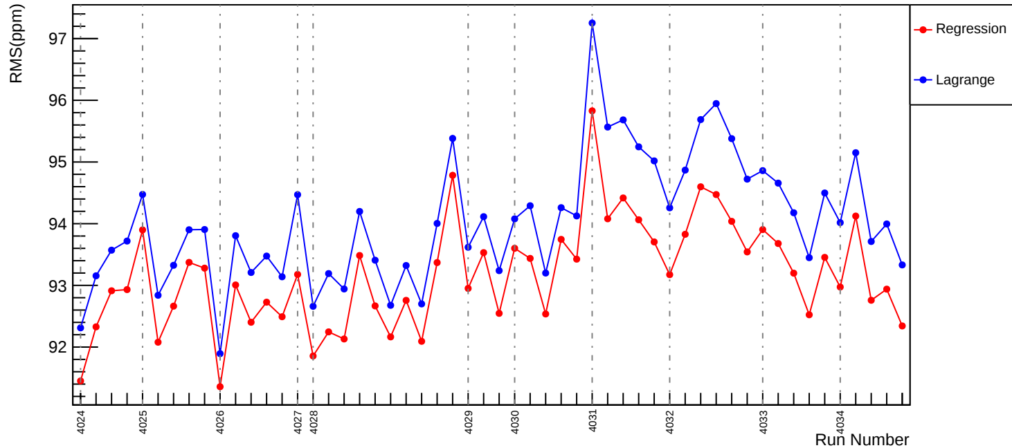
Slug40: Corrected RMS (ppm): asym_us_avg
