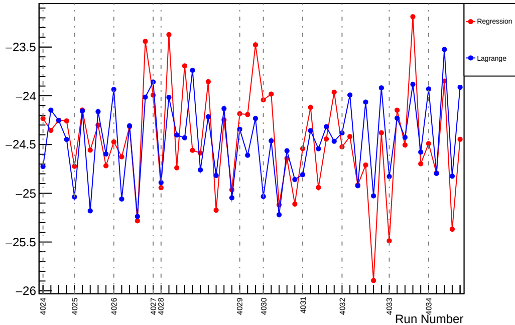
Slug40: Slope : us_avg_vs_evMon3 (ppm/um)
