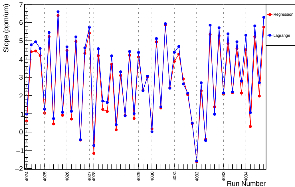
Slug40: Slope : us_avg_vs_evMon0 (ppm/um)
