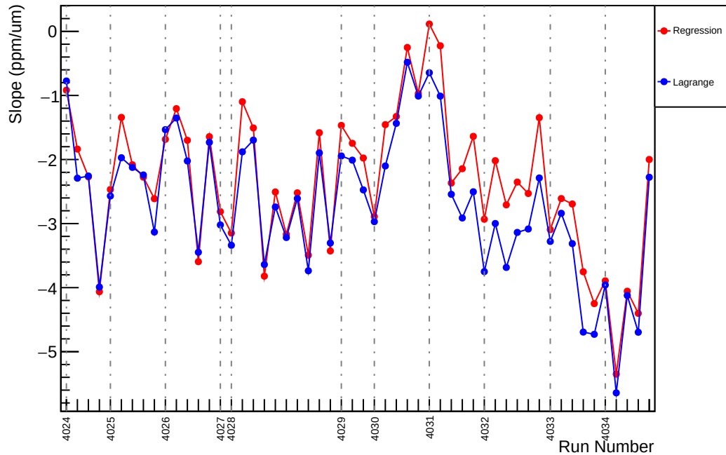
Slug40: Slope : us_avg_vs_evMon3 (ppm/um)
