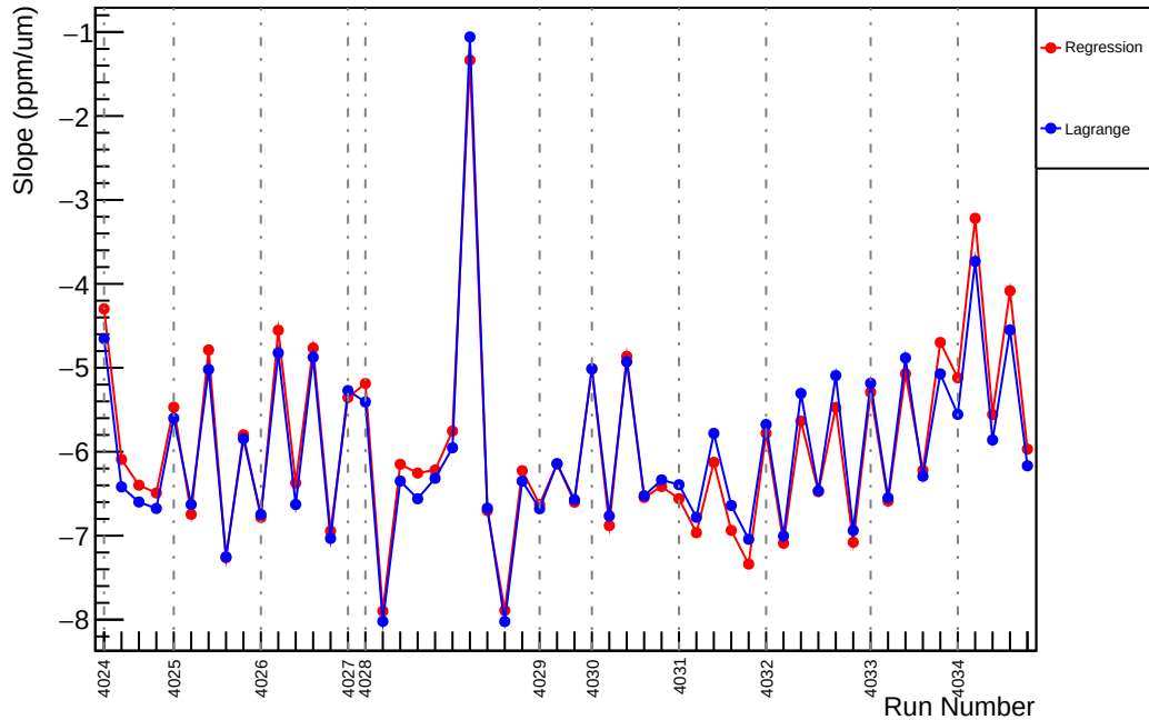
Slug40: Slope : us_avg_vs_evMon0 (ppm/um)
