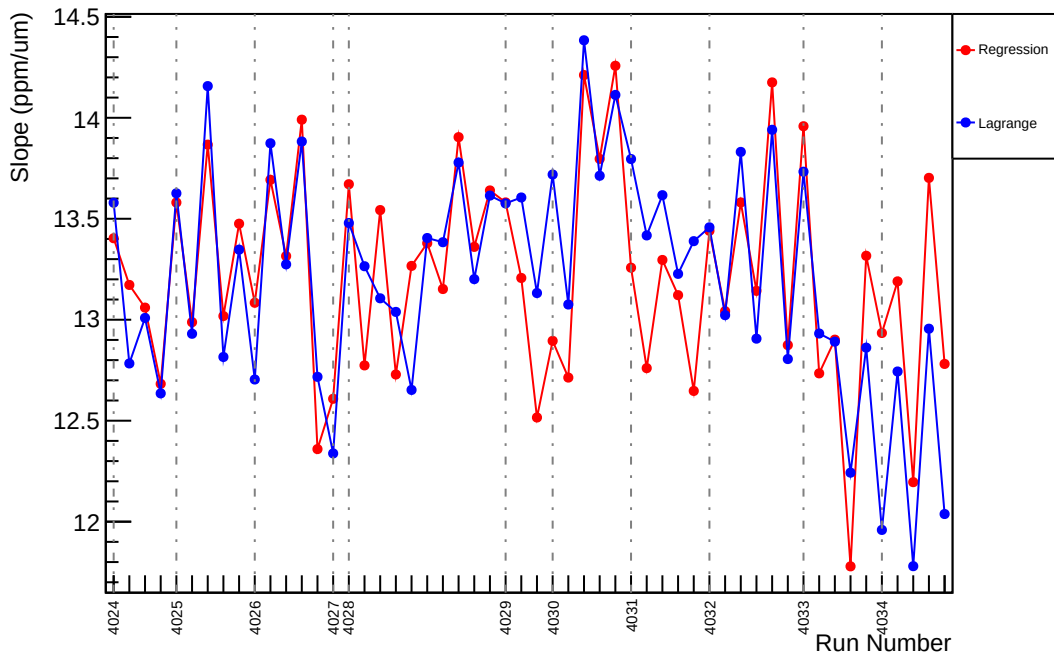
Slug40: Slope : us_avg_vs_evMon4 (ppm/um)
