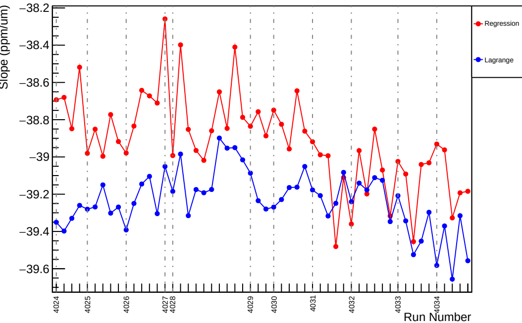
Slug40: Slope : us_avg_vs_evMon2 (ppm/um)
