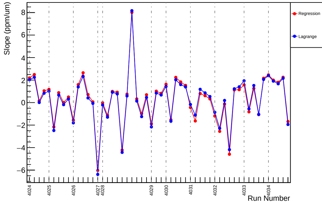
Slug40: Slope : us_avg_vs_evMon1 (ppm/um)
