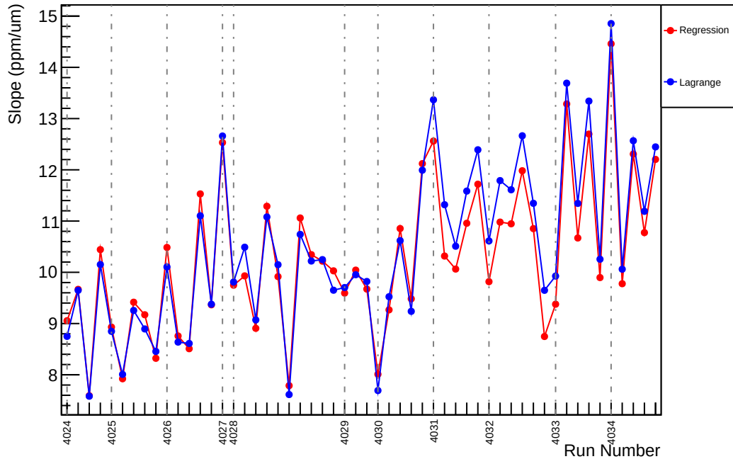
Slug40: Slope : us_avg_vs_evMon6 (ppm/um)
