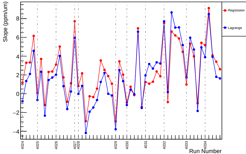
Slug40: Slope : us_avg_vs_evMon11 (ppm/um)
