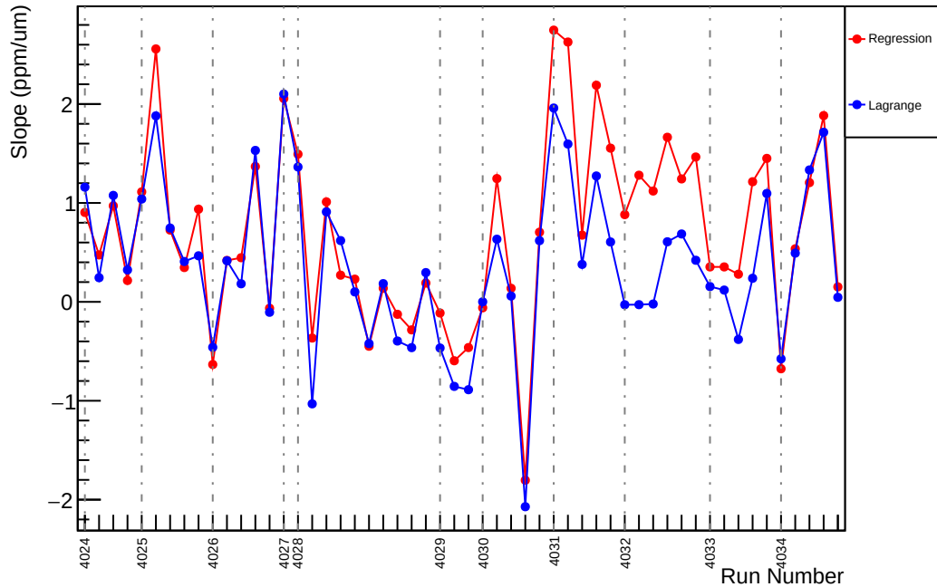
Slug40: Slope : us_avg_vs_evMon5 (ppm/um)
