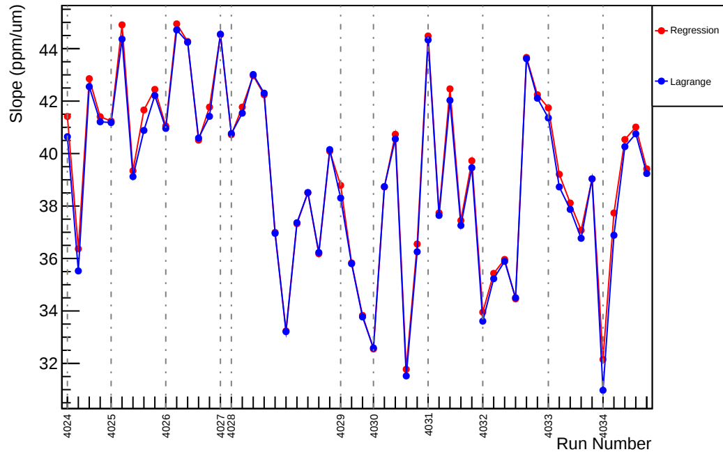
Slug40: Slope : us_dd_vs_evMon5 (ppm/um)
