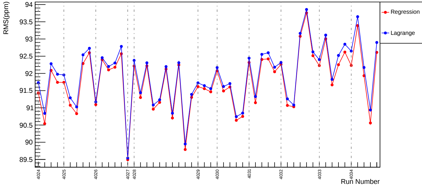
Slug40: Corrected RMS (ppm): asym_us_dd
