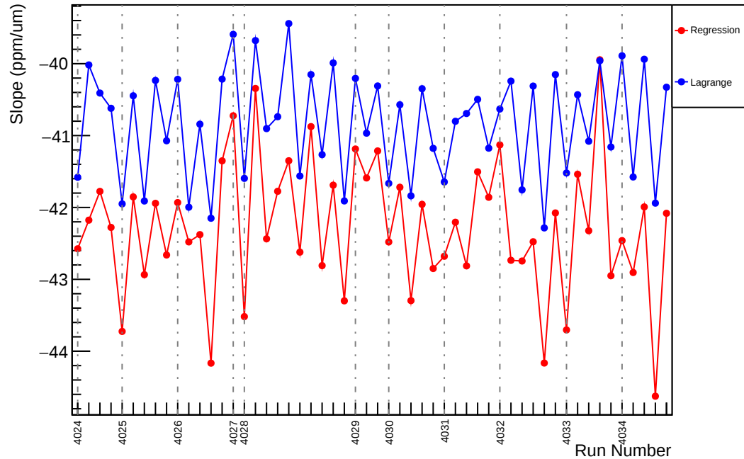
Slug40: Slope : usl_vs_evMon3 (ppm/um)
