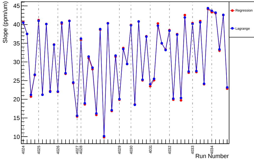
Slug40: Slope : usl_vs_evMon0 (ppm/um)
