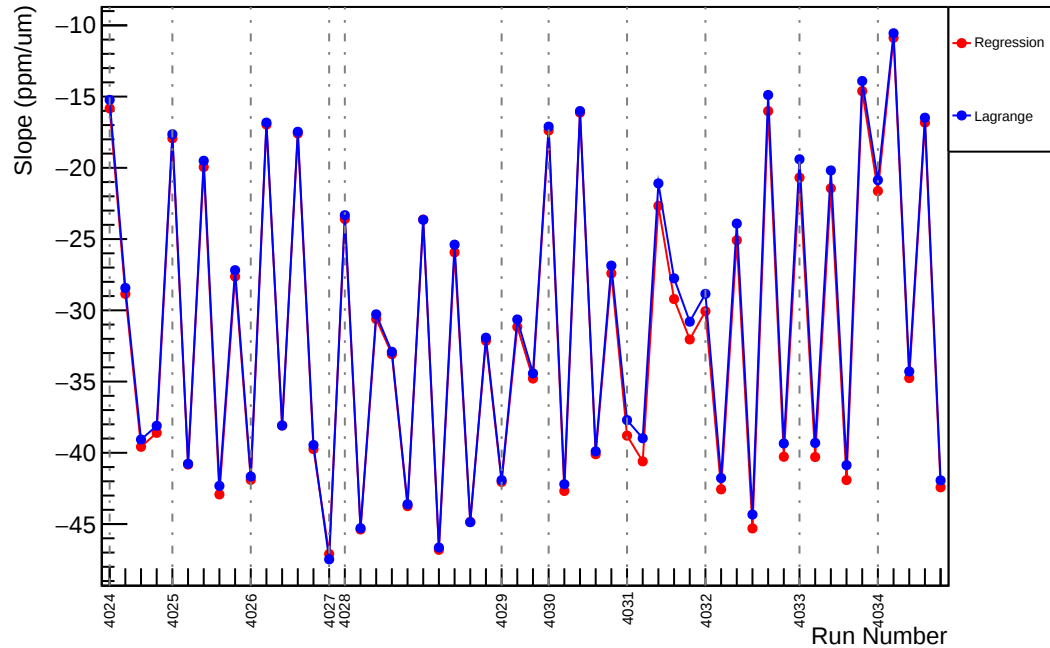
Slug40: Slope : usl_vs_evMon1 (ppm/um)
