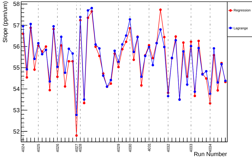
Slug40: Slope : usl_vs_evMon2 (ppm/um)
