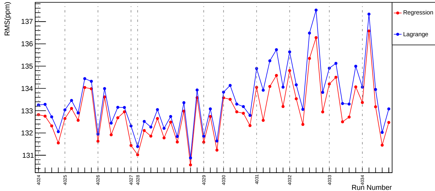
Slug40: Corrected RMS (ppm): asym_usl
