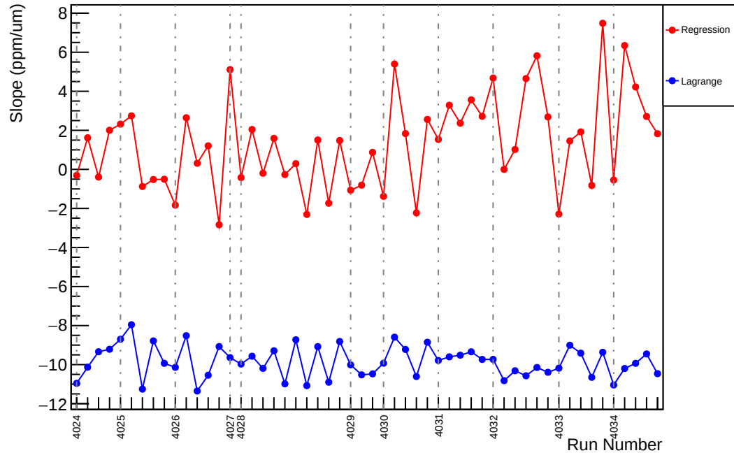
Slug40: Slope : usl_vs_evMon4 (ppm/um)
