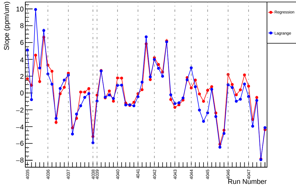
Slug41: Slope : us_avg_vs_evMon9 (ppm/um)
