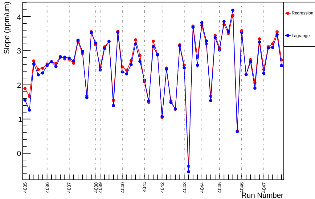
Slug41: Slope : us_avg_vs_evMon1 (ppm/um)
