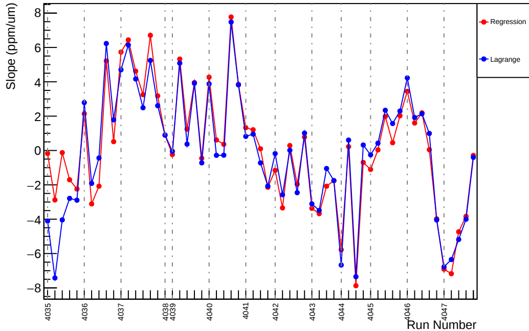
Slug41: Slope : us_avg_vs_evMon10 (ppm/um)
