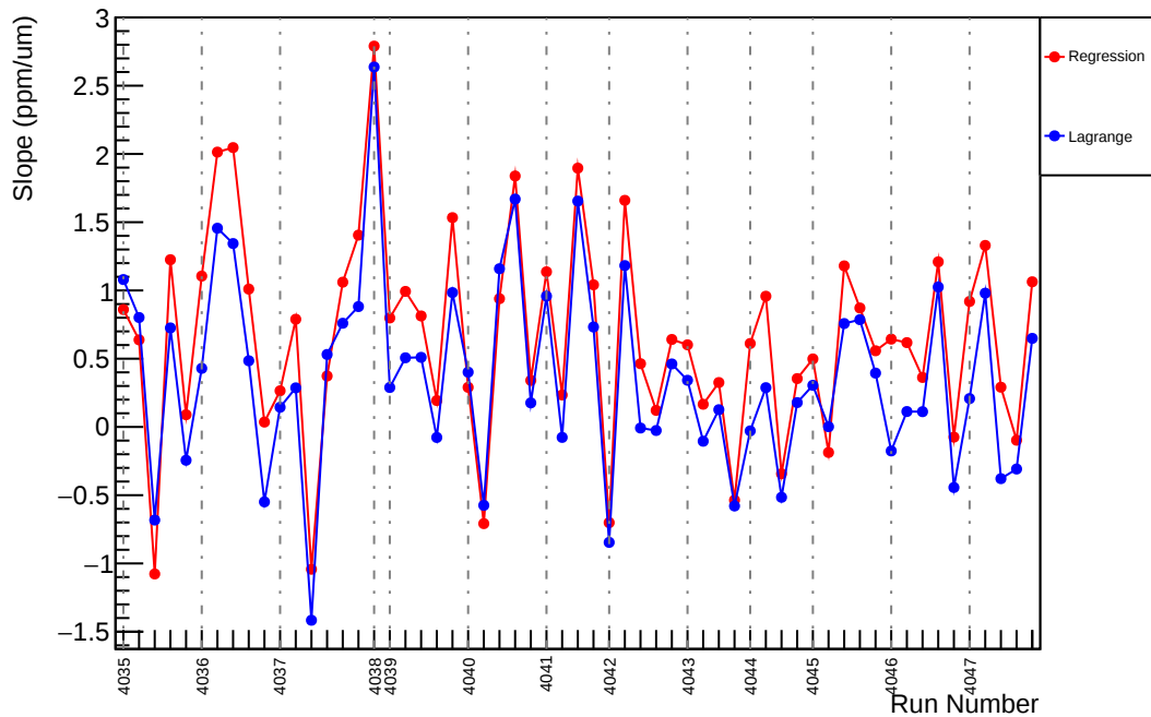
Slug41: Slope : us_avg_vs_evMon5 (ppm/um)
