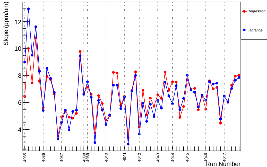
Slug41: Slope : us_avg_vs_evMon7 (ppm/um)
