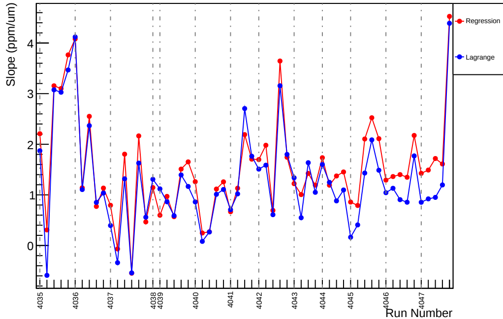
Slug41: Slope : us_dd_vs_evMon5 (ppm/um)
