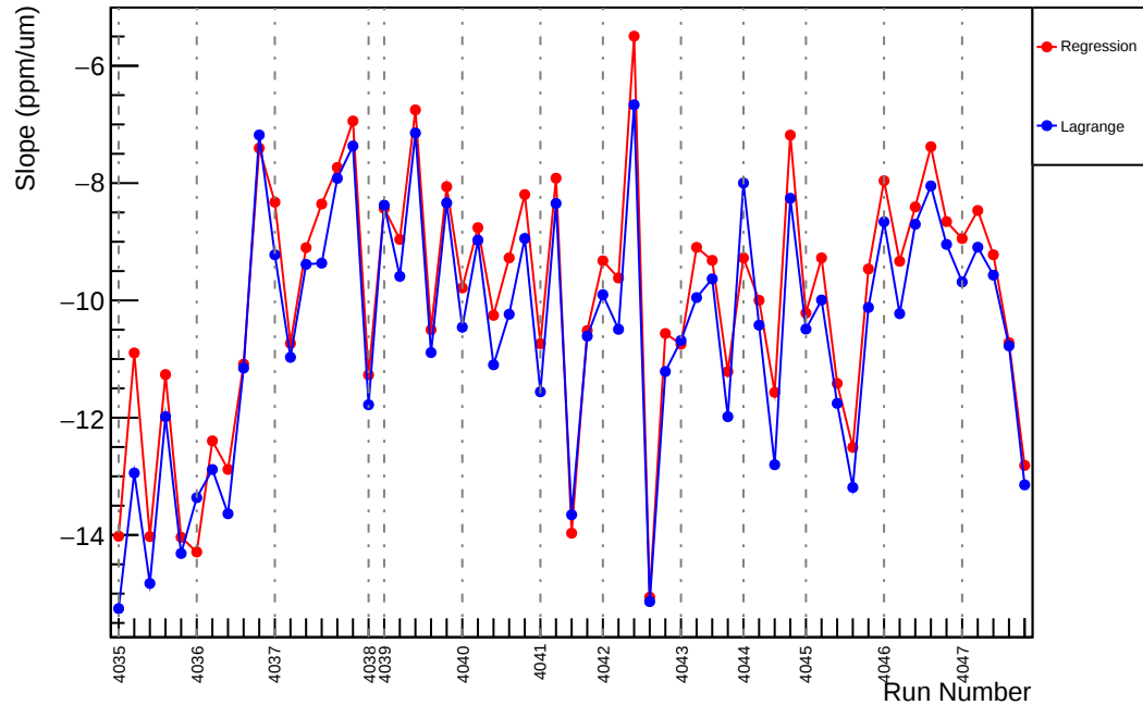
Slug41: Slope : us_dd_vs_evMon7 (ppm/um)
