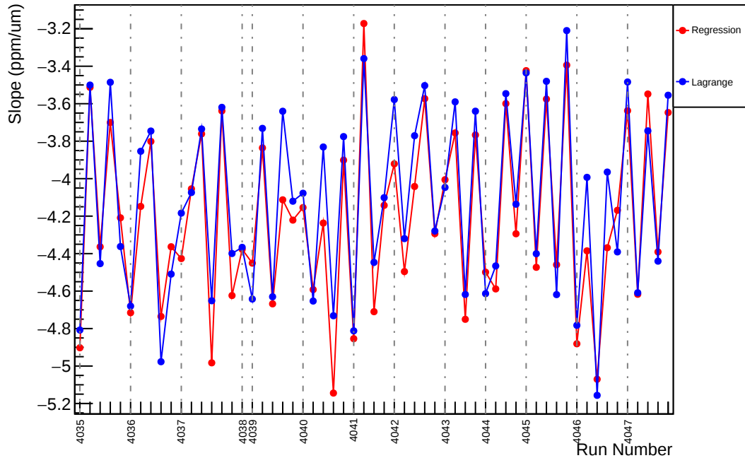
Slug41: Slope : us_dd_vs_evMon2 (ppm/um)
