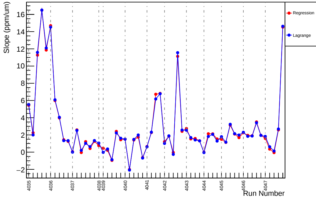
Slug41: Slope : us_dd_vs_evMon6 (ppm/um)
