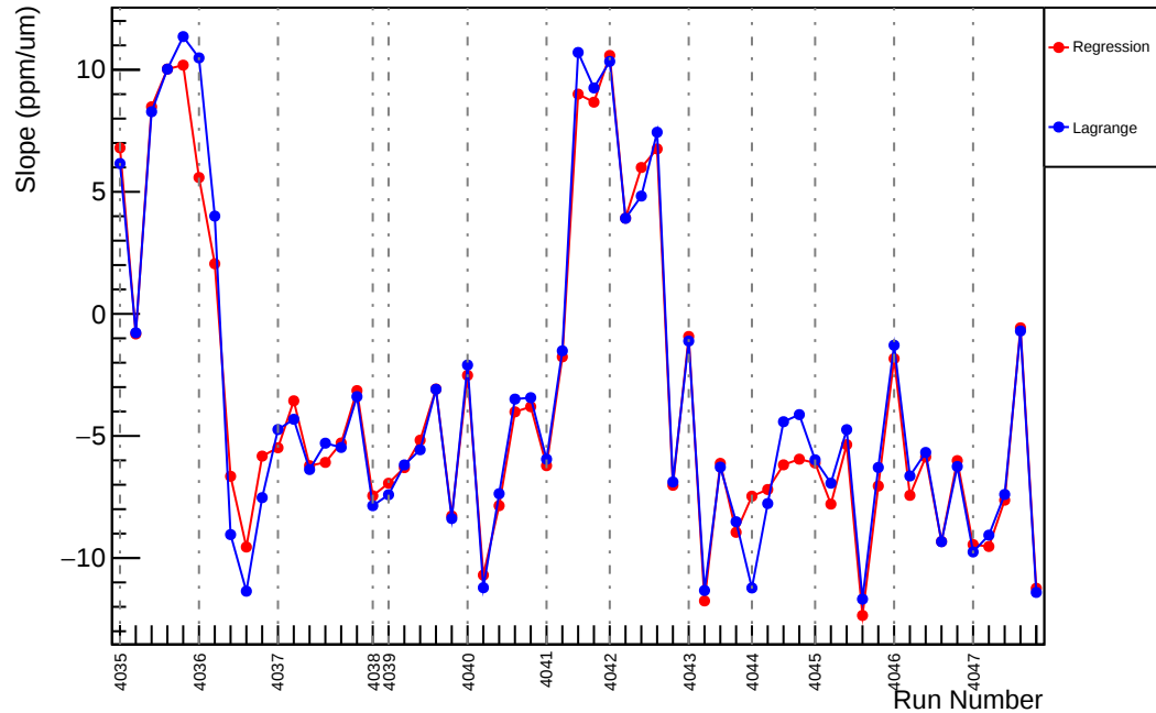
Slug41: Slope : us_dd_vs_evMon9 (ppm/um)
