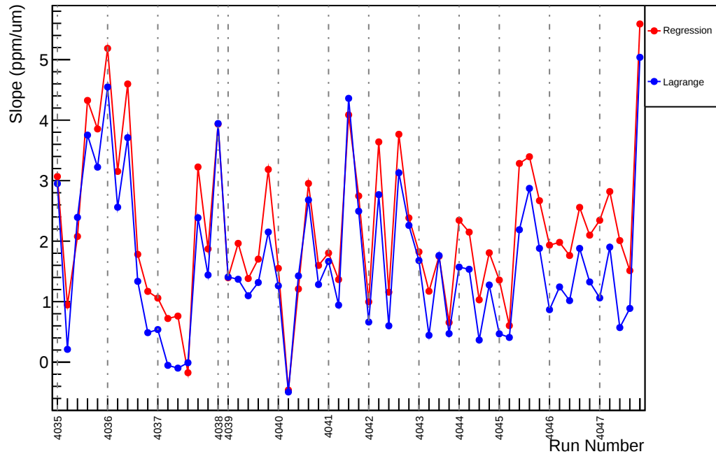
Slug41: Slope : usl_vs_evMon5 (ppm/um)
