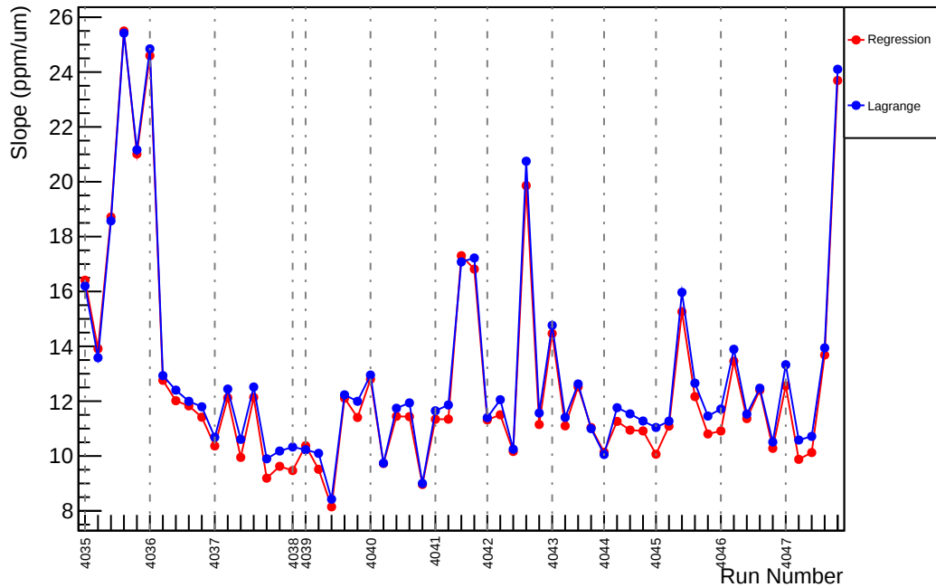
Slug41: Slope : usl_vs_evMon6 (ppm/um)
