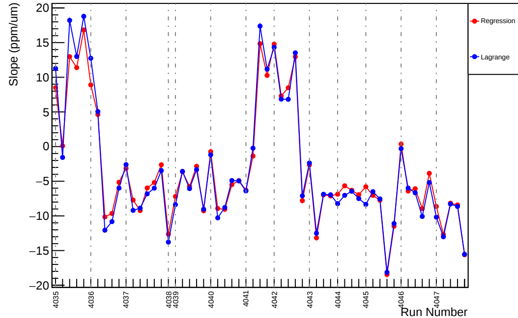
Slug41: Slope : usl_vs_evMon9 (ppm/um)
