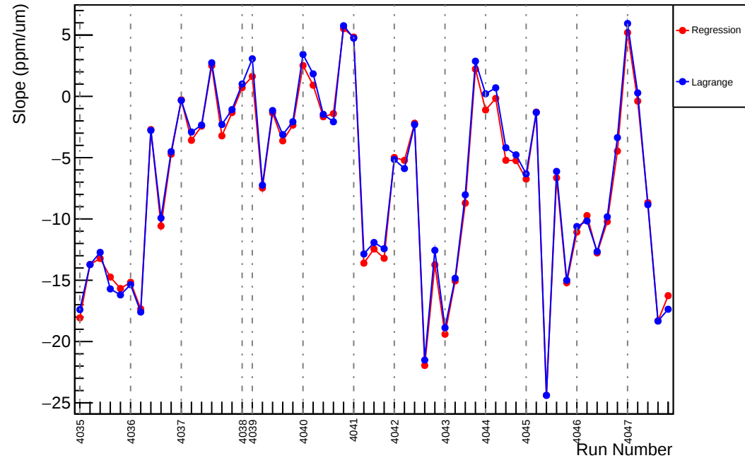
Slug41: Slope : usl_vs_evMon11 (ppm/um)
