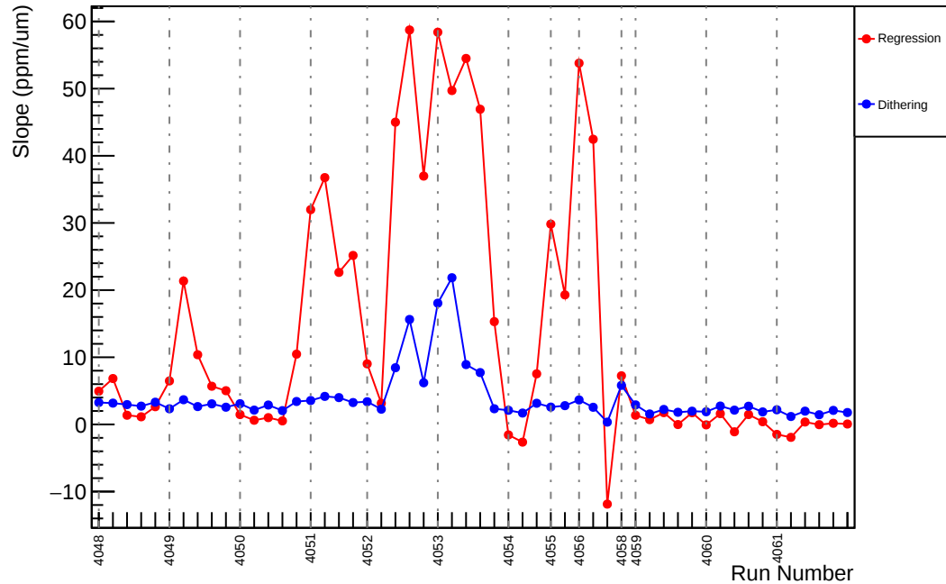
Slug42: Slope : us_dd_vs_evMon4 (ppm/um)
