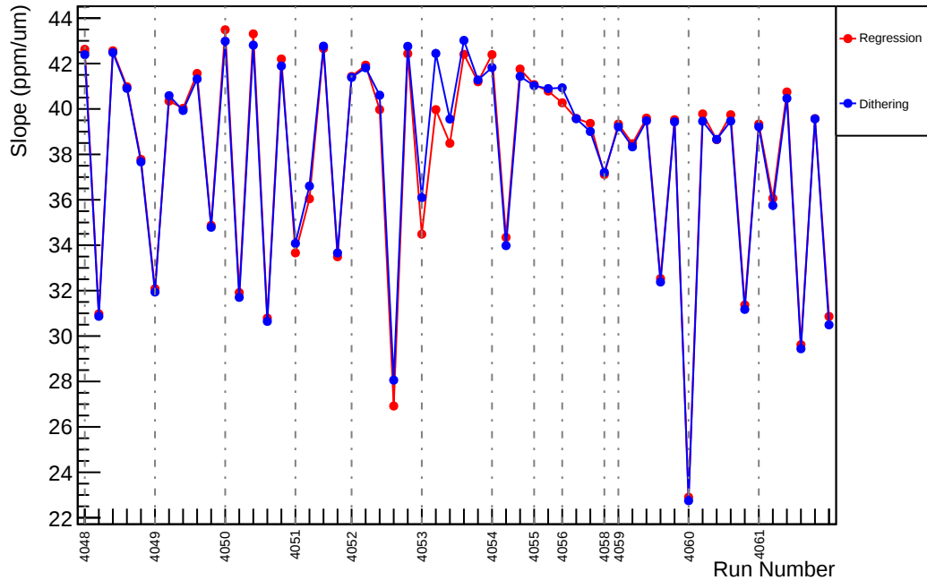
Slug42: Slope : us_dd_vs_evMon0 (ppm/um)
