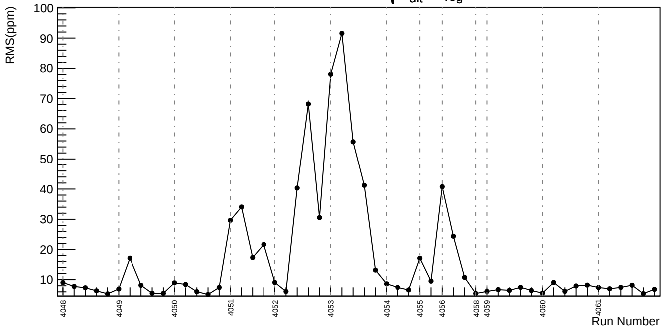
Slug42: asym_us_dd: \sqrt{\sigma_{\text{dit}}^2 - \sigma_{\text{reg}}^2} (ppm)
