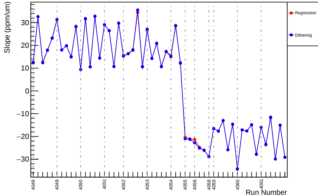
Slug42: Slope : us_dd_vs_evMon1 (ppm/um)
