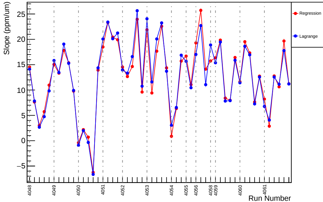
Slug42: Slope : usl_vs_evMon11 (ppm/um)
