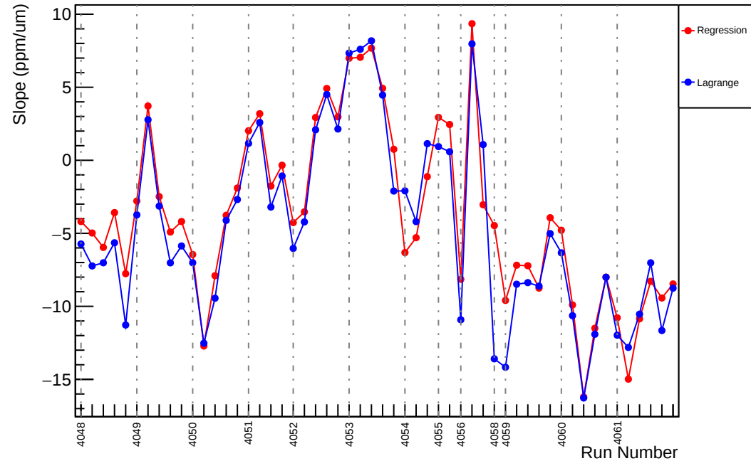
Slug42: Slope : usl_vs_evMon8 (ppm/um)
