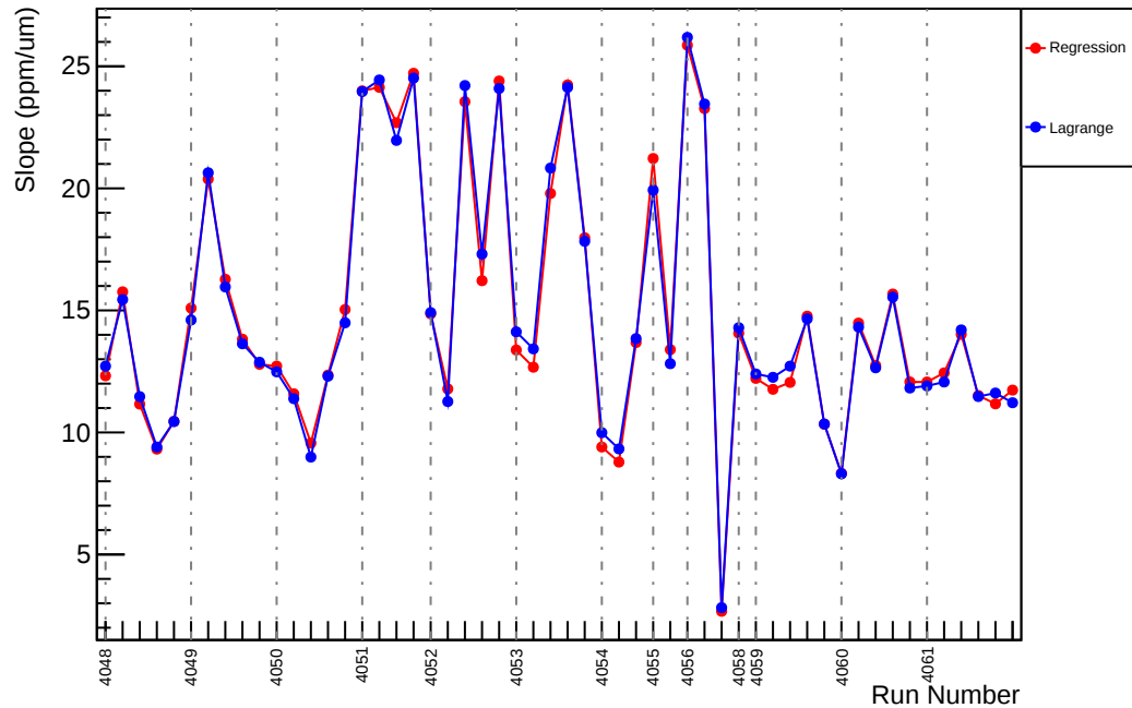
Slug42: Slope : usl_vs_evMon6 (ppm/um)
