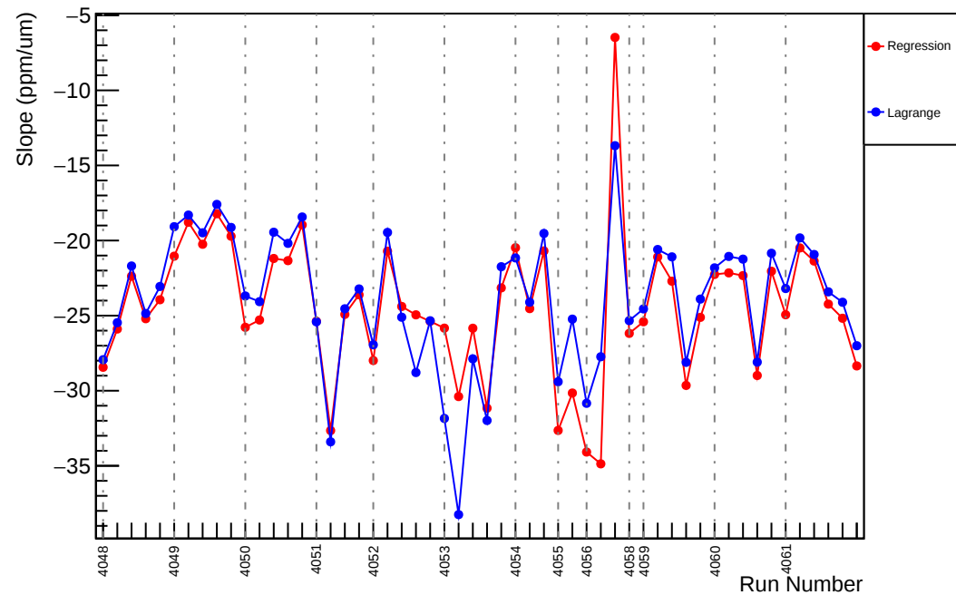
Slug42: Slope : usr_vs_evMon5 (ppm/um)
