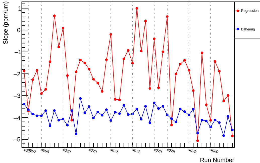
Slug43: Slope : us_dd_vs_evMon4 (ppm/um)
