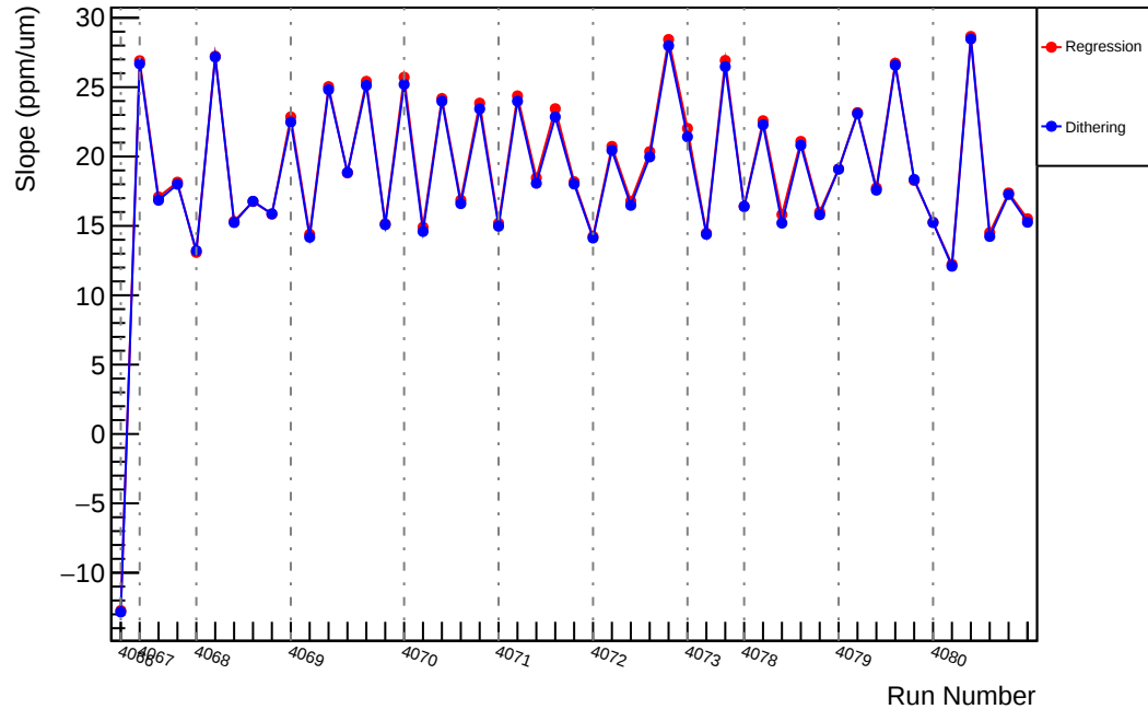
Slug43: Slope : us_dd_vs_evMon1 (ppm/um)
