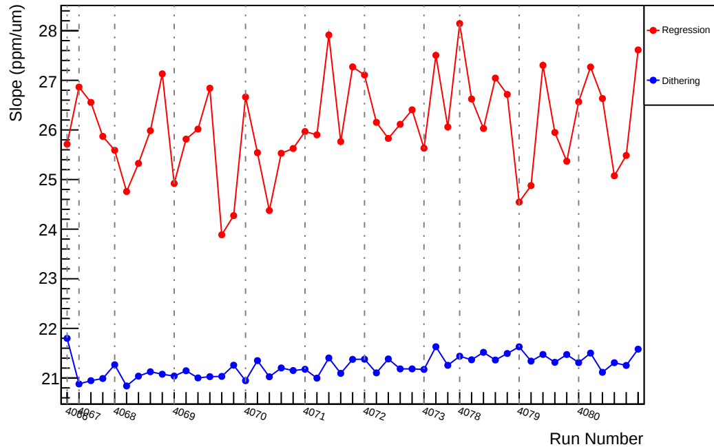
Slug43: Slope : us_dd_vs_evMon3 (ppm/um)
