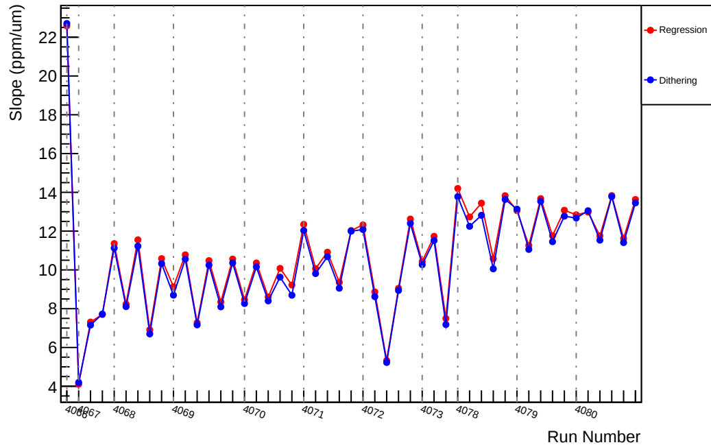
Slug43: Slope : us_dd_vs_evMon2 (ppm/um)
