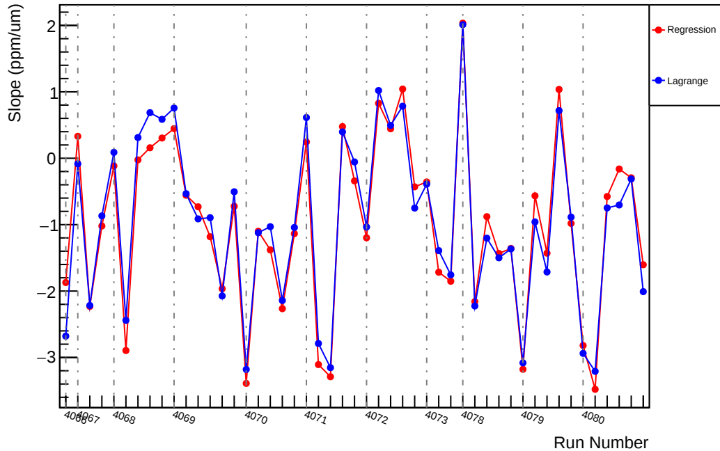
Slug43: Slope : us_dd_vs_evMon6 (ppm/um)
