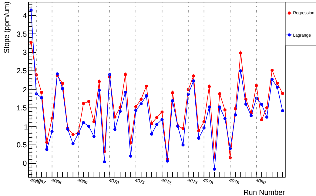
Slug43: Slope : us_dd_vs_evMon5 (ppm/um)
