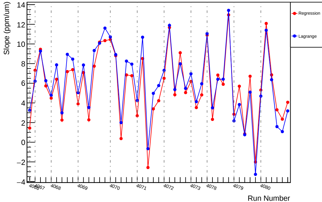
Slug43: Slope : us_dd_vs_evMon10 (ppm/um)
