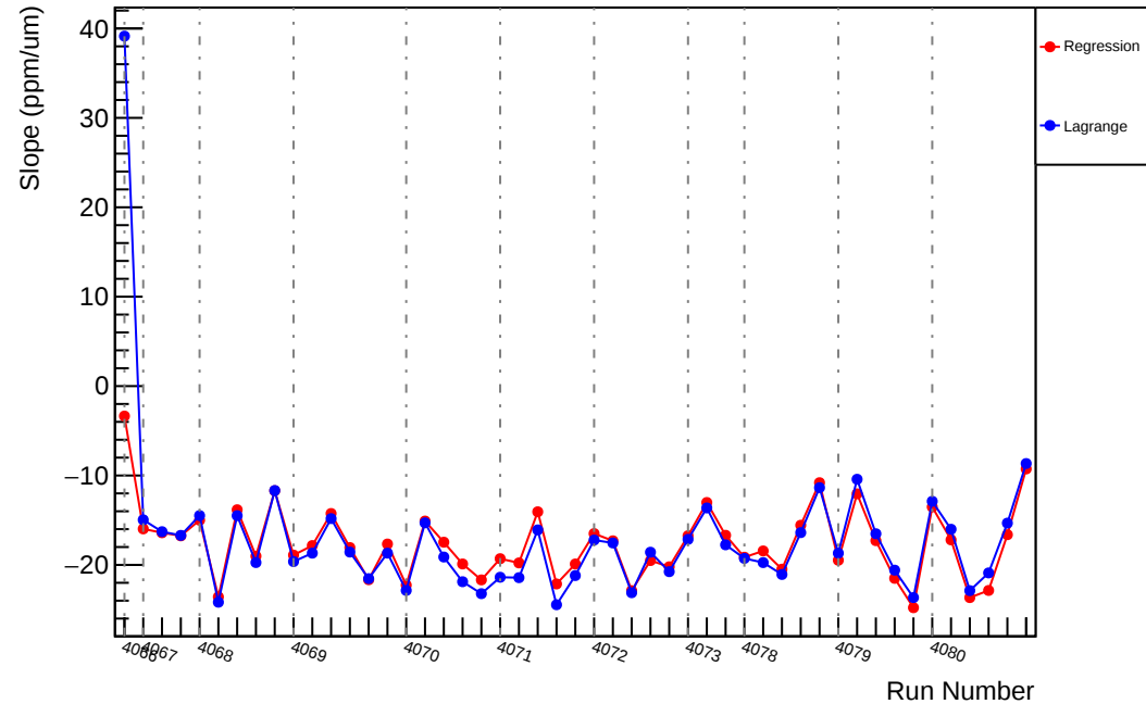
Slug43: Slope : us_dd_vs_evMon11 (ppm/um)
