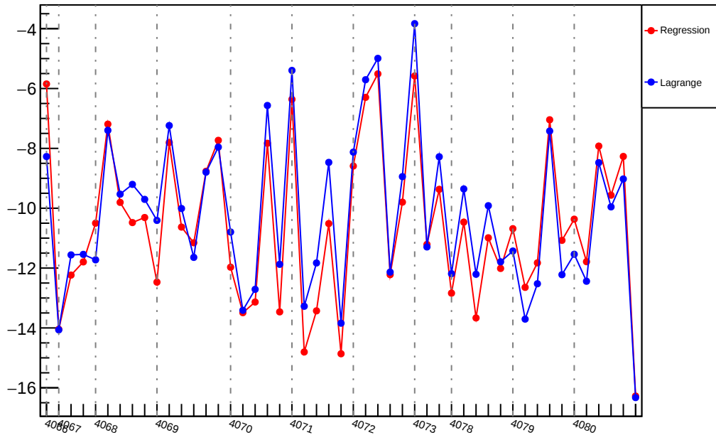
Slug43: Slope : us_dd_vs_evMon9 (ppm/um)
