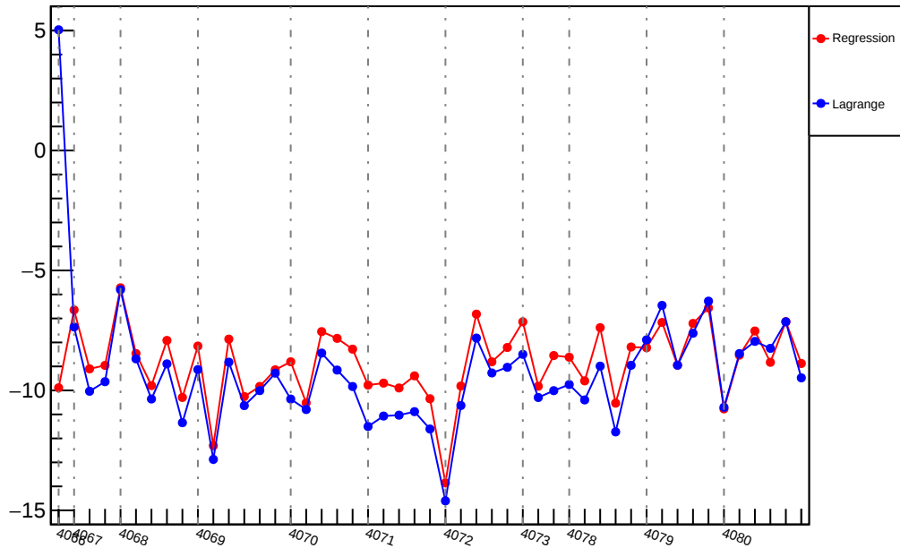
Slug43: Slope : us_dd_vs_evMon7 (ppm/um)
