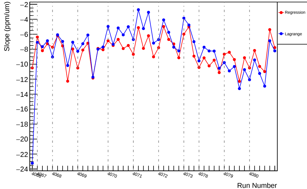
Slug43: Slope : us_dd_vs_evMon8 (ppm/um)
