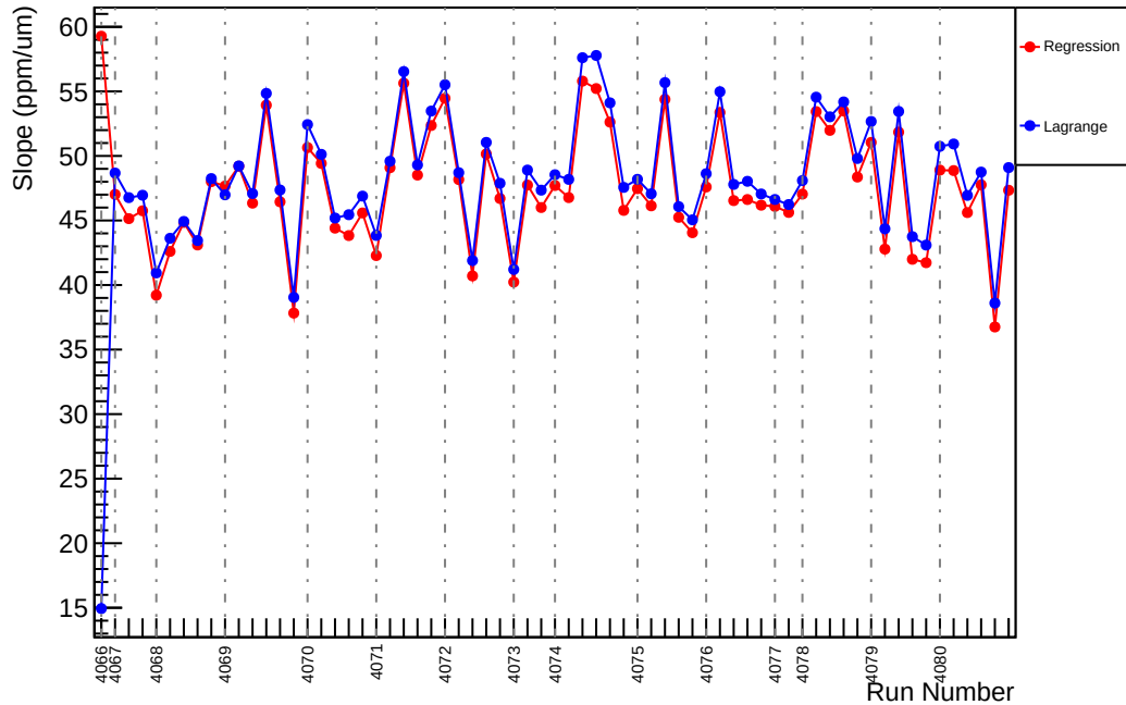
Slug43: Slope : usl_vs_evMon5 (ppm/um)
