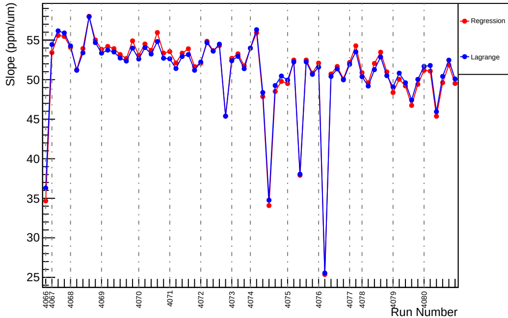
Slug43: Slope : usl_vs_evMon0 (ppm/um)
