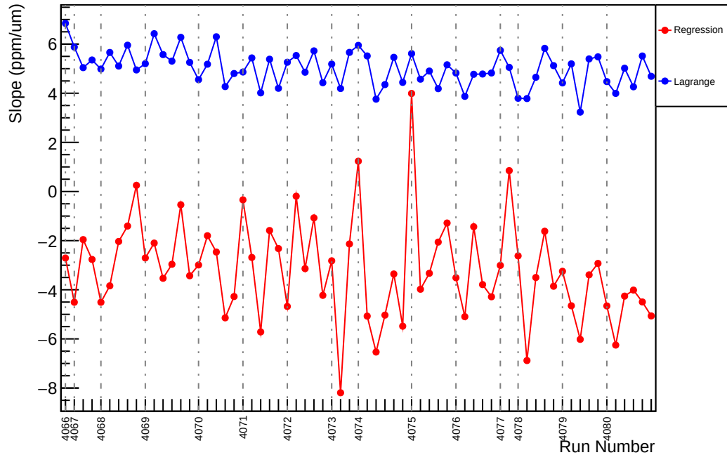
Slug43: Slope : usl_vs_evMon4 (ppm/um)
