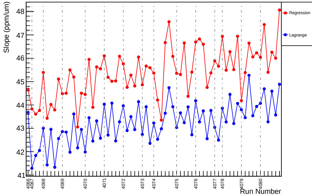
Slug43: Slope : usl_vs_evMon3 (ppm/um)
