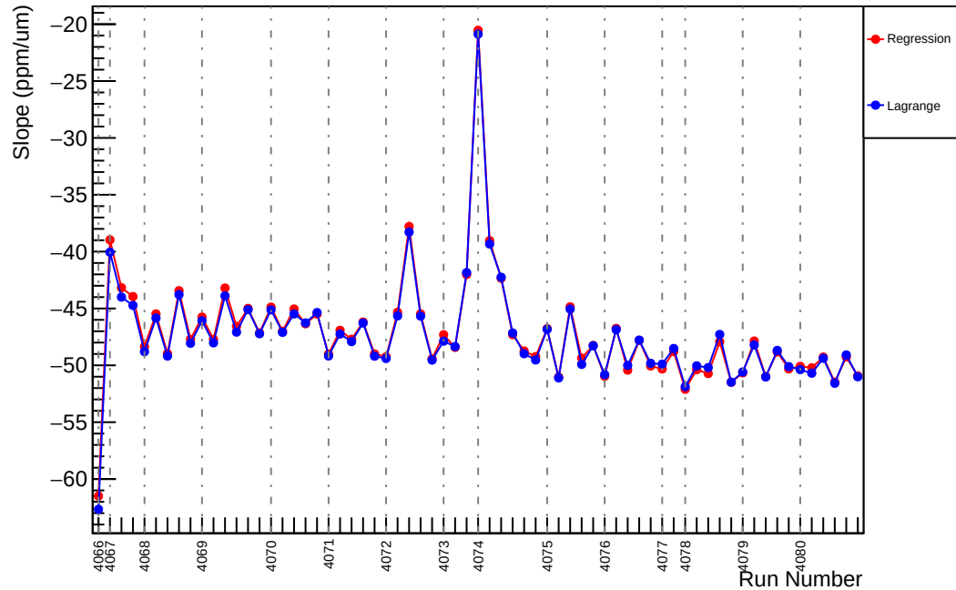
Slug43: Slope : usl_vs_evMon2 (ppm/um)
