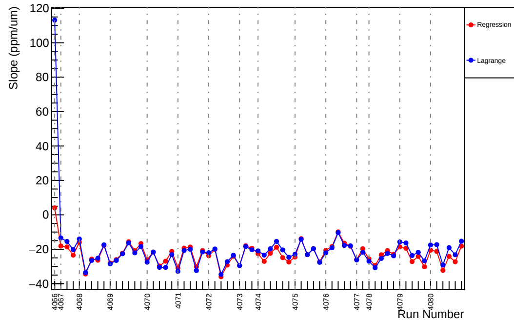
Slug43: Slope : usl_vs_evMon11 (ppm/um)
