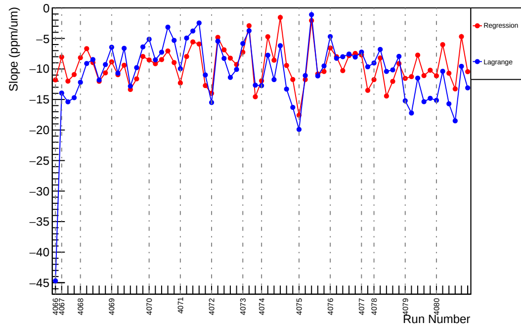
Slug43: Slope : usl_vs_evMon8 (ppm/um)
