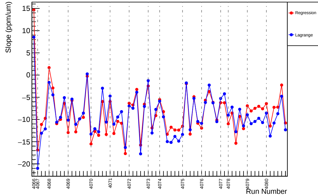
Slug43: Slope : usl_vs_evMon9 (ppm/um)
