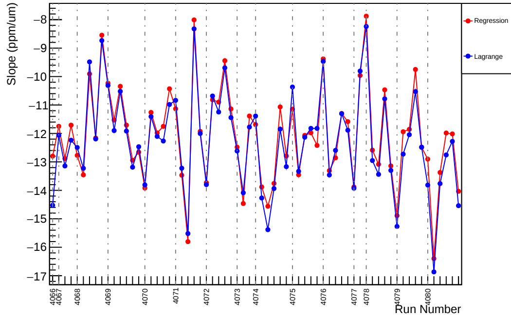
Slug43: Slope : usl_vs_evMon6 (ppm/um)
