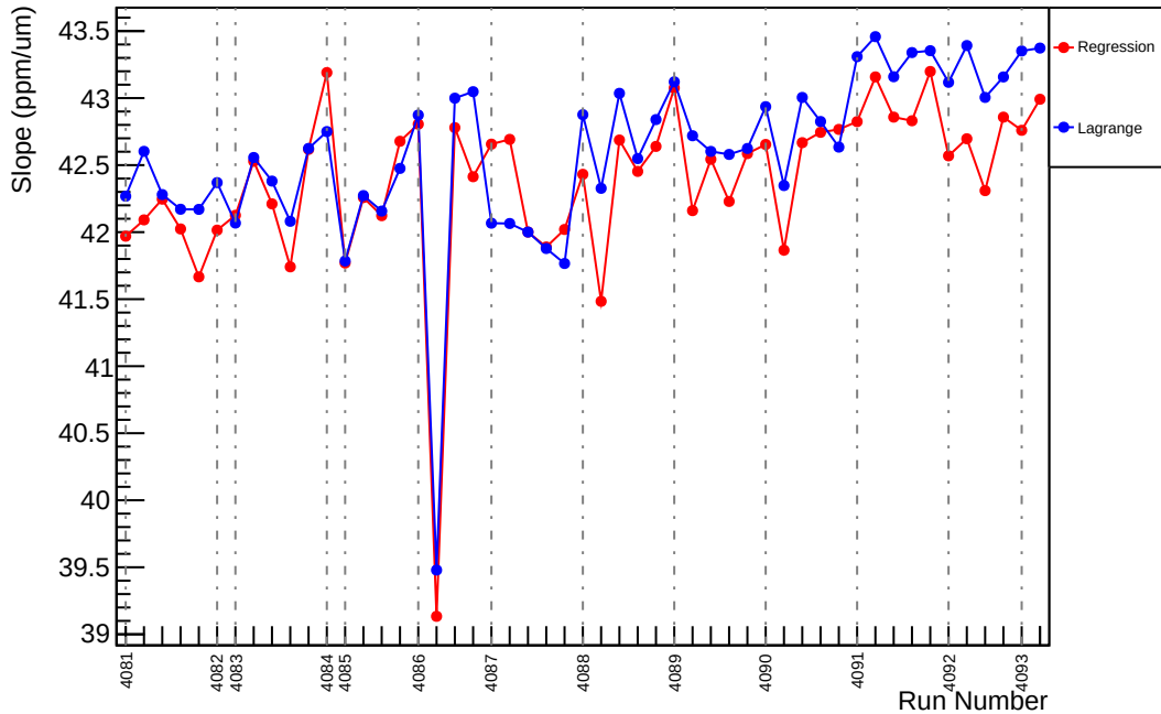
Slug44: Slope : us_avg_vs_evMon2 (ppm/um)
