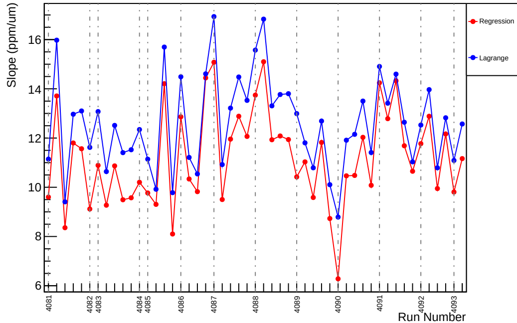
Slug44: Slope : us_avg_vs_evMon5 (ppm/um)
