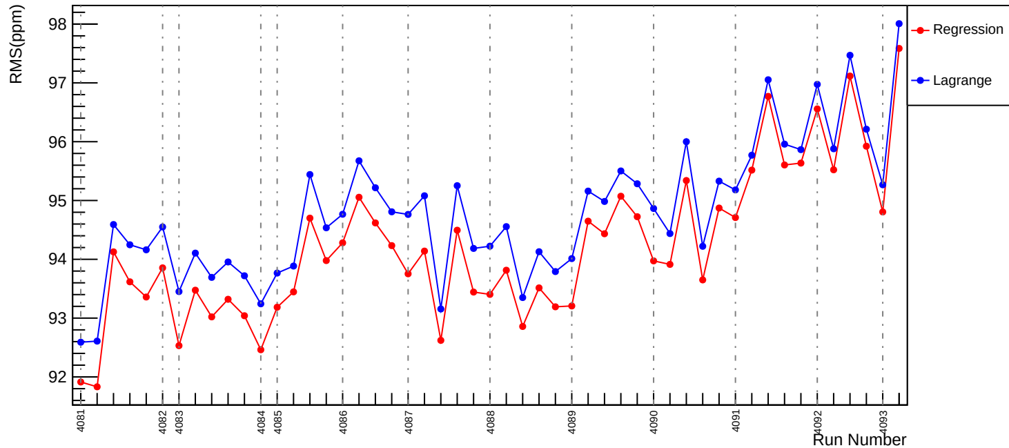
Slug44: Corrected RMS (ppm): asym_us_avg
