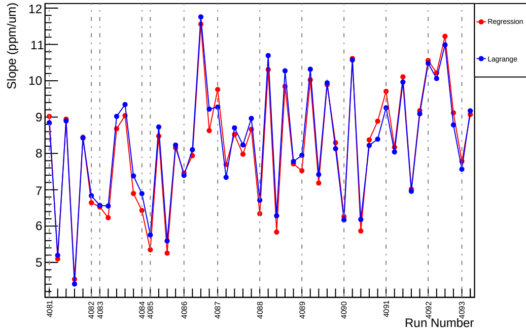
Slug44: Slope : us_avg_vs_evMon0 (ppm/um)
