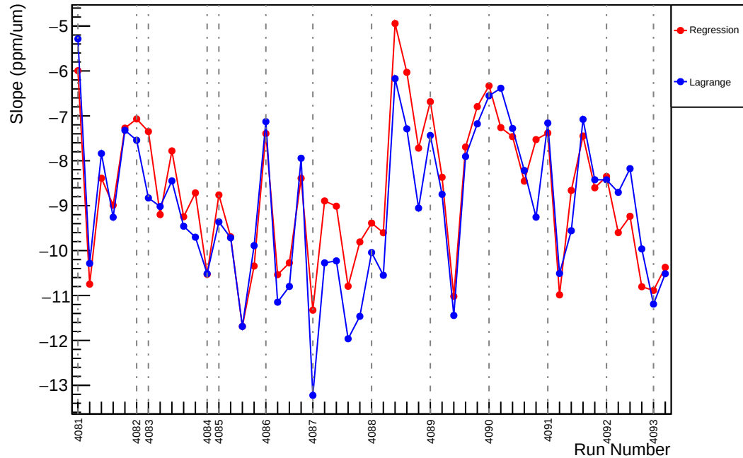
Slug44: Slope : us_dd_vs_evMon7 (ppm/um)
