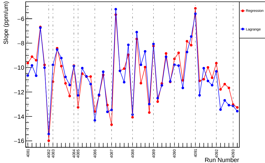
Slug44: Slope : us_dd_vs_evMon9 (ppm/um)
