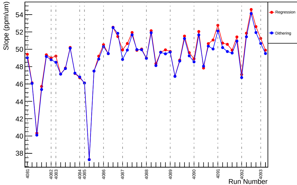
Slug44: Slope : usl_vs_evMon0 (ppm/um)
