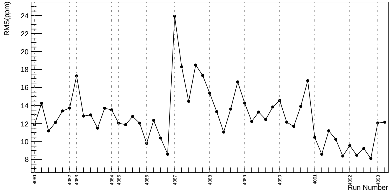
Slug44: asym_usl: \sqrt{\sigma_{\text{dit}}^2 - \sigma_{\text{reg}}^2} (ppm)
