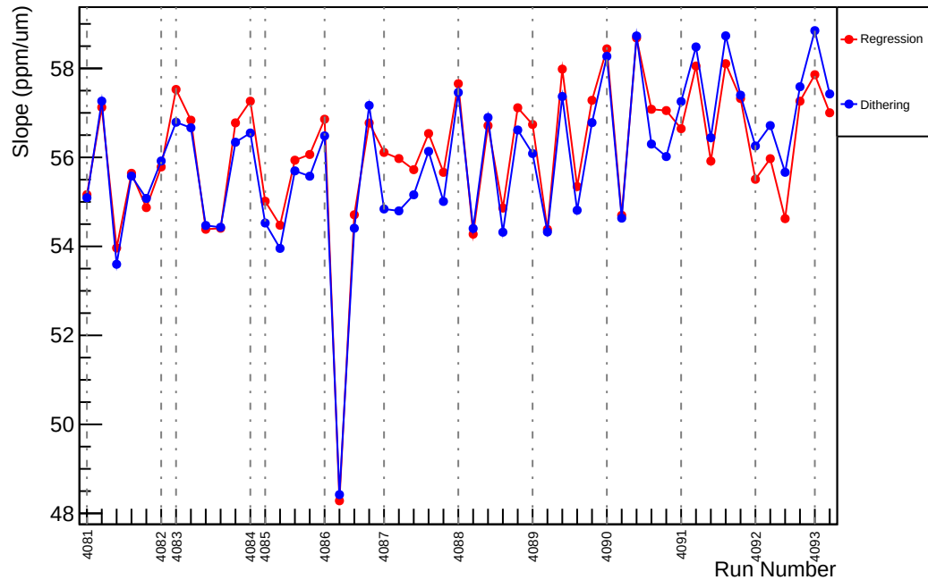
Slug44: Slope : usl_evMon2 (ppm/um)
