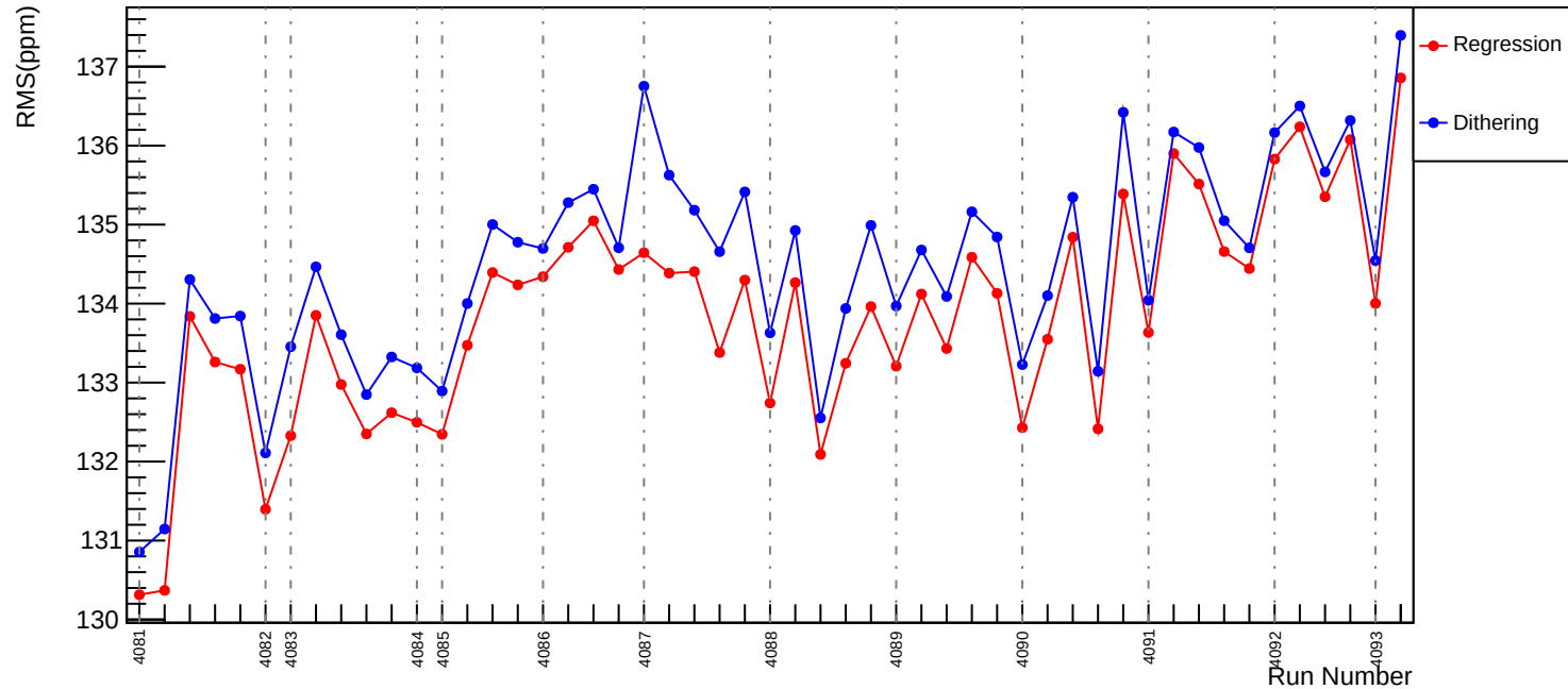
Slug44: Corrected RMS (ppm): asym_usl
