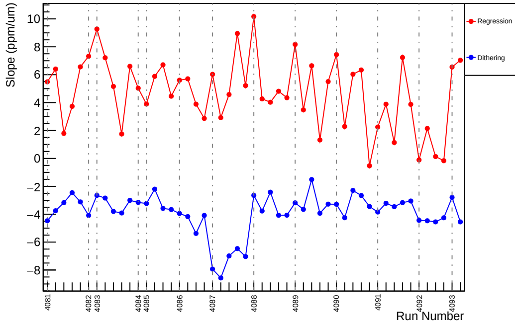
Slug44: Slope : usl_vs_evMon4 (ppm/um)
