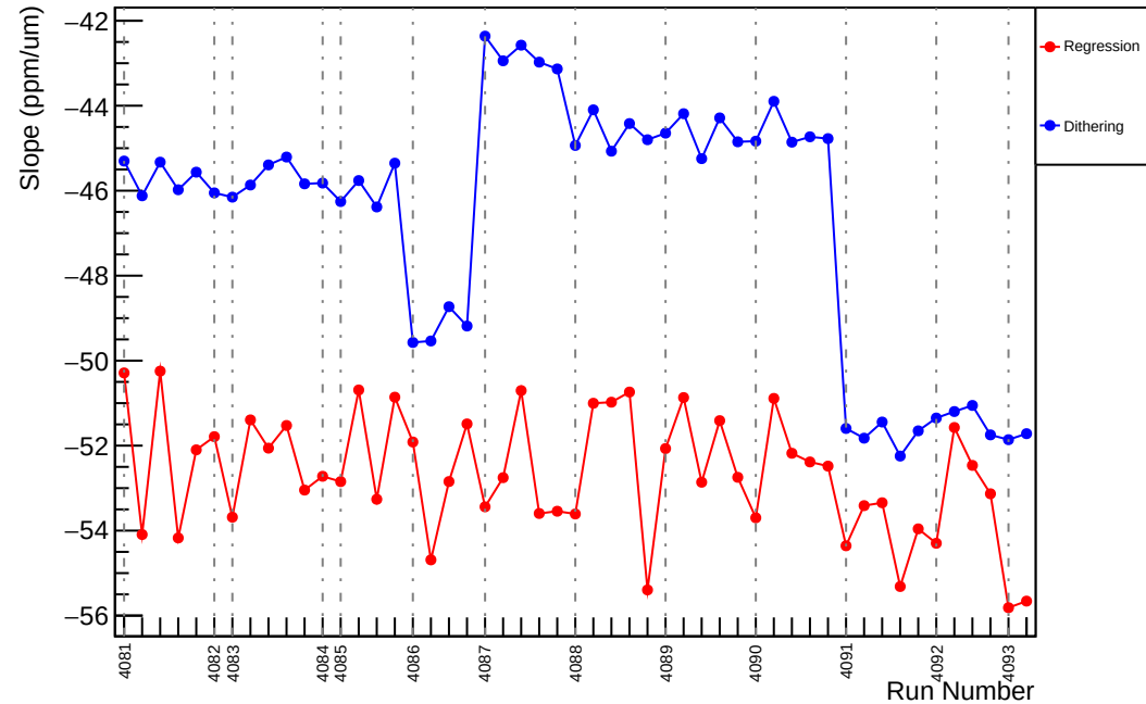
Slug44: Slope : usl_vs_evMon3 (ppm/um)
