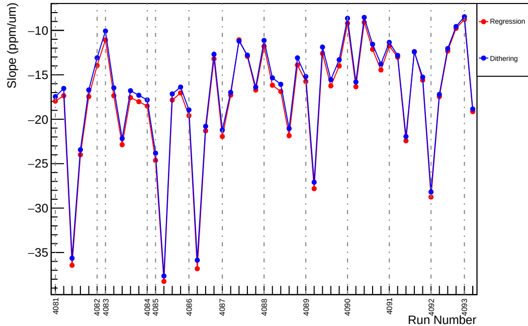
Slug44: Slope : usl_vs_evMon1 (ppm/um)
