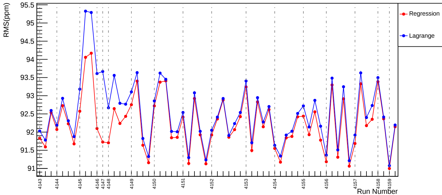
Slug45: Corrected RMS (ppm): asym_us_dd
