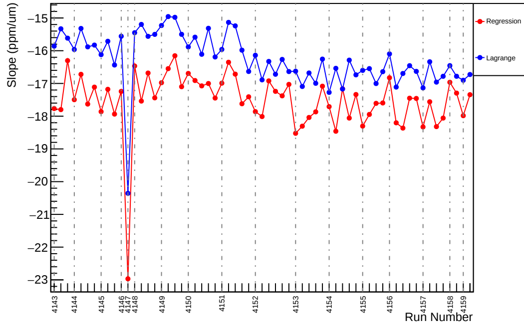
Slug45: Slope : us_dd_vs_evMon3 (ppm/um)
