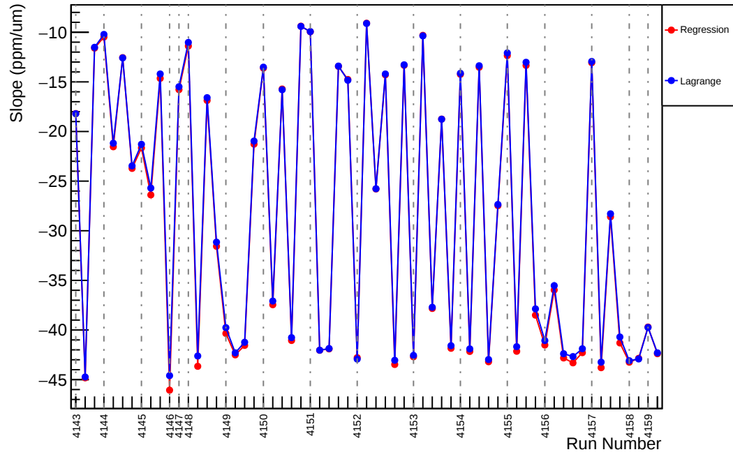
Slug45: Slope : us_dd_vs_evMon1 (ppm/um)
