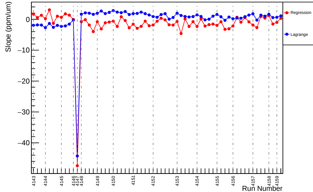
Slug45: Slope : us_dd_vs_evMon4 (ppm/um)
