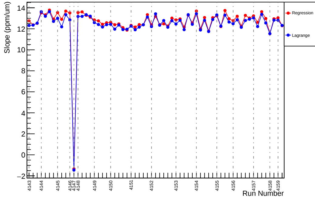
Slug45: Slope : us_dd_vs_evMon2 (ppm/um)
