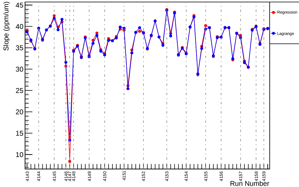
Slug45: Slope : us_dd_vs_evMon5 (ppm/um)
