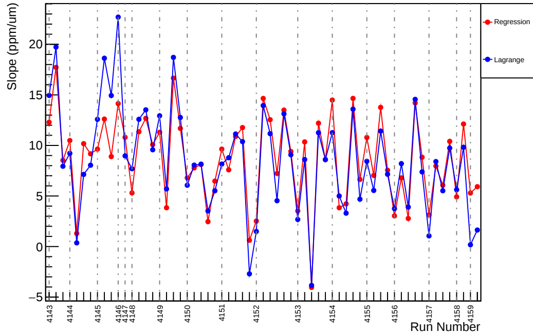
Slug45: Slope : usl_vs_evMon11 (ppm/um)
