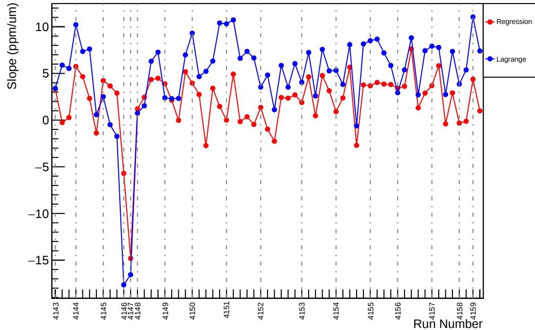
Slug45: Slope : usl_vs_evMon8 (ppm/um)
