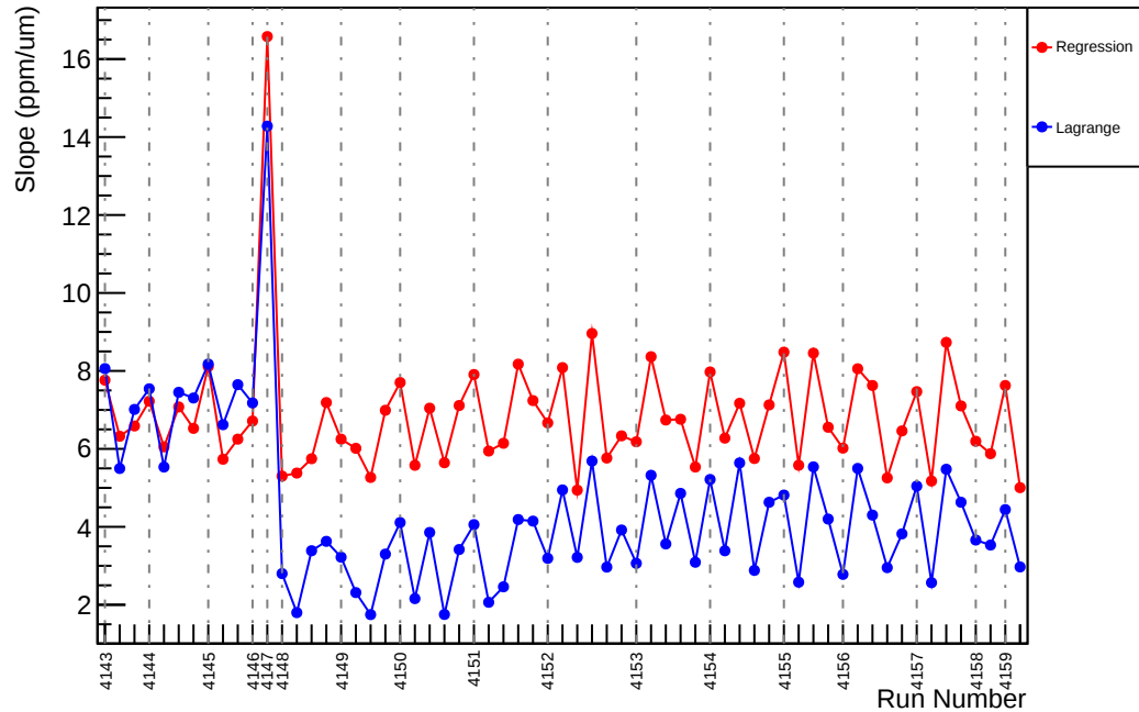
Slug45: Slope : usl_vs_evMon4 (ppm/um)
