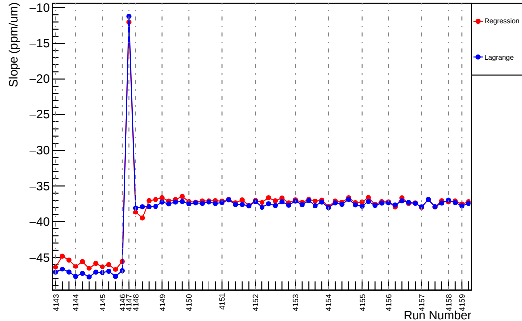
Slug45: Slope : usl_vs_evMon2 (ppm/um)
