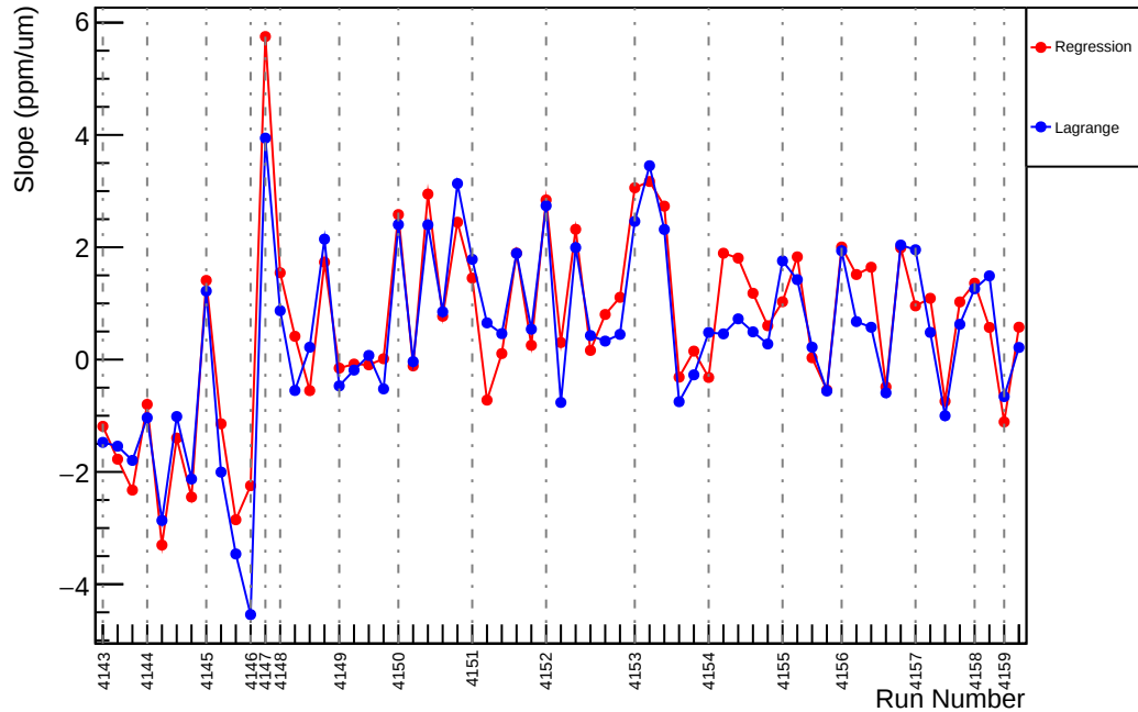
Slug45: Slope : usl_vs_evMon5 (ppm/um)
