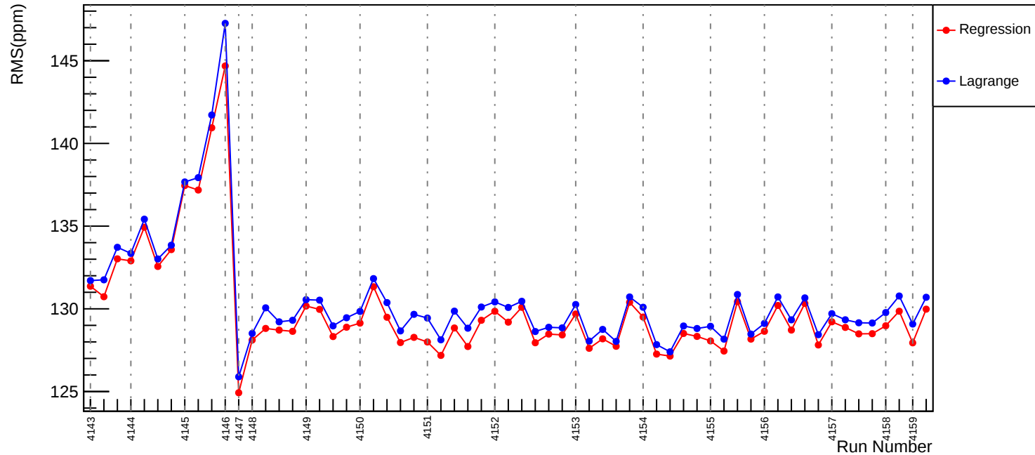
Slug45: Corrected RMS (ppm): asym_usl
