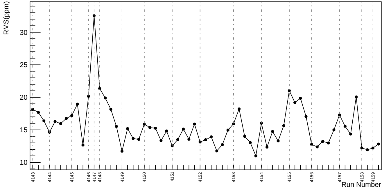
Slug45: asym_usr: \sqrt{\sigma_{\text{dit}}^2 - \sigma_{\text{reg}}^2} (ppm)
