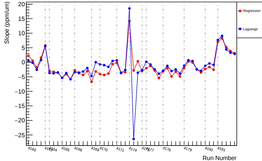
Slug46: Slope : us_avg_vs_evMon7 (ppm/um)
