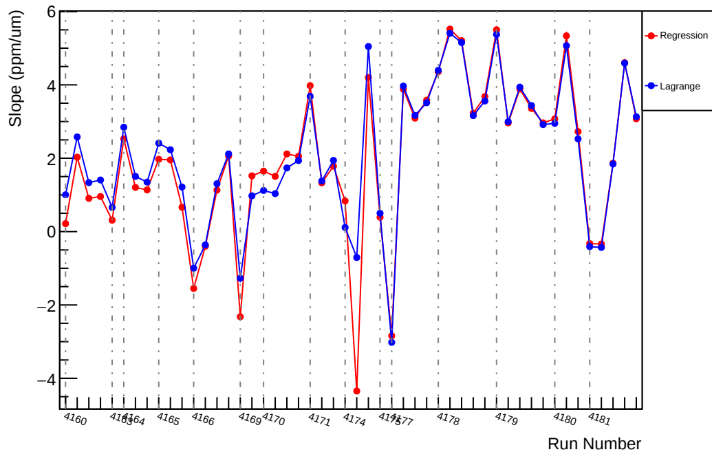
Slug46: Slope : us_avg_vs_evMon0 (ppm/um)
