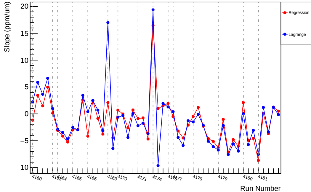
Slug46: Slope : us_avg_vs_evMon10 (ppm/um)
