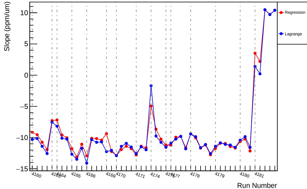
Slug46: Slope : us_avg_vs_evMon6 (ppm/um)
