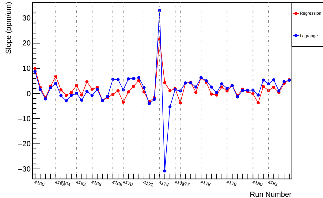
Slug46: Slope : us_avg_vs_evMon9 (ppm/um)
