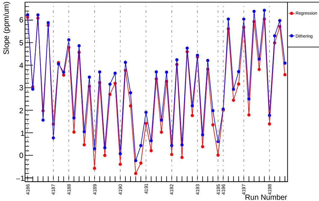
Slug47: Slope : us_avg_vs_evMon0 (ppm/um)
