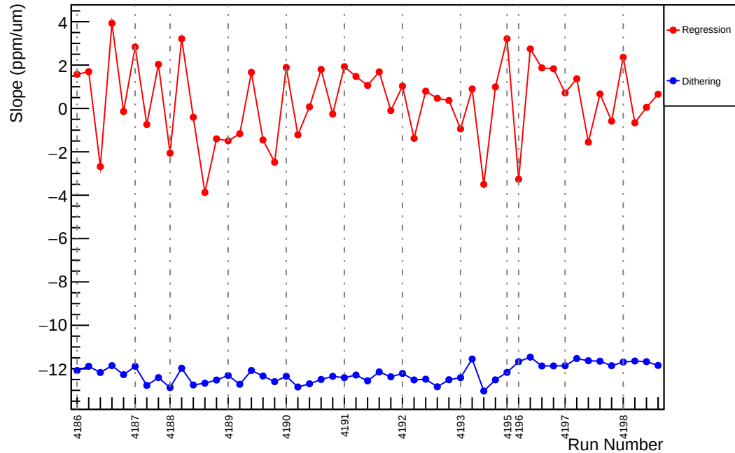
Slug47: Slope : us_avg_vs_evMon4 (ppm/um)
