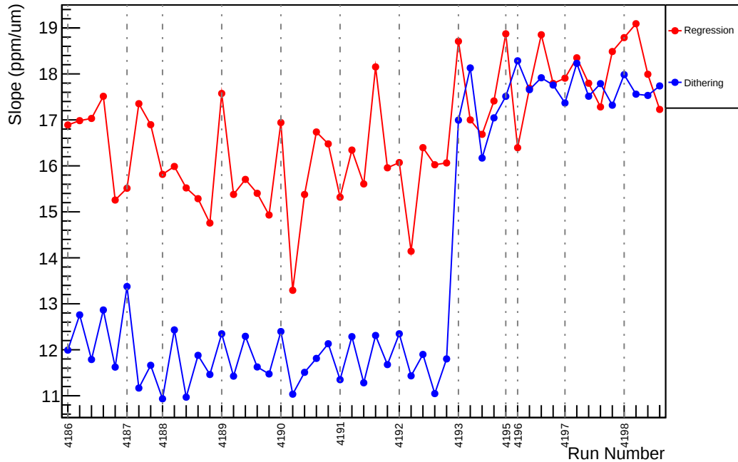
Slug47: Slope : us_avg_vs_evMon3 (ppm/um)
