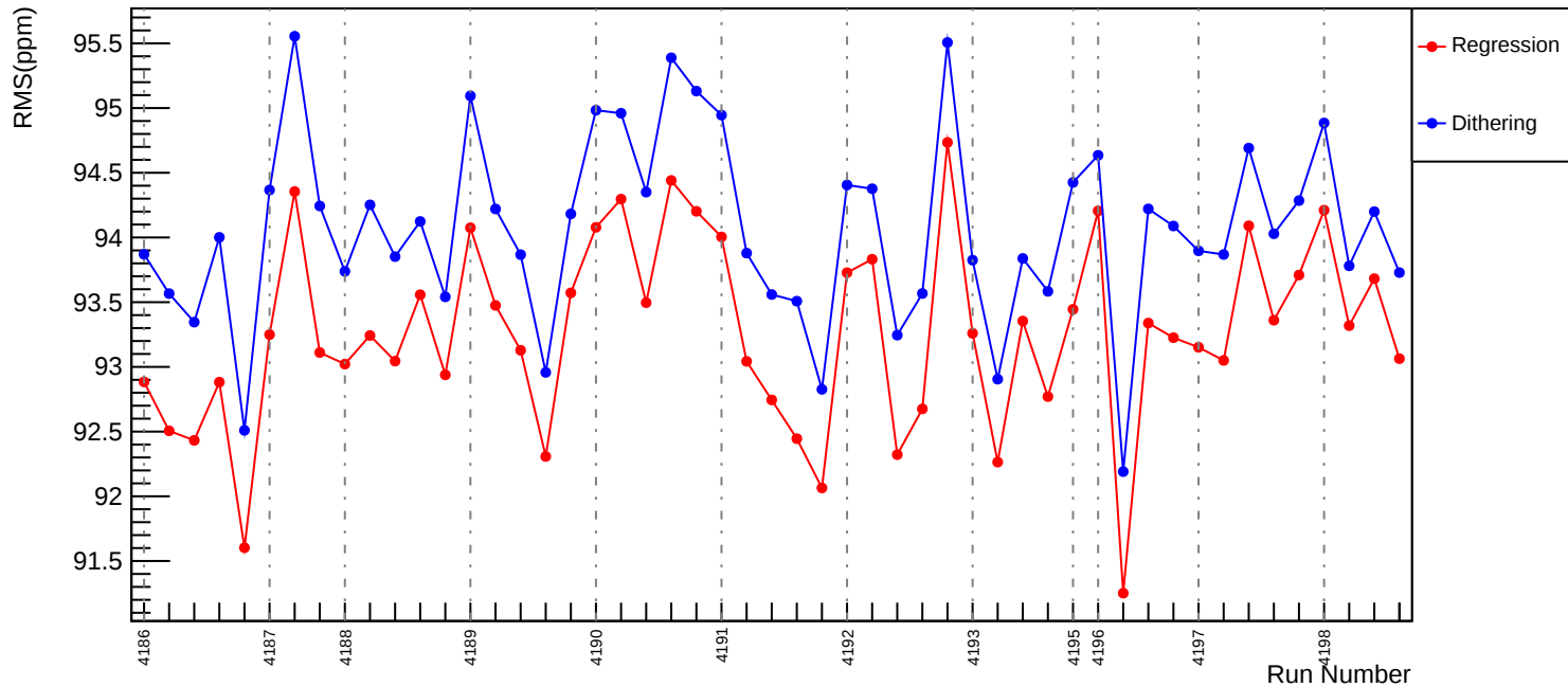
Slug47: Corrected RMS (ppm): asym_us_avg
