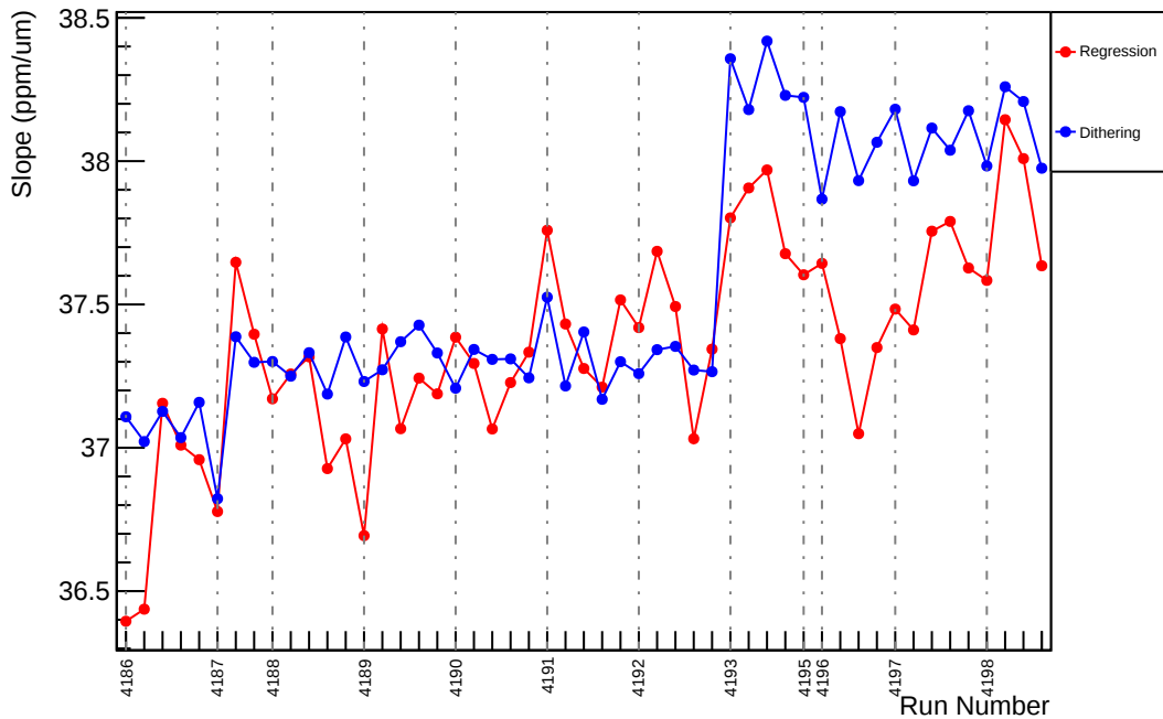
Slug47: Slope : us_avg_vs_evMon2 (ppm/um)
