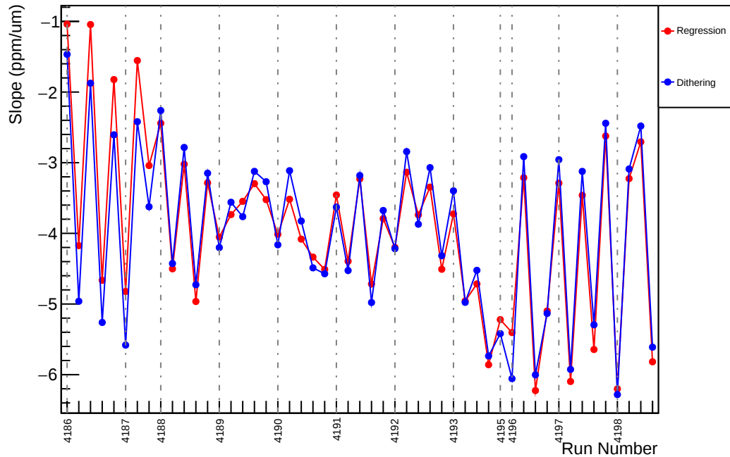
Slug47: Slope : us_avg_vs_evMon1 (ppm/um)
