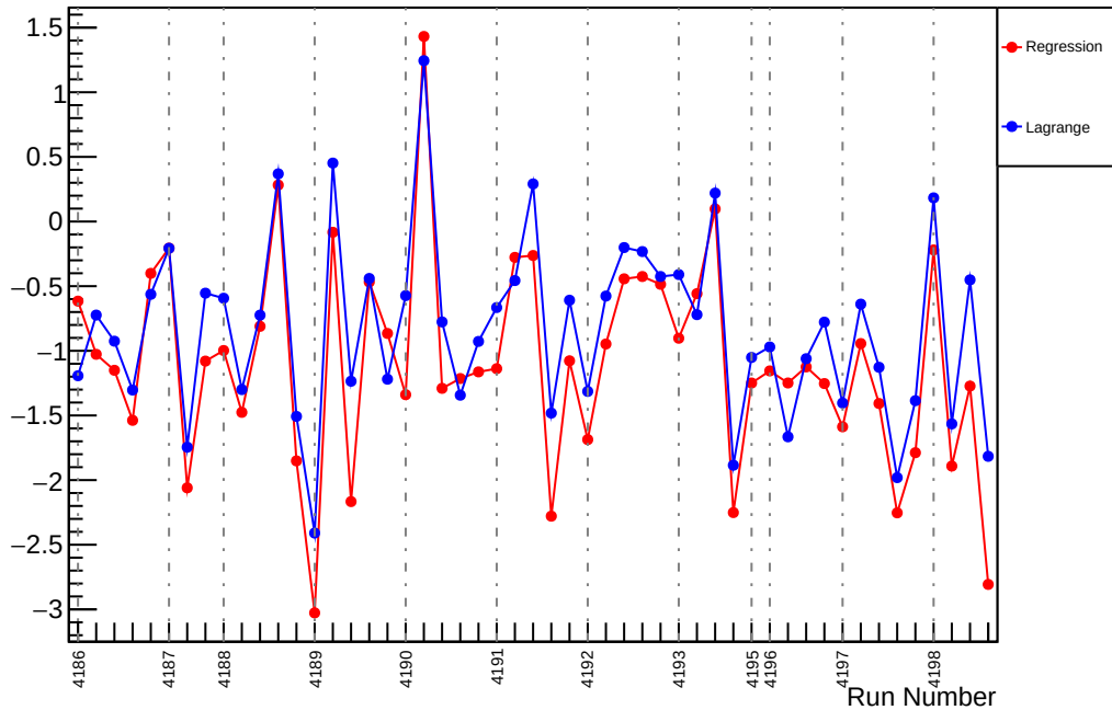
Slug47: Slope : us_dd_vs_evMon5 (ppm/um)
