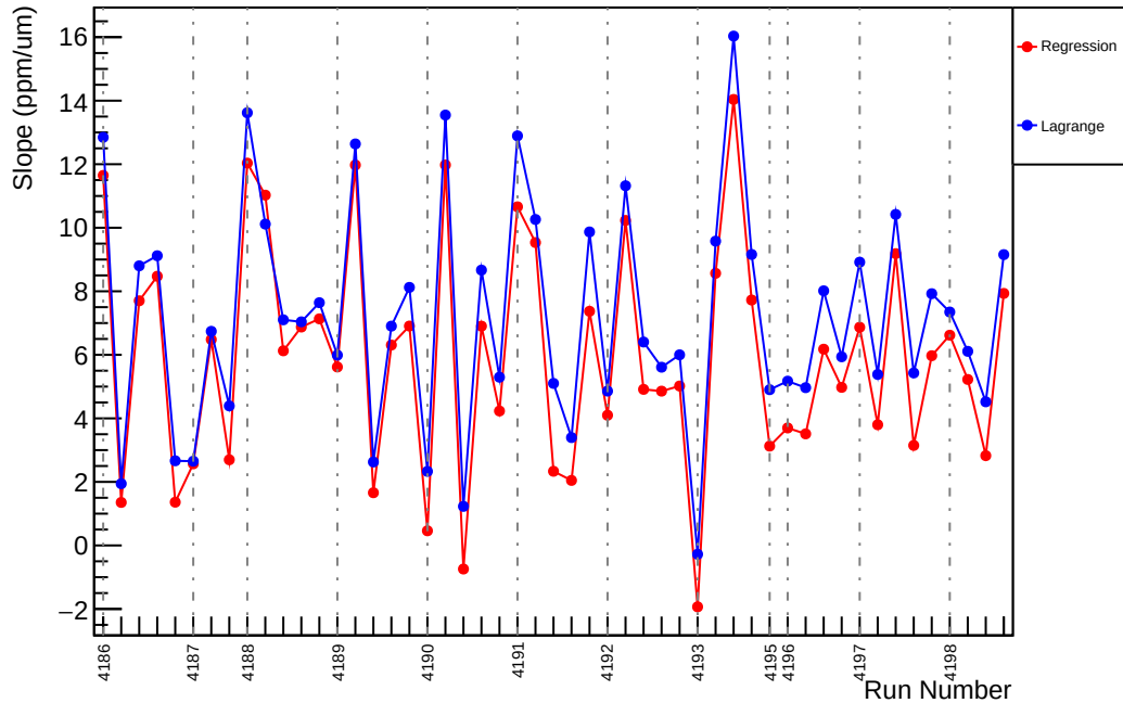
Slug47: Slope : us_dd_vs_evMon11 (ppm/um)
