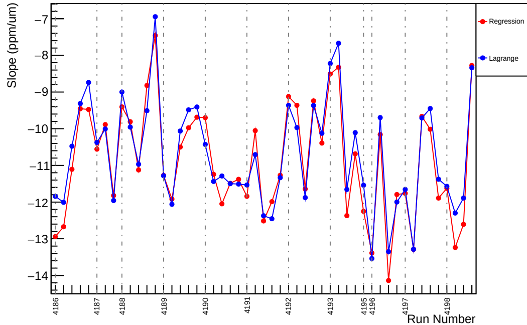
Slug47: Slope : us_dd_vs_evMon7 (ppm/um)
