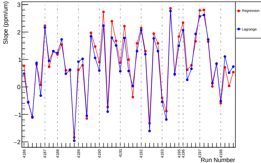
Slug47: Slope : us_dd_vs_evMon6 (ppm/um)
