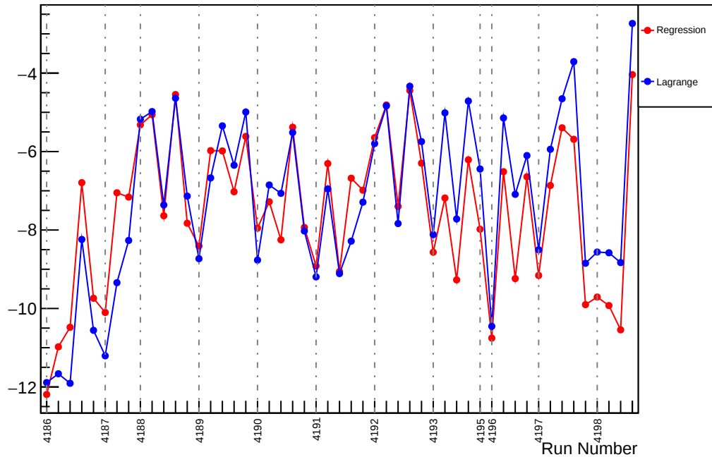
Slug47: Slope : usl_vs_evMon7 (ppm/um)
