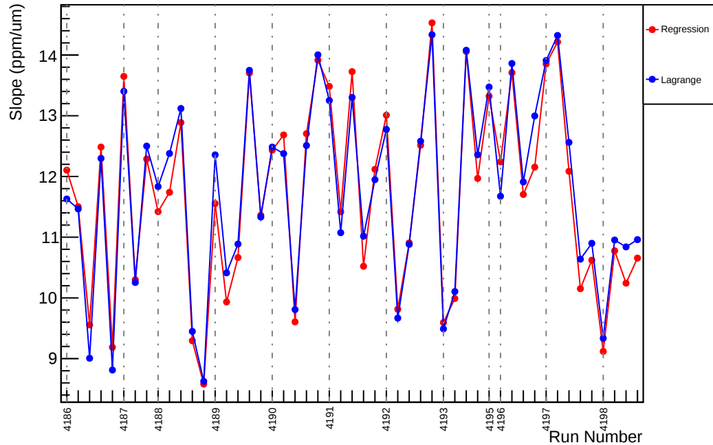
Slug47: Slope : usl_vs_evMon6 (ppm/um)
