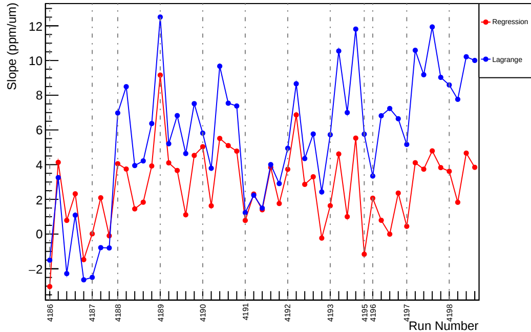
Slug47: Slope : usl_vs_evMon8 (ppm/um)
