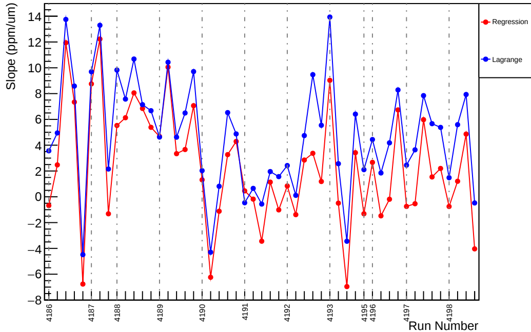
Slug47: Slope : usl_vs_evMon10 (ppm/um)
