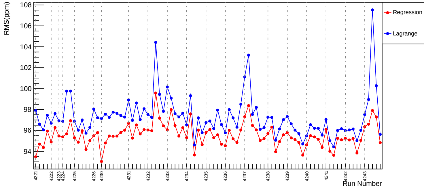
Slug49: Corrected RMS (ppm): asym_us_avg
