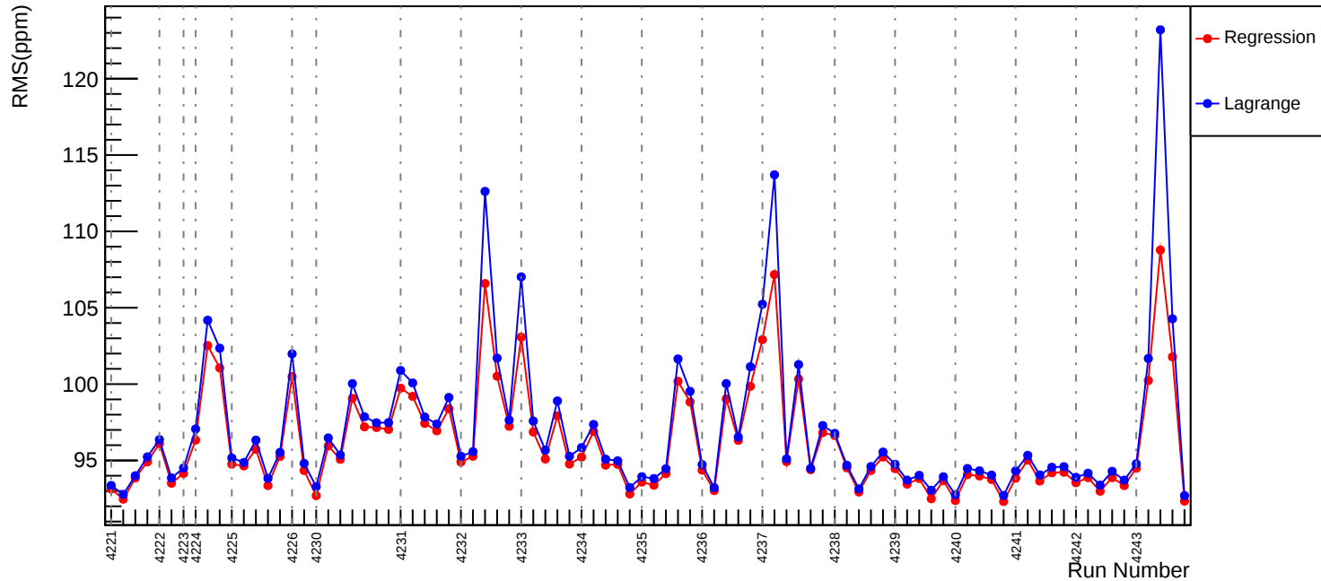
Slug49: Corrected RMS (ppm): asym_us_dd
