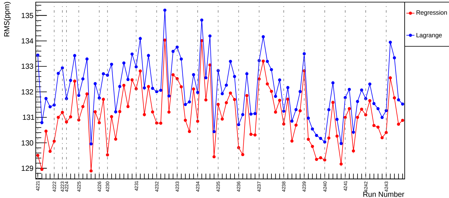
Slug49: Corrected RMS (ppm): asym_usl
