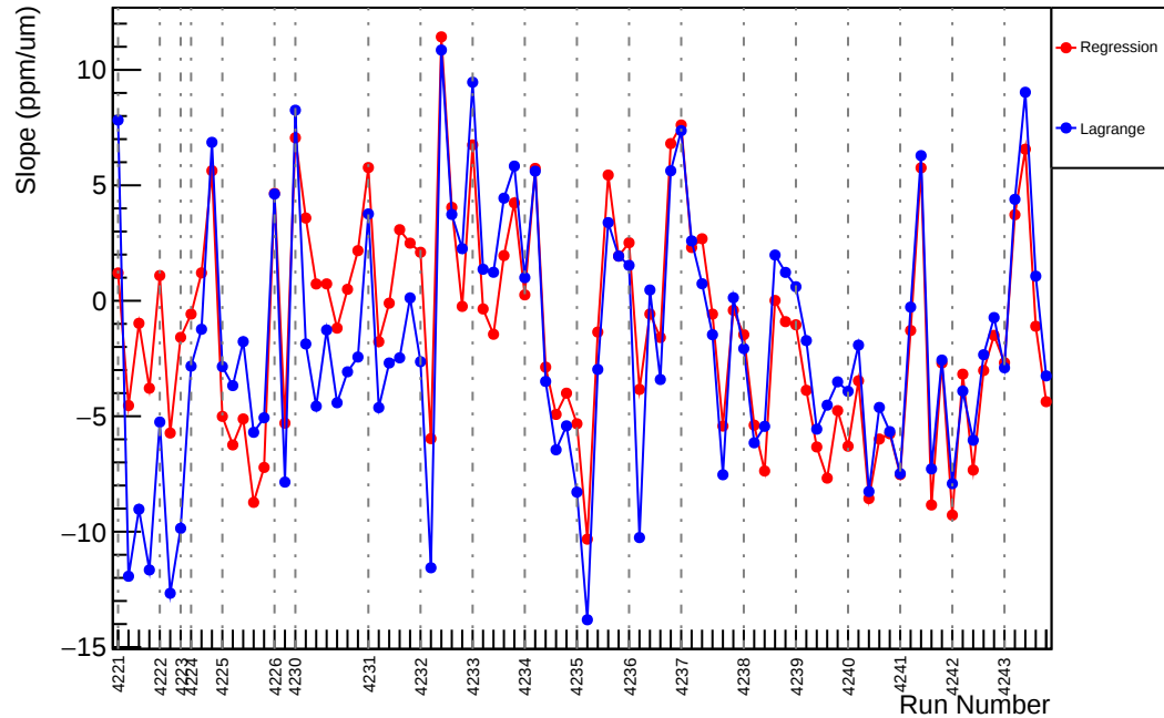
Slug49: Slope : usl_vs_evMon8 (ppm/um)
