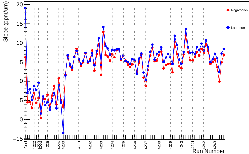
Slug49: Slope : usl_vs_evMon7 (ppm/um)
