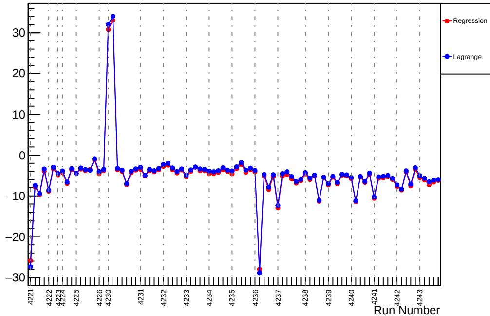
Slug49: Slope : usl_vs_evMon0 (ppm/um)
