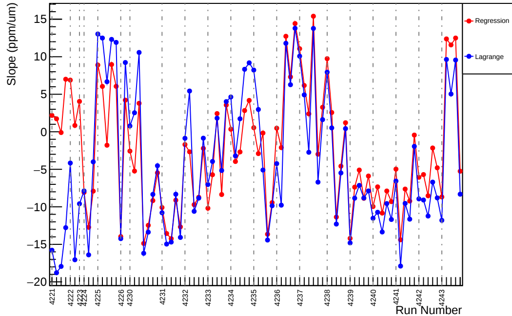
Slug49: Slope : usl_vs_evMon9 (ppm/um)
