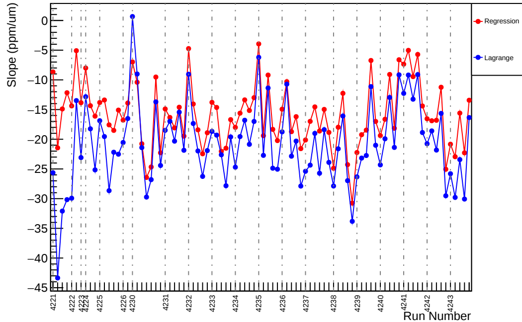
Slug49: Slope : usl_vs_evMon11 (ppm/um)
