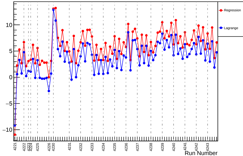
Slug49: Slope : usl_vs_evMon3 (ppm/um)
