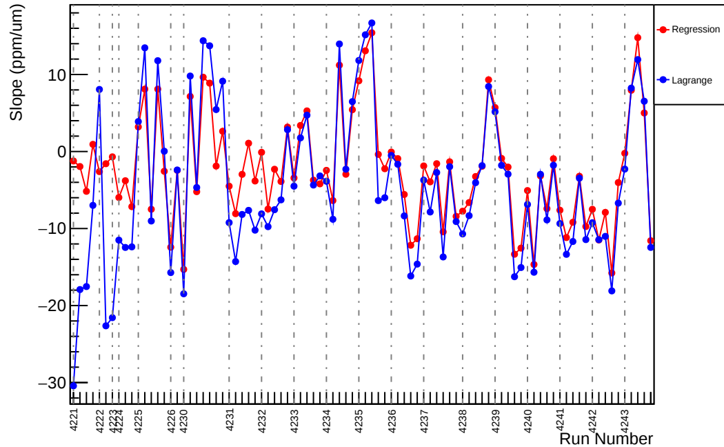
Slug49: Slope : usl_vs_evMon10 (ppm/um)
