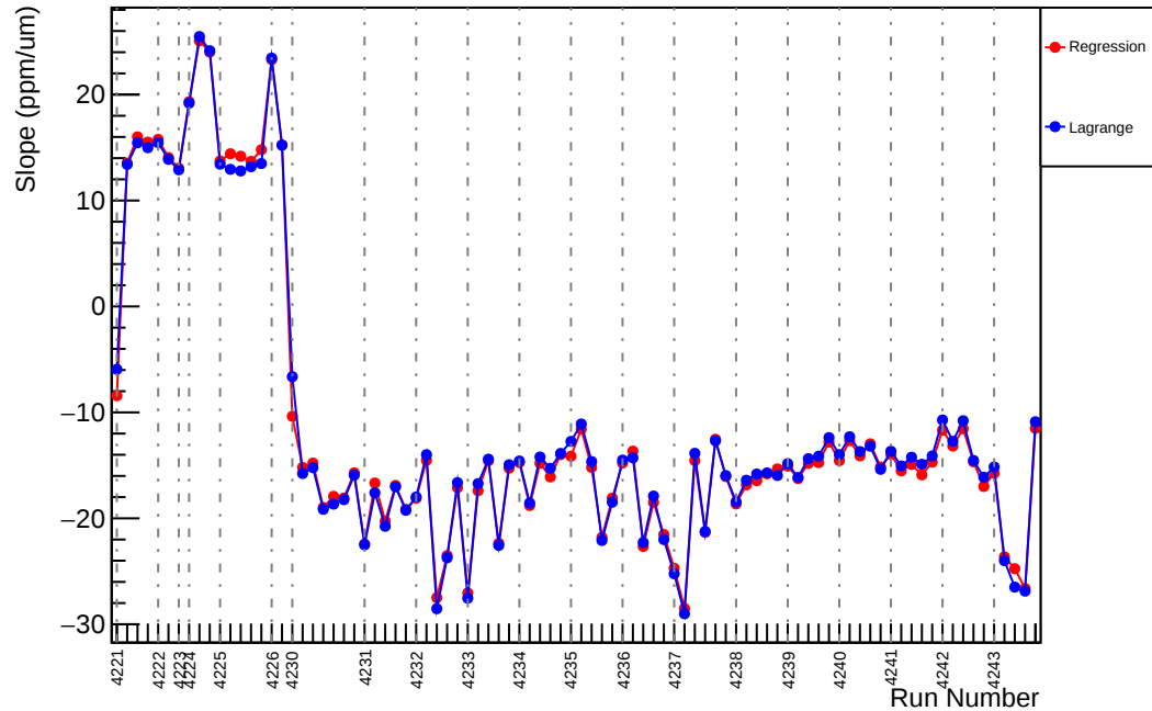
Slug49: Slope : usl_vs_evMon6 (ppm/um)
