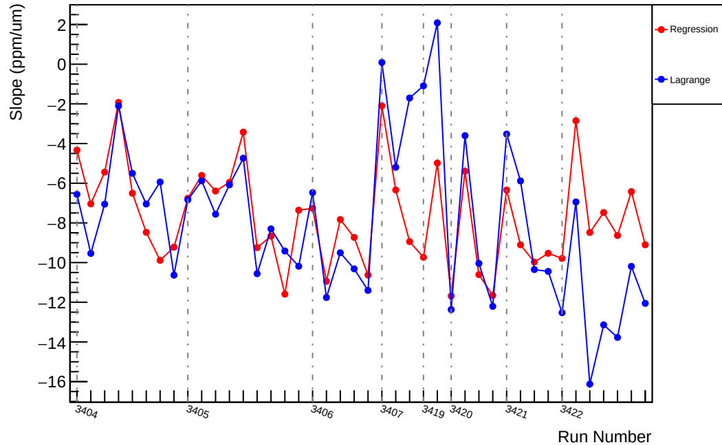
Slug4: Slope : us_avg_vs_evMon9 (ppm/um)
