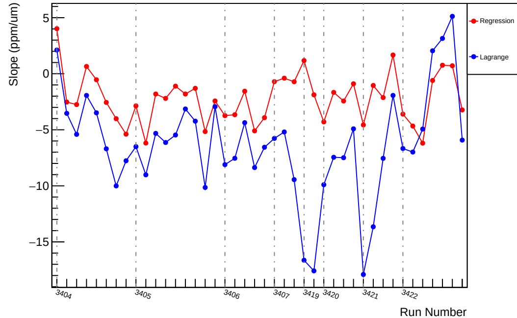
Slug4: Slope : us_avg_vs_evMon8 (ppm/um)
