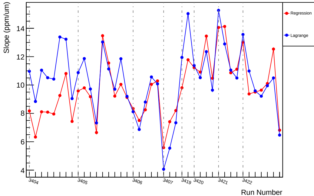
Slug4: Slope : us_avg_vs_evMon7 (ppm/um)
