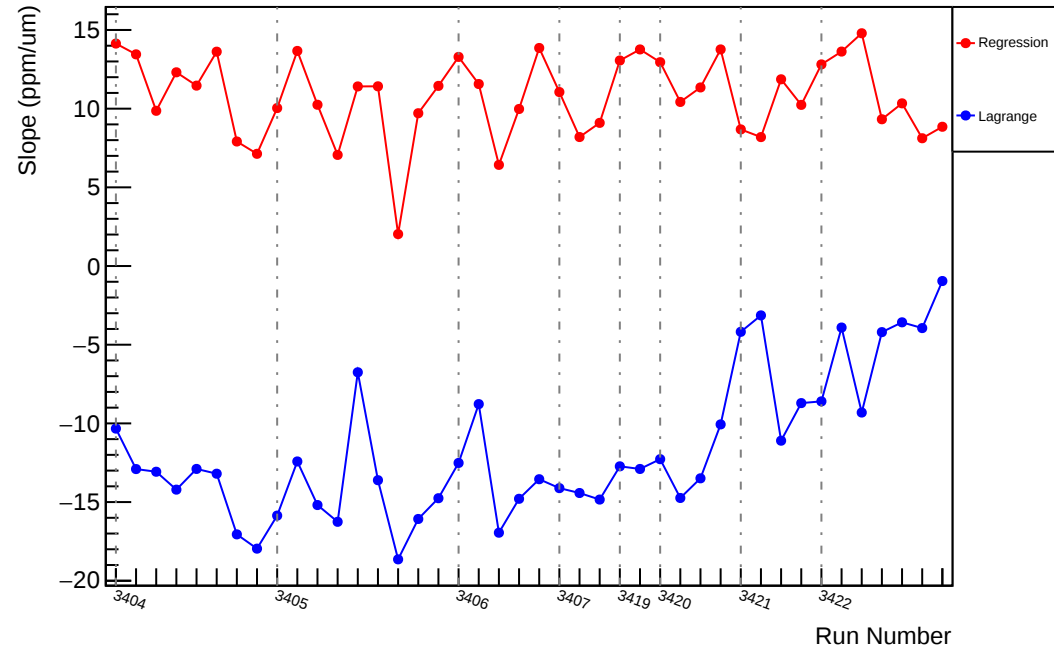
Slug4: Slope : us_dd_vs_evMon3 (ppm/um)
