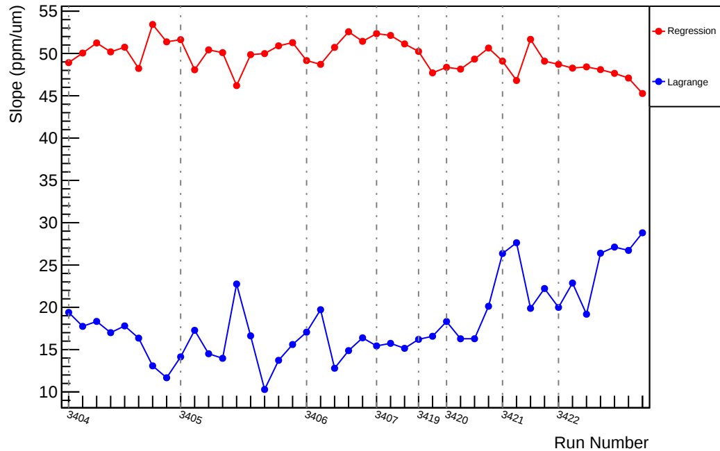
Slug4: Slope : us_dd_vs_evMon4 (ppm/um)
