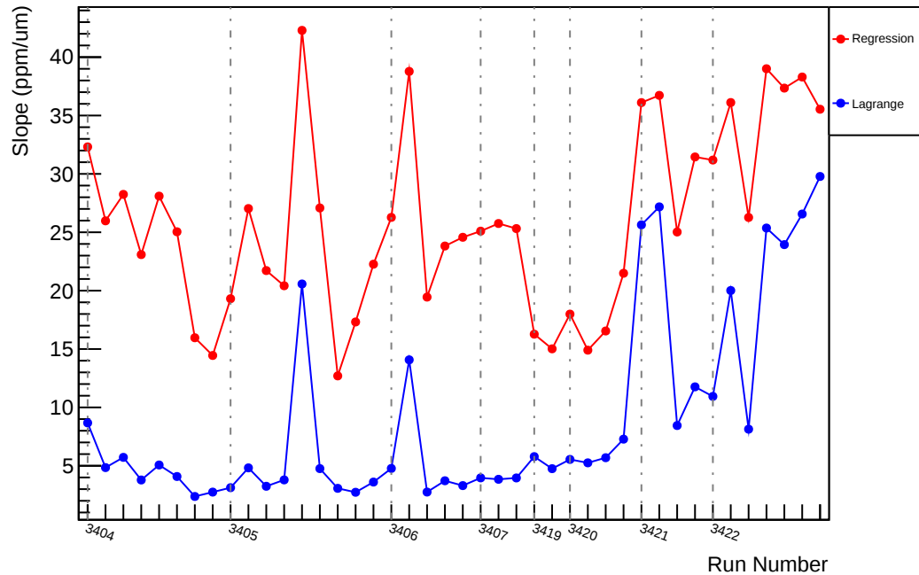
Slug4: Slope : us_dd_vs_evMon2 (ppm/um)
