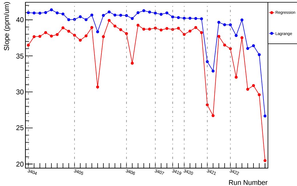
Slug4: Slope : us_dd_vs_evMon0 (ppm/um)
