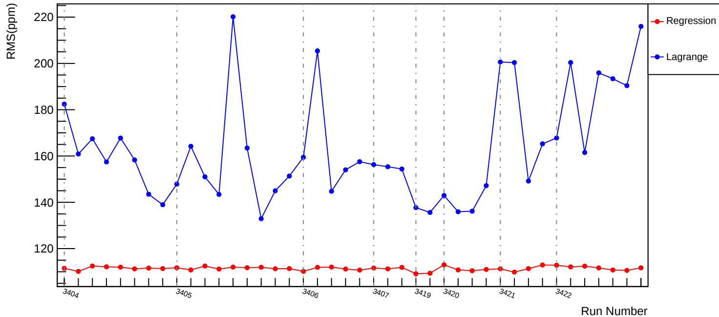
Slug4: Corrected RMS (ppm): asym_us_dd
