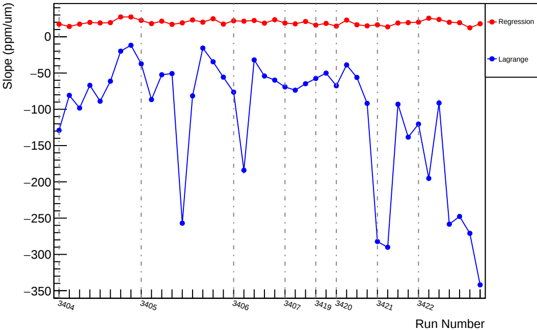
Slug4: Slope : us_dd_vs_evMon5 (ppm/um)
