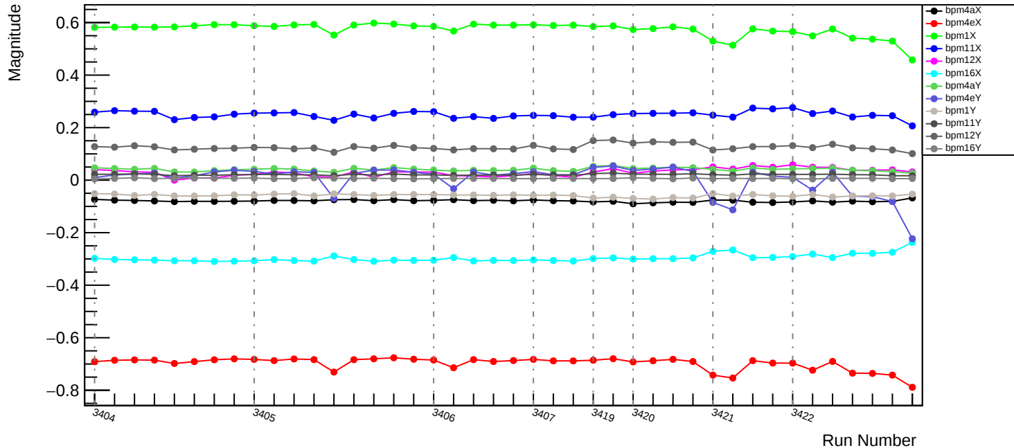
Slug4: EigenVector #0
