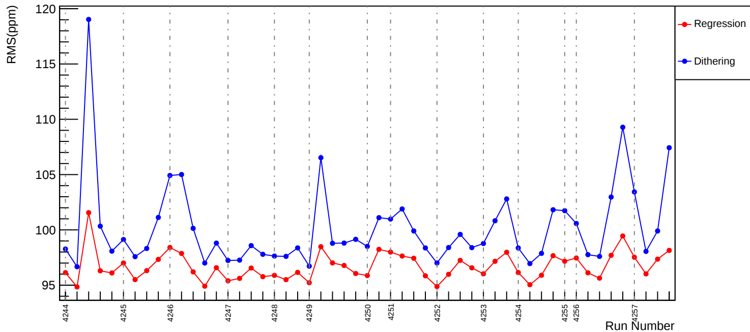
Slug50: Corrected RMS (ppm): asym_us_avg
