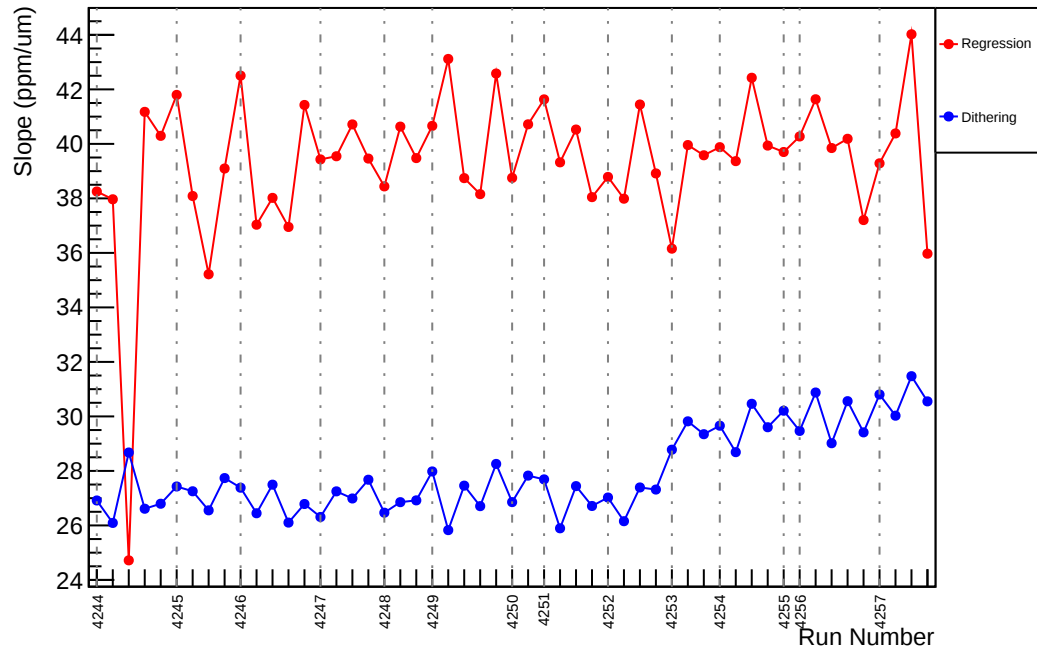
Slug50: Slope : usl_vs_evMon3 (ppm/um)
