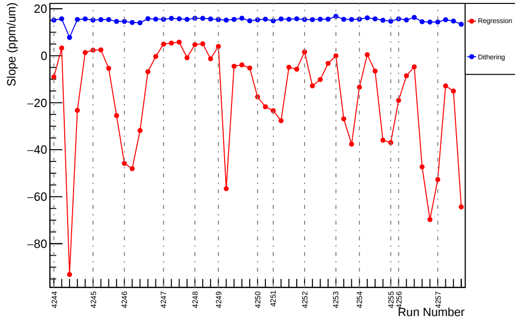
Slug50: Slope : usl_vs_evMon4 (ppm/um)
