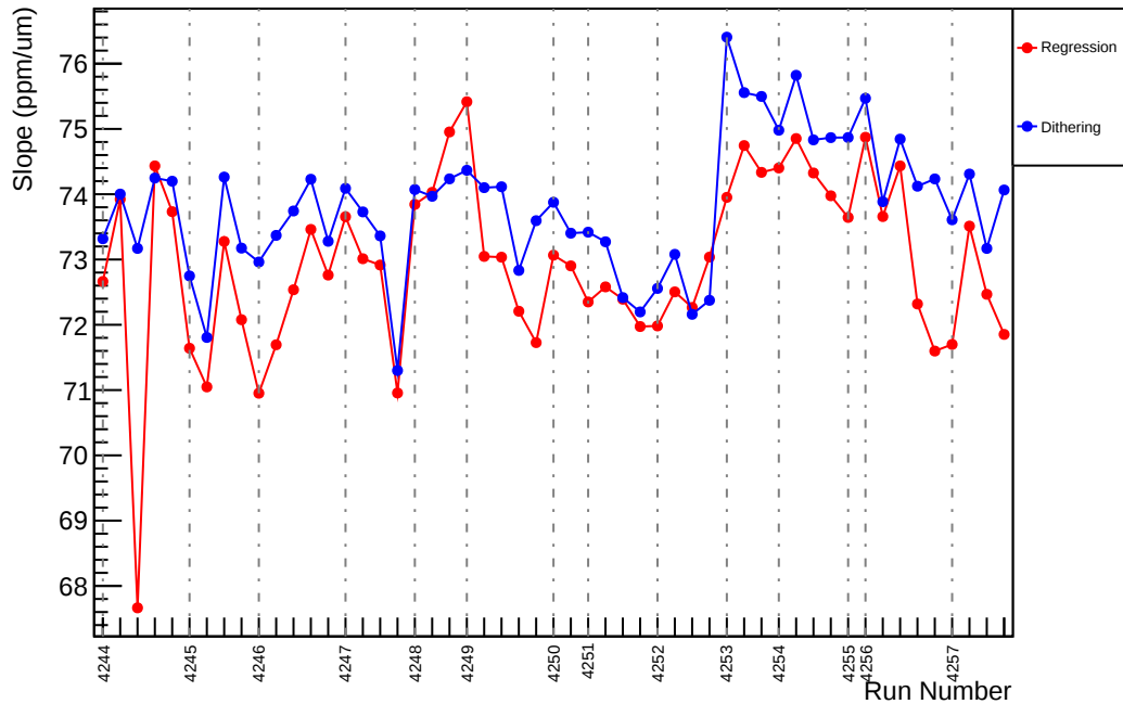
Slug50: Slope : usl_vs_evMon2 (ppm/um)
