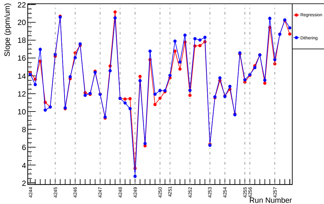
Slug50: Slope : usl_vs_evMon1 (ppm/um)
