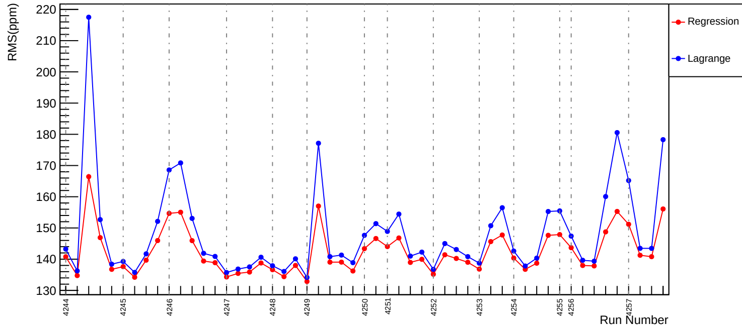
Slug50: Corrected RMS (ppm): asym_usl
