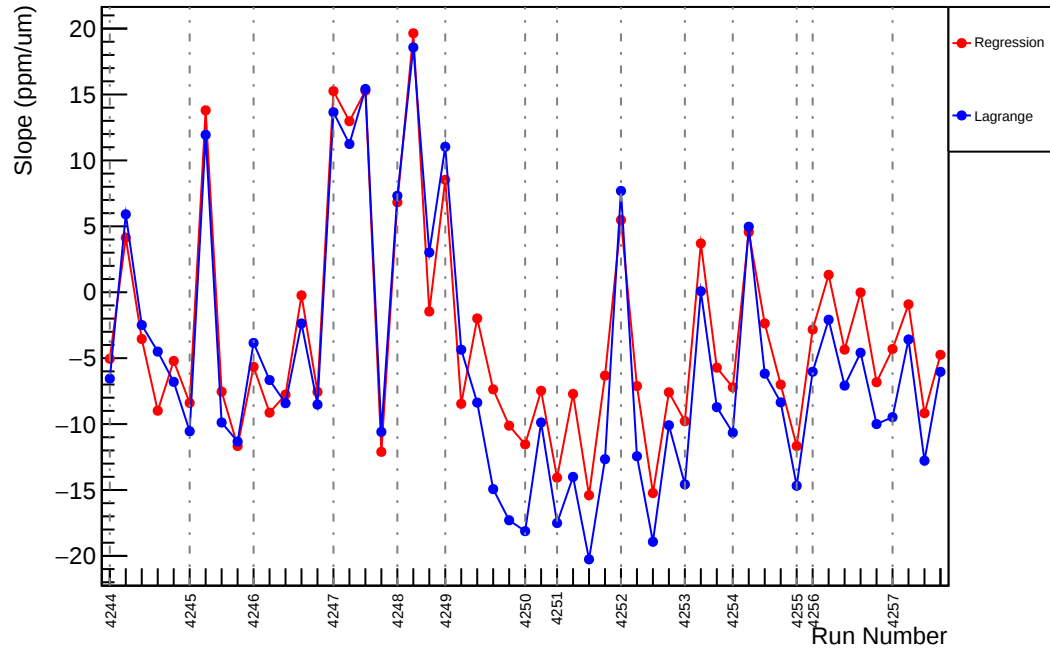
Slug50: Slope : usl_vs_evMon10 (ppm/um)
