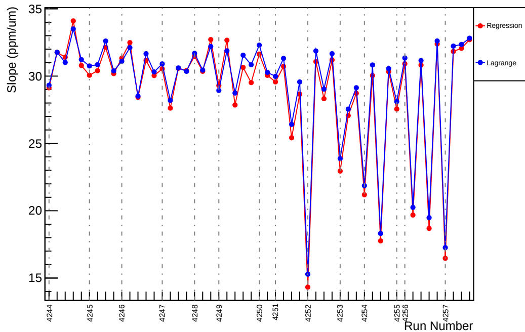
Slug50: Slope : usl_vs_evMon1 (ppm/um)
