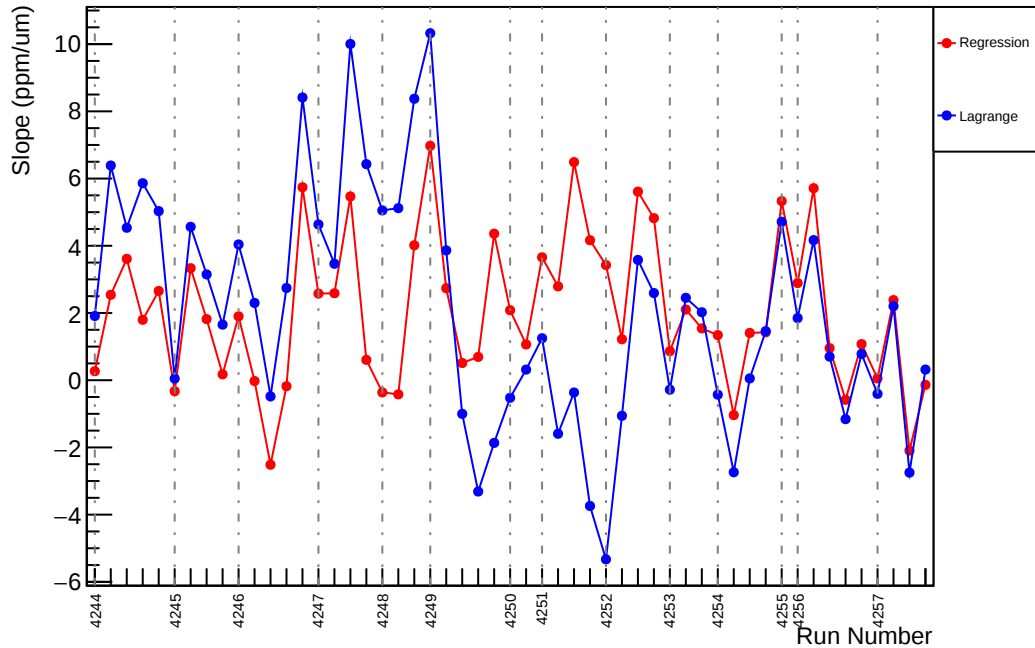
Slug50: Slope : usr_vs_evMon8 (ppm/um)
