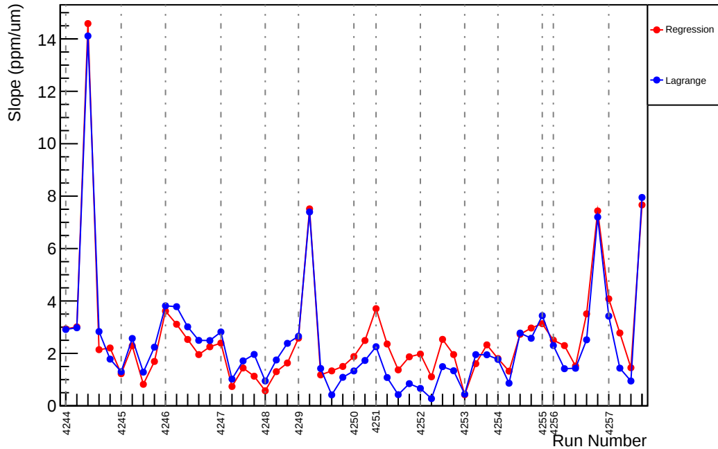
Slug50: Slope : usr_vs_evMon5 (ppm/um)
