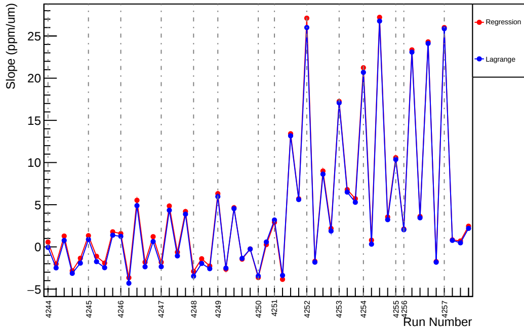
Slug50: Slope : usr_vs_evMon0 (ppm/um)
