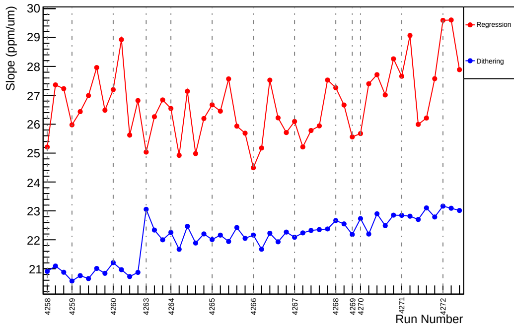
Slug51: Slope : us_dd_vs_evMon3 (ppm/um)
