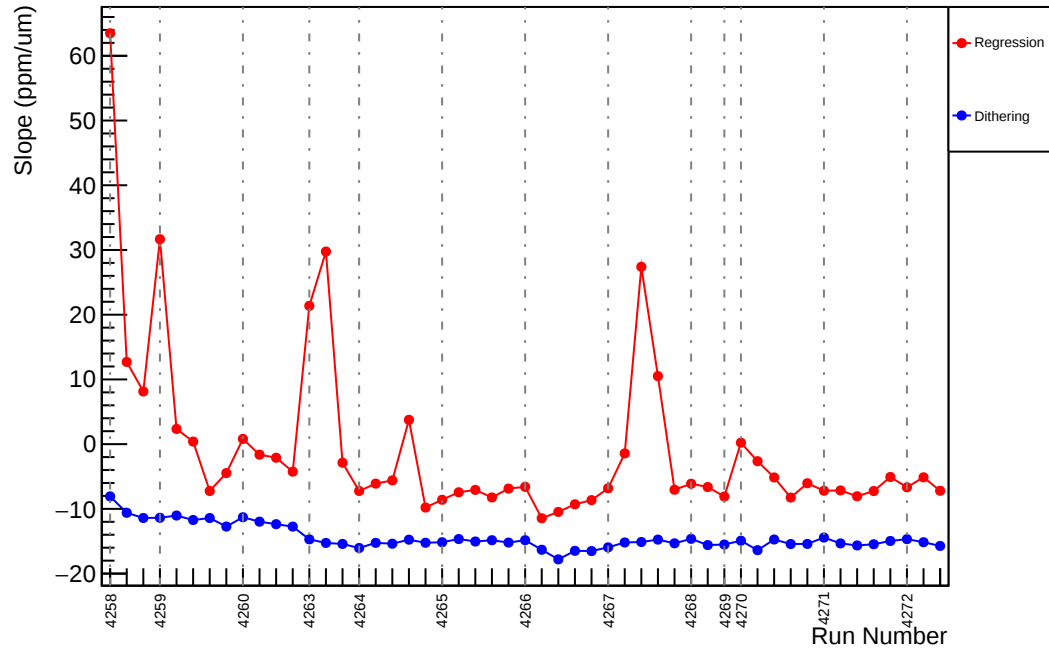
Slug51: Slope : usl_vs_evMon4 (ppm/um)
