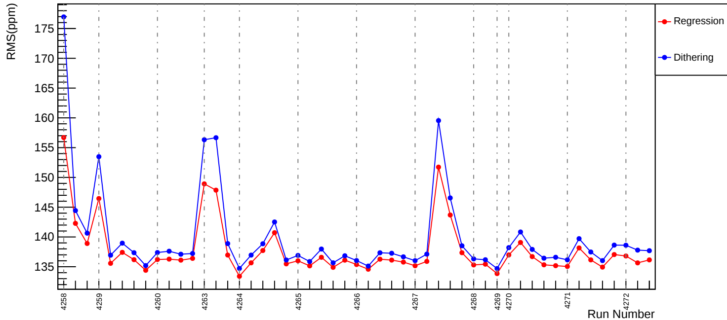
Slug51: Corrected RMS (ppm): asym_usl
