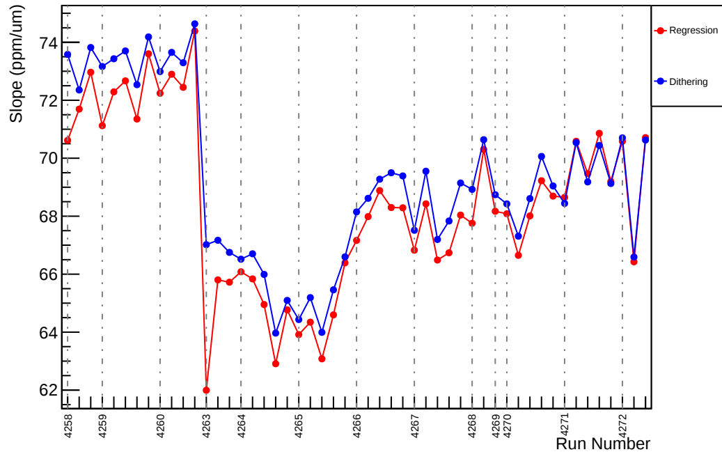
Slug51: Slope : usl_vs_evMon2 (ppm/um)
