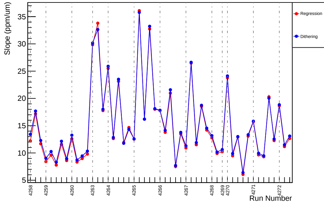
Slug51: Slope : usl_vs_evMon0 (ppm/um)
